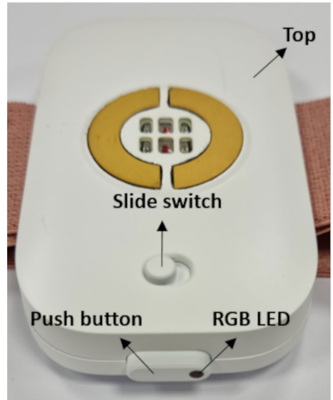
FIGURE 4. Slide switch, push button, and RGB LED. RGB = Red-Green-Blue.
