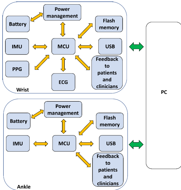
FIGURE 2. WESAA system architecture. ECG = Electrocardiogram, IMU = Inertial Measurement Unit, MCU = Microcontroller Unit, PC = Personal Computer, PPG = Photoplethysmograph.
