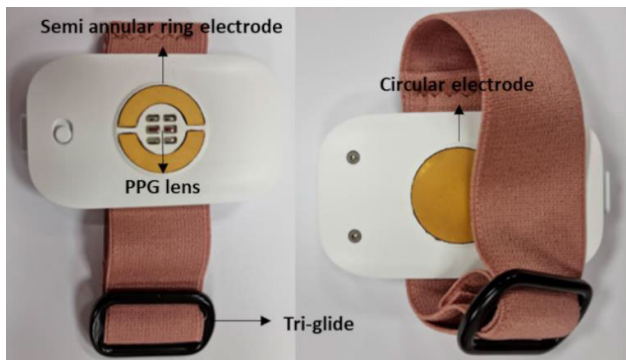
FIGURE 3. WESAA unit. PPG = Photoplethysmograph.
