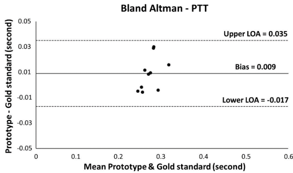
FIGURE 18. Bland Altman for PTT (Prototype & Gold standard). LOA = Limits Of Agreement, PTT = pulse transit time.
