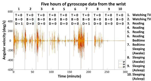
FIGURE 9. Five hours of gyroscope data from the most affected wrist. T = Tremor, B = Bradykinesia, D = Dyskinesia.
