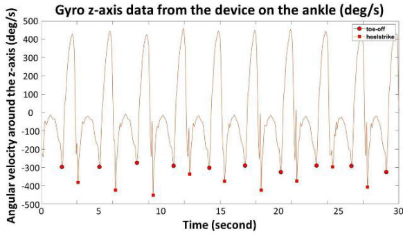
FIGURE 13. Angular velocity around the z-axis during walking. Gyro = Gyroscope.
