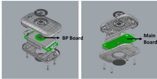
FIGURE 7. WESAA boards configuration (exploded view). BP = Blood Pressure.
