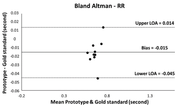
FIGURE 19. Bland Altman for RR (Prototype & Gold standard). LOA = Limits Of Agreement, RR = R-R interval.
