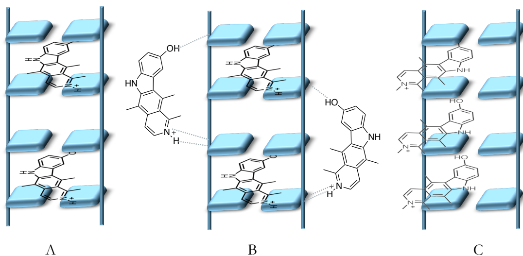
Figure 1.5: Binding modes of Ellipticine derivatives (adapted from Monnot et al. ) 21
