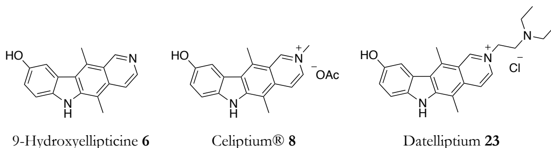
Figure 1.36: Ellipticine derivatives used in clinical trials
