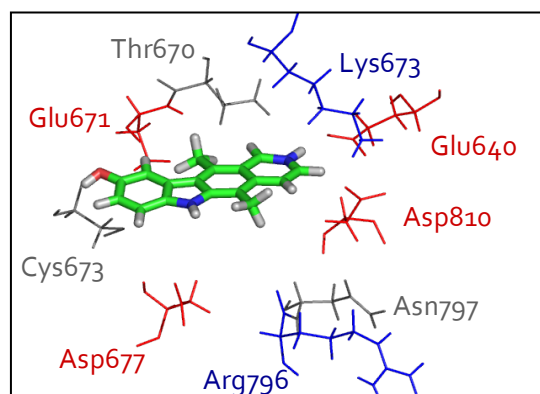
Figure 3.2: Proposed binding mode of protonated 9-Hydroxyellipticine 6 in the c-Kit kinase active site, determined from Molecular Dynamics simulations. 5
