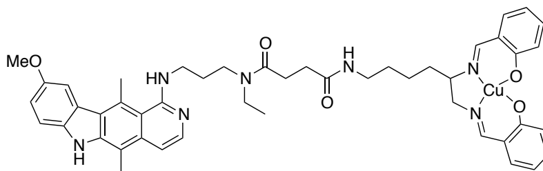
Figure 1.32: Ellipticine-Salen Copper hybrid 30
