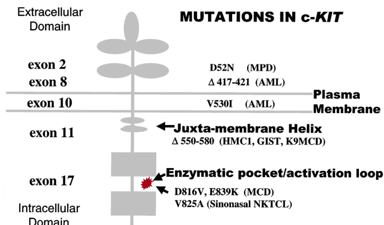
Figure 1.13: Mutations in c-Kit 2
