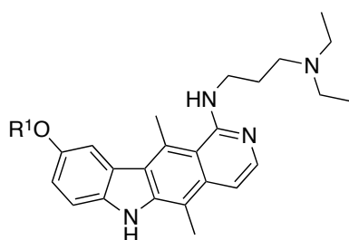
Figure 1.25 and Table 1.4: DNA binding constants and ID_{50} values for 1-[3-(diethylamino) propylamino]ellipticines 14c and 14f 99
