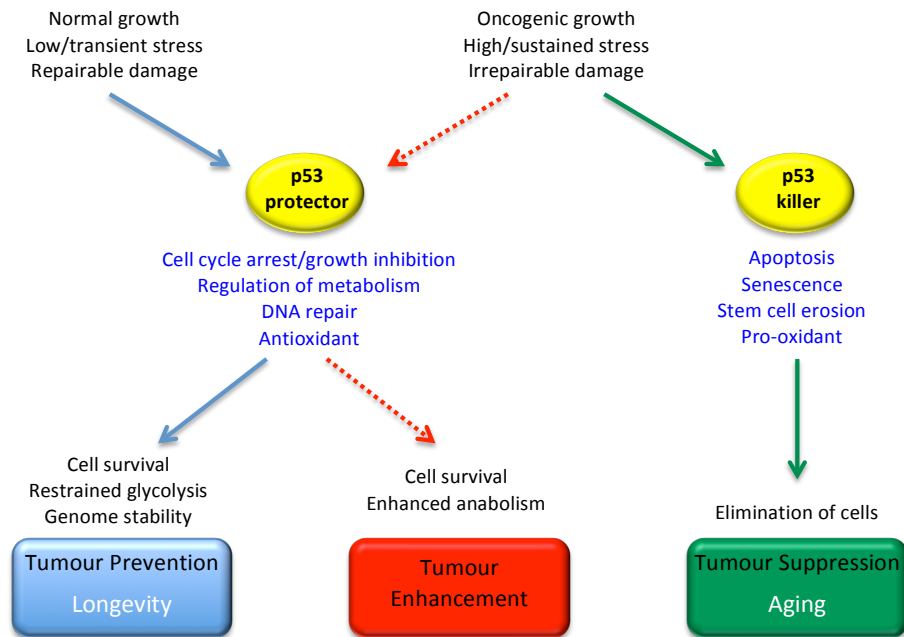
Figure 1.18: Dual mechanisms of p53 function (adapted from Vousden and Prives). 79
