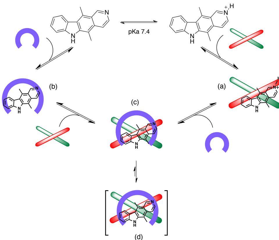
Figure 1.10: Model of ellipticine binding to DNA (G segment, red), topoisomerase II (purple arc) and the topoisomerase II-DNA complex (adapted from Froelich-Ammon, 1995). 43
