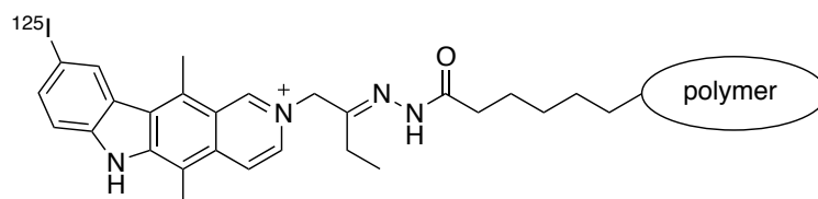
Figure 1.35: Polymer-conjugated Ellipticine Auger electron emitter
