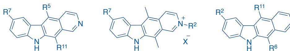
Figure 3.4: Isoellipticine and Deazaellipticine derivatives targeted for synthesis
