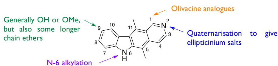
Figure 1.23: Ellipticine numbering system and main areas of derivatisation.
