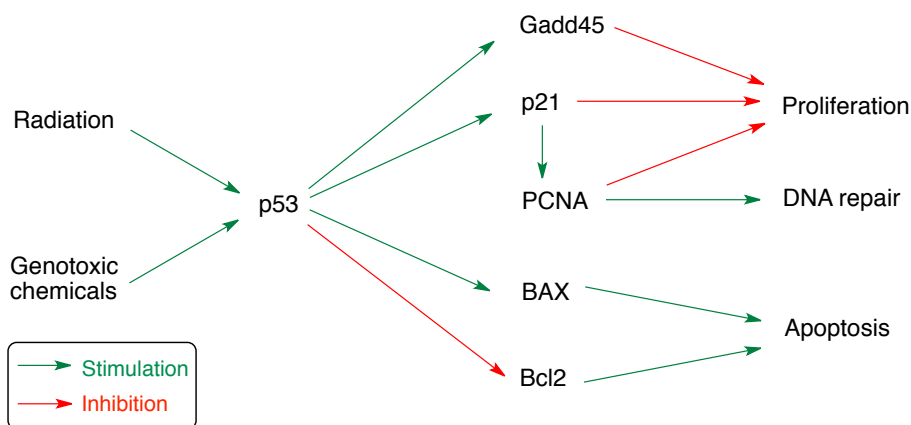
Figure 1.19: Response of p53 to DNA damage. 1
