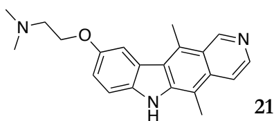
Figure 1.21: 9-( N,N -dimethyl ethanamine)-oxyellipticine derivative
