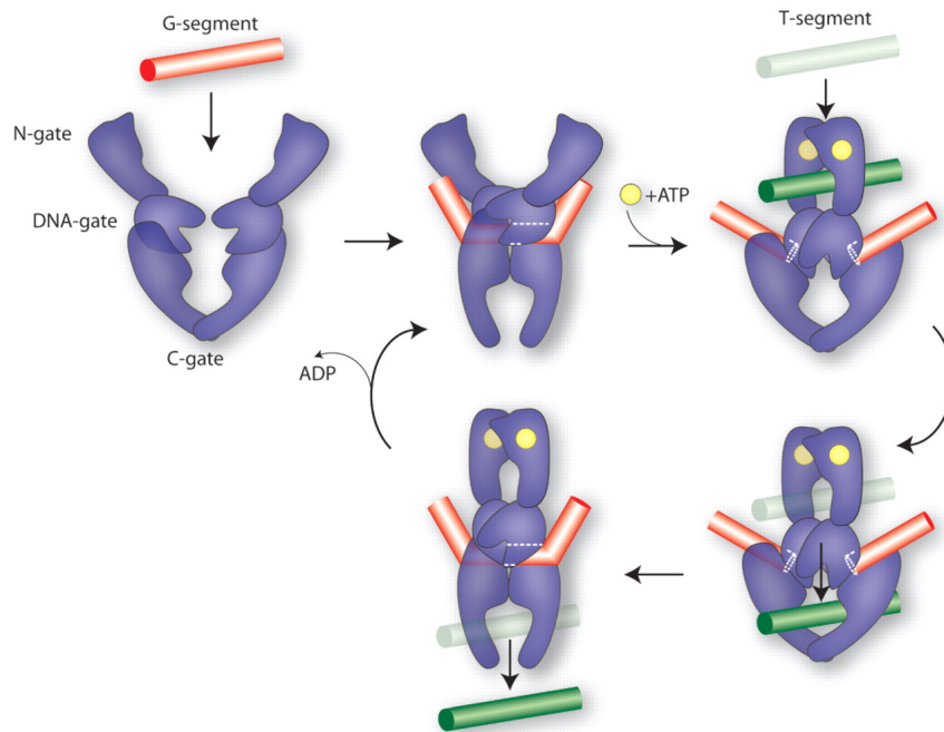
Figure 1.8: Catalytic cycle of topoisomerase II. 32 Topo II binds to a segment of DNA (G-segment, red bar), ATP (yellow circle) binds to the N-terminal domains, promoting the capture of a second DNA duplex, the T-segment (green bar) and dimerization of the ATPase domains (N-gate). Closure of the N-gate stimulates cleavage of G-segment DNA, coupled with opening of the DNA gate to allow passage of the T-segment through this double-stranded break. The G-segment is religated and the T-segment exits via the C-gate.
