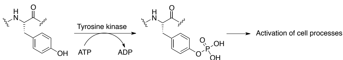
Figure 1.12: Phosphorylation by tyrosine kinases. 3
