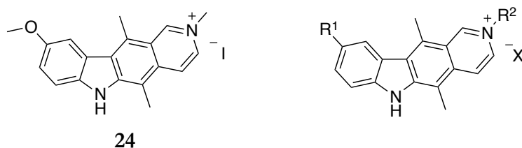
Figure 1.26: N -Methyl-9-methoxyellipticinium iodide 24 and general structure of ellipticinium salts.
