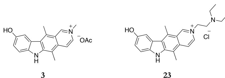
Figure 1.24: Celiptium 3 and Datelliptium 23
