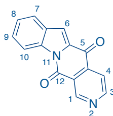
Figure 3.5: Indolo[1,2- b ][2,7]naphthyridine-5,12-dione 89
