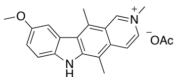
Figure 1.17: 9-Methoxy- N -methylellypticinium acetate 19
