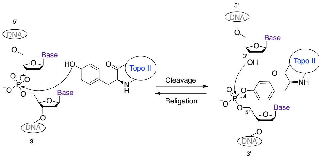
Scheme 1.1: Transesterification reactions involved in topoisomerase II activity. 3 (Reaction of one monomer shown)
