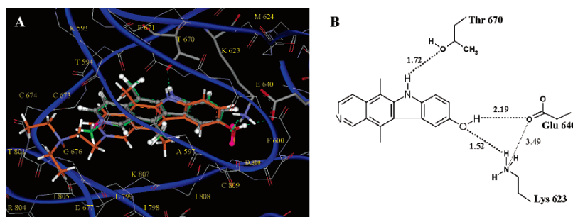
Figure 1.16: (A) Detail of the docked position of the most active compounds (9-hydroxyellipticine 6 is shown in gray, 9-hydroxy- N -methylellipticinium 3 in green, and N -alkylamino-9-hydroxyellipticinium 16 in orange). Conserved interactions are represented by dashed lines. (B) Map of the main interactions for 9-hydroxyellipticine 6 . 58
