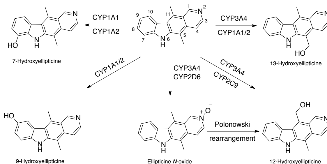
Scheme 1.4: Metabolism of ellipticine by human cytochrome P450 enzymes. 51
