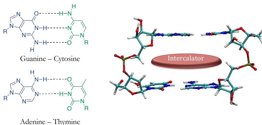
Figure 1.2: DNA base pairs (purines in blue and pyrimidines in green) and intercalation model
