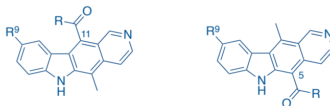
Figure 3.3: Ellipticine derivatives targeted for synthesis and biological evaluation
