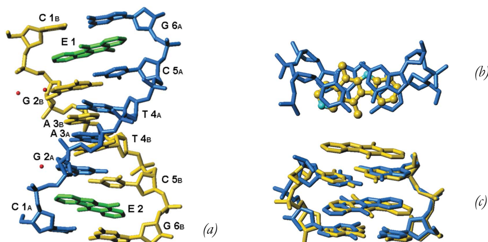
Figure 1.7: (a) The bis-intercalated d(CGATCG) 2 hexanucleotide. (b) Projection down the helix axis of a d(CpG)-d(GpC) dinucleotide with the sandwiched ligand. (c) Superimposition of the structure from Jain et al. (1979) in yellow and the equivalent part of Canals' structure in blue. 25
