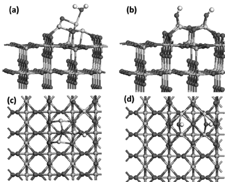
Figure 6: Relaxed atomic structures after water adsorption and relaxation at (a), (c) (CaO) 4 -modified rutile (110) and (b), (d) (BaO) 4 -modified rutile (110). Molecular adsorption of water relaxes to dissociative water adsorption. The colour coding is the same as Figure 5
