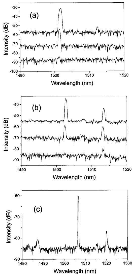
FIG. 2. Spectra from microring under (a) pulsed and (b) cw pumping. The estimated absorbed pump power in the pulse case is 31, 58, and 154 \mu\text{W} while in the cw regime it is 50, 85, and 115 \mu\text{W} . The resolution of the spectrometer is set to be 0.5 nm. The spectrum from a second disk is shown in (c) under cw pumping with power of 110 \mu\text{W} . Note the change in scale in (c).
