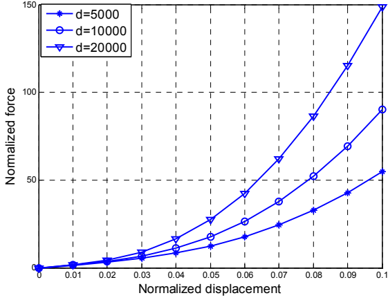
Figure 5 Normalized force against normalized displacement
