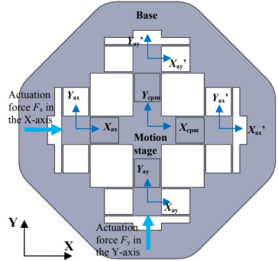
(a) XY CPM view I: Top view
