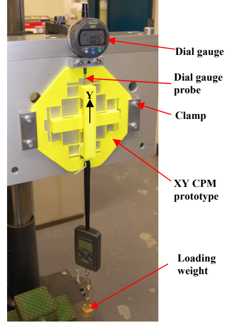
Figure 7 Single-axis loading testing rig
