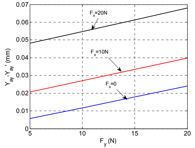
Fig. 11 Displacement difference on the input stage along the Y-axis
