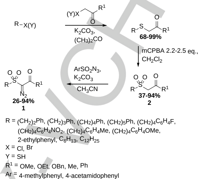
Scheme 1. Copper catalysed C–H insertion reactions of \alpha -diazo- \beta -oxo sulfones. [11]
