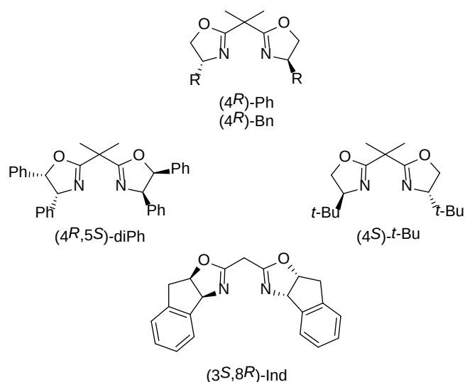
Figure 1. Commercially available bis(oxazoline) ligands.
