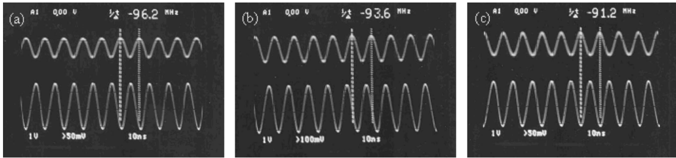
FIG. 9. Instrument provided rf phase shift produced with the NLC cell sample with no voltage applied and instrument wavelength tuned to (a) 1520 nm @ 96.2 MHz=2 X AOTF drive, (b) 1560 nm @ 93.6 MHz=2 X AOTF drive, and (c) 1600 nm @ 91.2 MHz=2 X AOTF drive. Top traces from instrument and bottom traces from phase-locked synthesizer.
