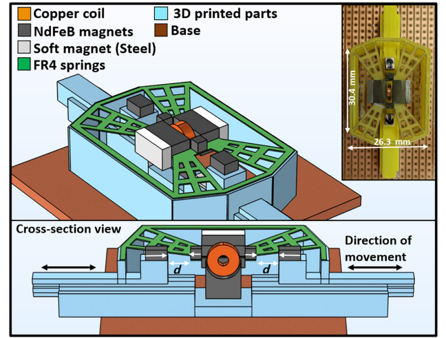
FIG. 1. Schematic view (top) and cross-section view (bottom) of the VEH. White arrows indicate the polarity of the magnets. The fabricated VEH prototype is shown at the inset.
