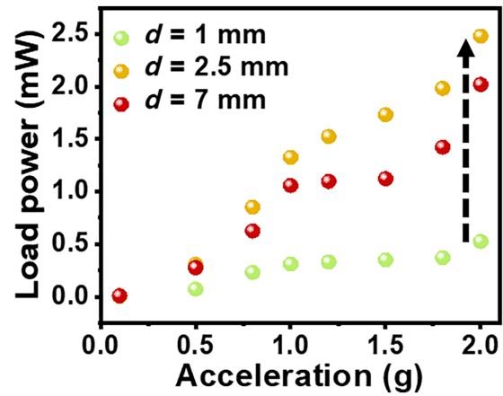
FIG. 11. The performance comparison of the VEH topologies in terms of the extracted power across a resistive load ( 2 \text{ k}\Omega ) for different values of interspacing between the repulsive magnets ( d = 1 \text{ mm} , 2.5 \text{ mm} , 7 \text{ mm} ).
