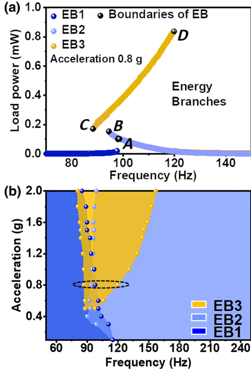
FIG. 4. (a) Shows the extent of the energy branches EB1, EB2, and EB3 for 0.8-g drive amplitude. The branch EB3 is achieved through the designed frequency routine. (b) Shows the mapping of energy branches EB1, EB2, and EB3 on the acceleration-frequency plane.
