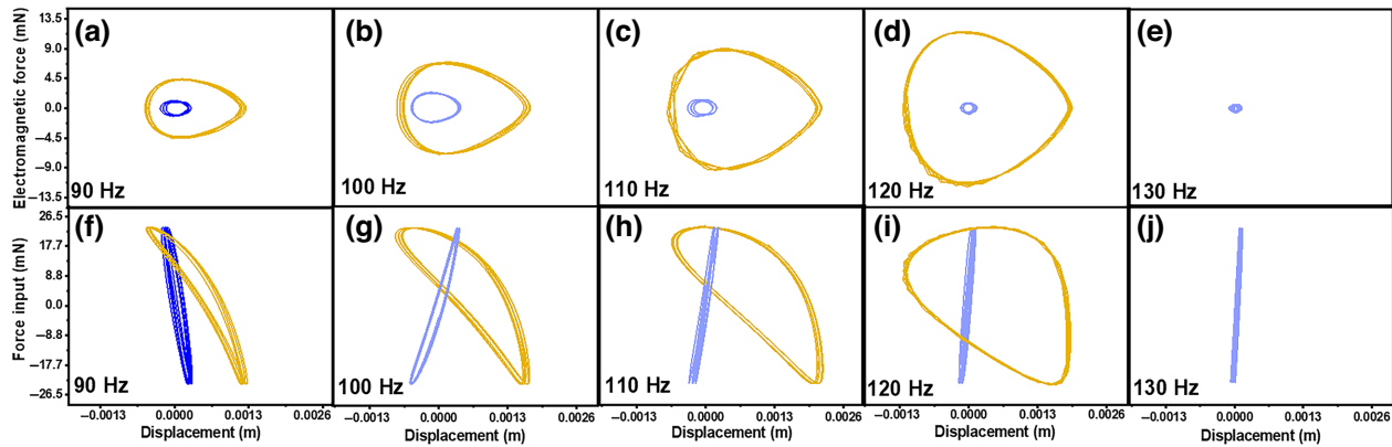
FIG. 9. With d = 2.5 mm, the eyes corresponding to electrical energy dissipating through involved damping are shown in (a)–(e). The eyes representing mechanical energy injection into the VEH are shown in (f)–(j). The colors of these eyes correspond to the different energy branches depicted in Figs. 2(a) and 3.
