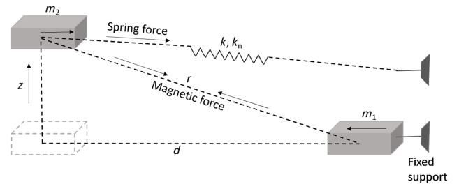
FIG. 5. Schematic of the magnetic interaction; for the sake of simplicity only the vertical displacement of m_2 is considered here.
