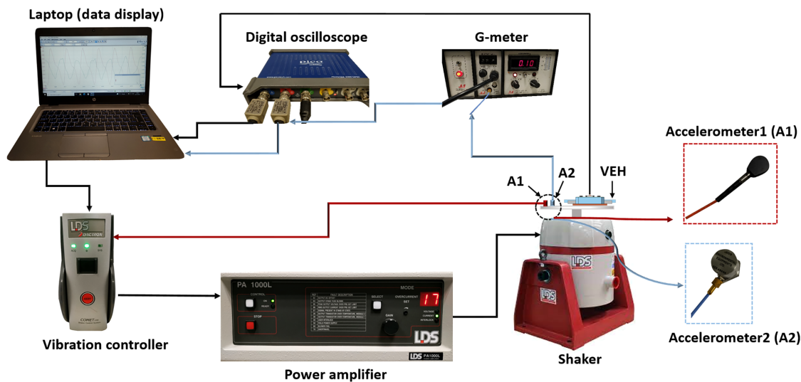
FIG. 2. Schematic view of the experimental setup for concurrent experimental measurement of the load voltage and the amplitude of excitation fed to the VEH to construct the eyes .
