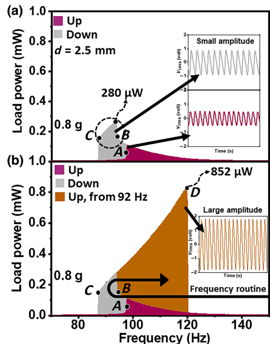
FIG. 3. Variation of load power with (a) conventional up and down sweep and (b) designed frequency sweep of the drive for 0.8-g excitation. The top and bottom inset of (a) are the time traces of the VEH's response on up and down sweep, respectively. The inset of (b) shows the time trace of the VEH's response corresponding to large power output.
