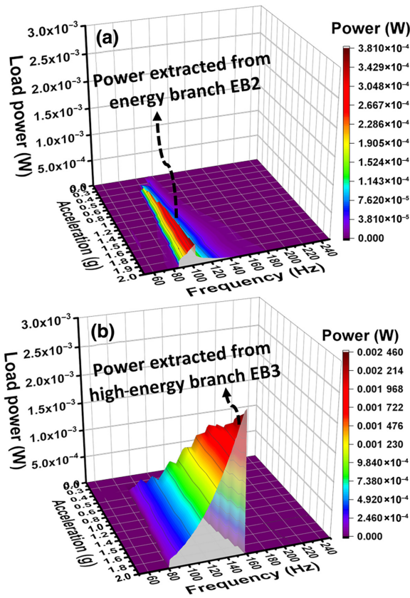
FIG. 10. Variation of the deliverable power of the VEH as a function of the frequency and amplitude of the drive for d = 2.5 mm, (a) with conventional up and down frequency sweep and (b) with specifically designed frequency routine.
