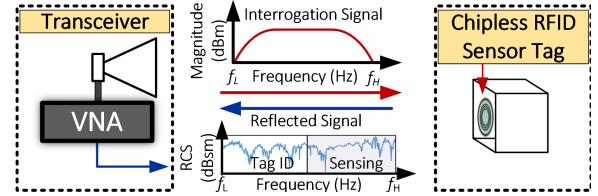
Fig. 1. Overview of a chipless RFID System.
