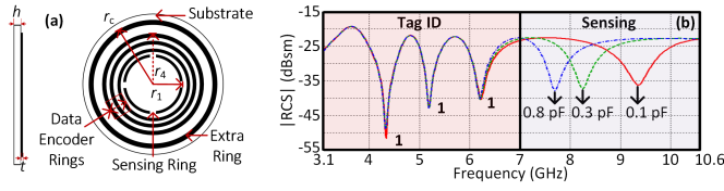
Fig. 2. A 3-bit CRFID sensor tag: (a) Topology ( r_c = 14 mm), (b) Simulated EM RCS response of tag ID 111 with 0.1, 0.3, and 0.8 pF sensing points.
