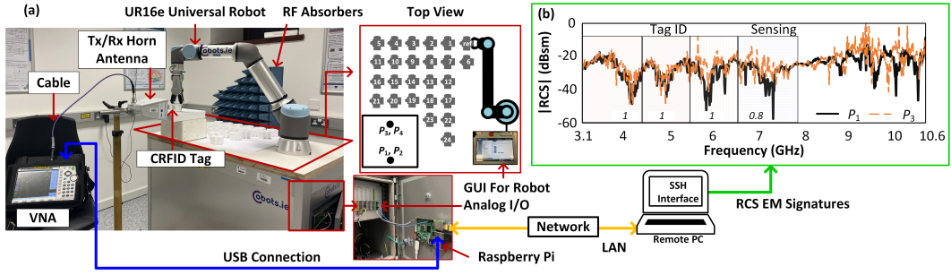
Fig. 4. (a) Automated RCS data collection setup using Ur16e Robot (b) Measured RCS of tag ID '111' with 0.8 pF sensing value at P_1 and P_3 .
