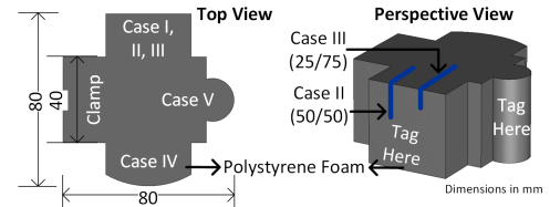
Fig. 3. Foam structure to mimic different shape surfaces.
