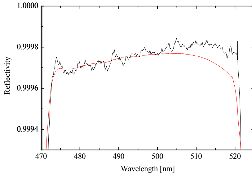
Figure 2.10 Comparison of the same mirror reflectivity calibrated by NO_2 (top black) and by Rayleigh scattering (red bottom)
