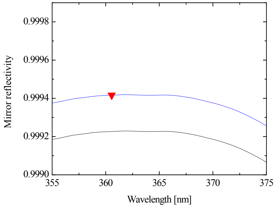
Figure 2.11 The mirror reflectivity calibrated by Rayleigh scattering (black line). The blue line shows the mirror reflectivity scaled to the value determined by the O 4 dimer absorption at 360.5 nm (red triangle)
