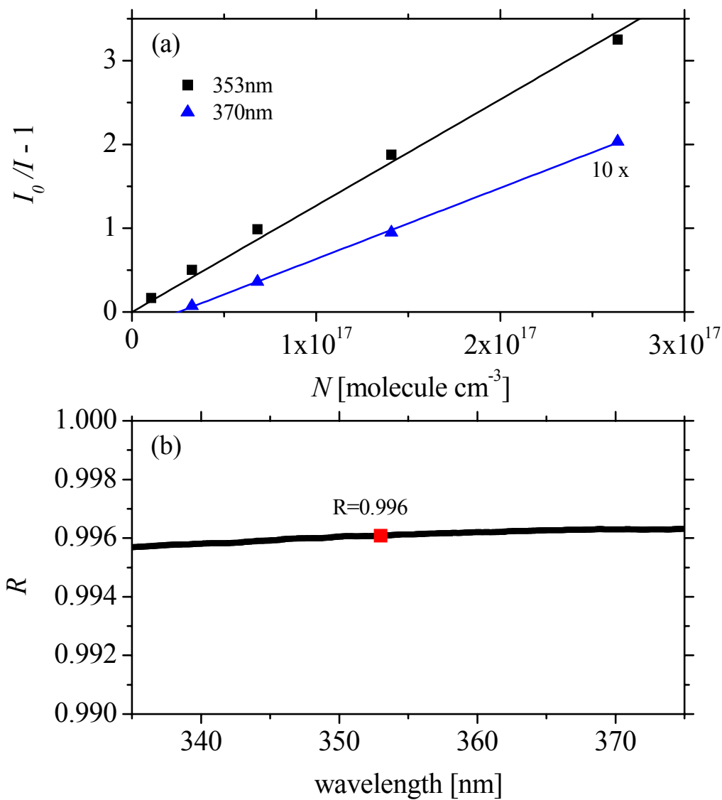
Figure 3.2 (a) Fractional absorption of \text{O}_3 at 353nm and 370 nm. The slope of the graph, \sigma_{\text{O}_3}d/(1 - R) , was used to determine R based on the literature absorption cross-section at 353 nm. (b) Mirror reflectivity scaled to give the literature cross-section of \text{O}_3 absorption at 353 nm.
