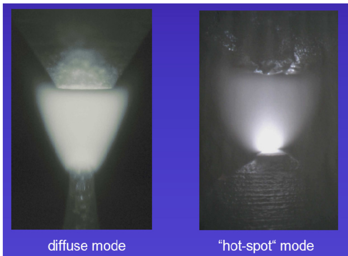
Figure 2.2 Hot Spot of the Arc Lamp. Comparison between the brightness of the normal Xe arc lamp (left) and that of the “hot-spot” mode lamp (right) showing the very bright spot near the cathode (Welz et al., 2006a)
