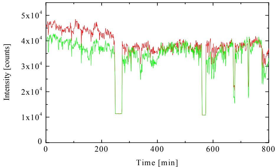
Figure 4.7 The cavity intensity measured at 370 nm (green) and 430 nm (red) on 20 Aug 2009. The intensity drops around 250 min and 550 min correspond to calibration of the system.
