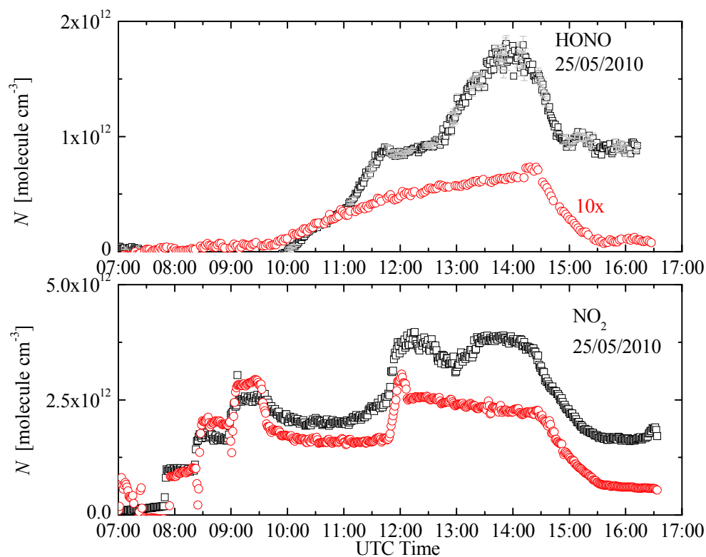
Figure 6.8 Results of IBBCEAS (black) and CEAM-DOAS and CL (red). Note that the DOAS HONO measurements are scaled 10 fold.
