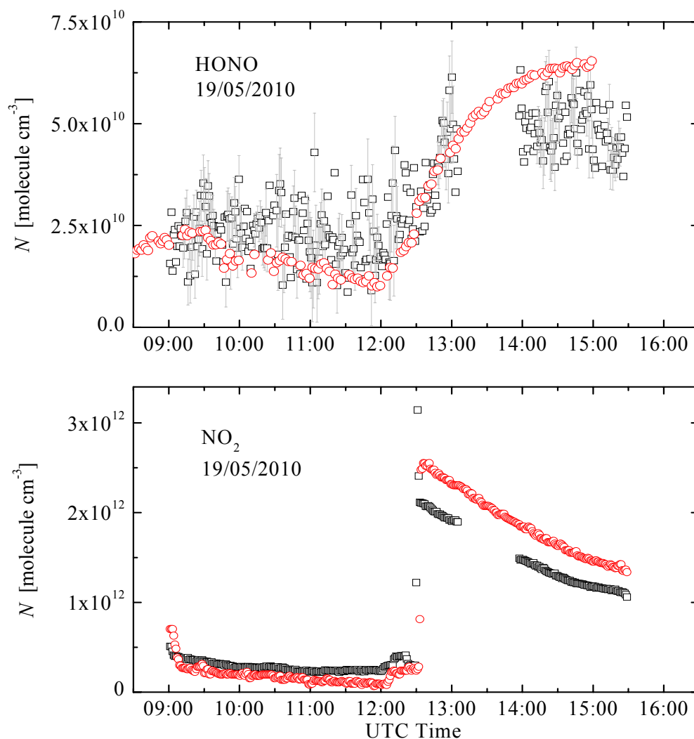
Figure 6.9 Results of IBBCEAS (black) and CEAM-DOAS and CL (red) measurements of HONO and NO 2 .
