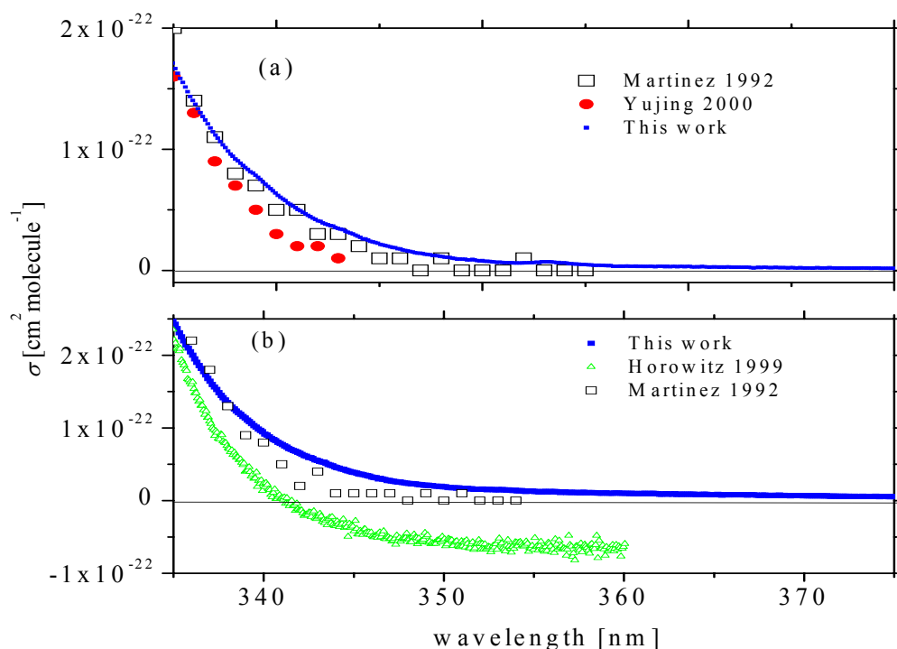
Figure 3.8 Absorption cross-sections of (a) 2-butanone and (b) 2-pentanone.
