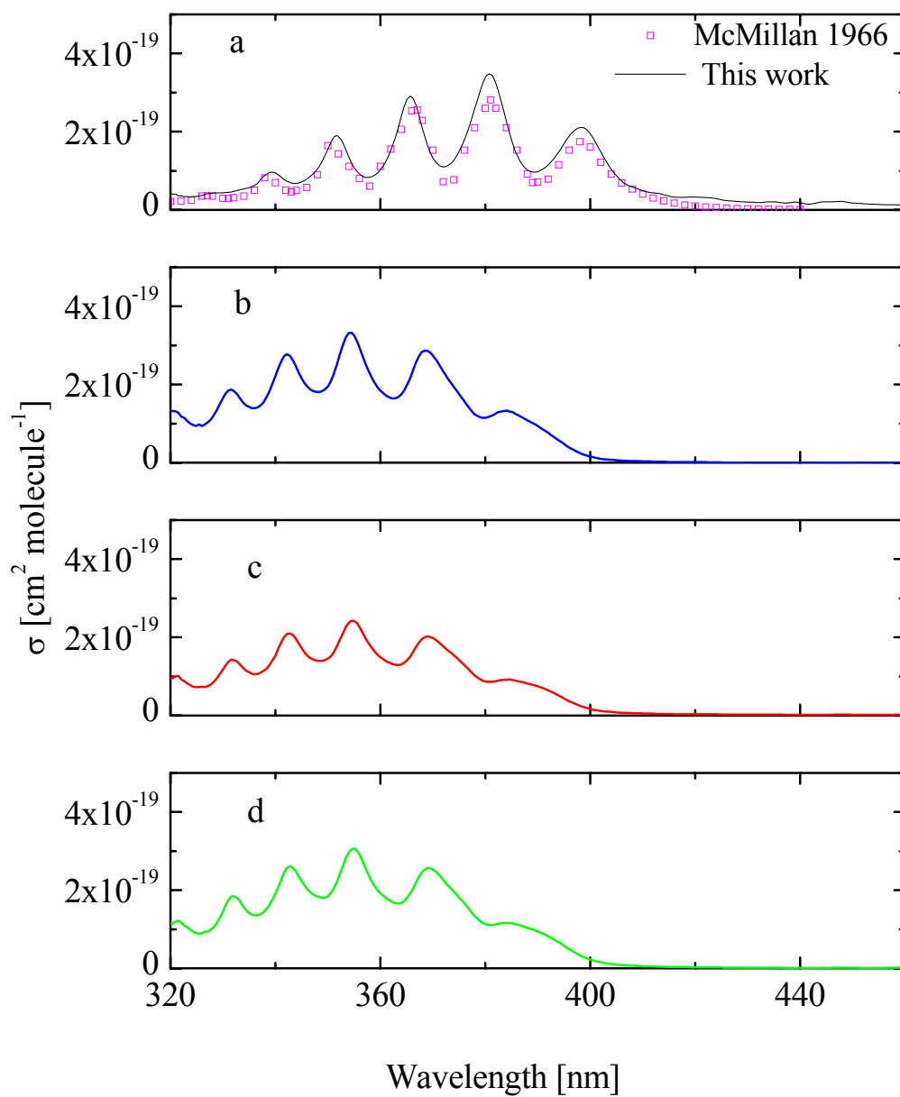
Figure 5.5 Absorption cross-sections of some alkyl nitrites from 320 to 460 nm (a) tert-butyl nitrite (this work in black line) with the McMillan 1966 spectrum (in pink squares) (b) iso-butyl nitrite (c) butyl nitrite (d) iso-pentyl nitrite.
