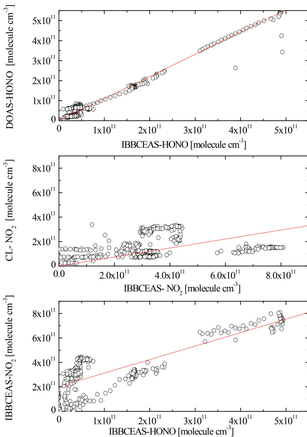
Figure 6.7 Top: HONO correlation between IBBCEAS and CEAM-DOAS and linear fitting (red) with slope = 1.1 and R^2 = 0.99 . Middle: the NO 2 correlation between IBBCEAS and CL detector and linear fitting (red) with slope = 0.36 and R^2 = 0.66 . Bottom: Correlation between IBBCEAS-HONO and IBBCEAS-NO 2 and linear fitting (red) with slope = 1.1 and R^2 = 0.68 .
