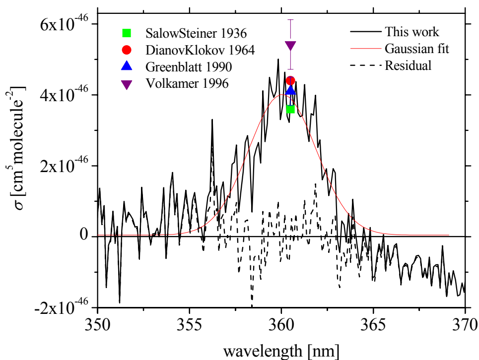
Figure 3.6 Experimental spectrum (black) and Gaussian fit (red) of the collision-induced absorption of the \text{O}_4 dimer. Literature maxima shown are those of Salow and Steiner (green square), Greenblatt (blue triangle), Dianov-Klokov (red circle), and Volkamer (purple triangle). Our measured spectrum was shifted downwards by the Gaussian offset of 1.1 \times 10^{-46} \text{ cm}^5 \text{ molecule}^{-2} to facilitate comparison with the literature maxima.
