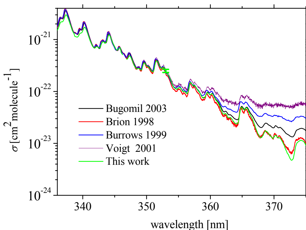
Figure 3.5 O 3 absorption cross-sections from this work, Voigt et al. (2001), Burrows et al. (1999), Bogumil et al. (2003), and Brion et al. (1998).
