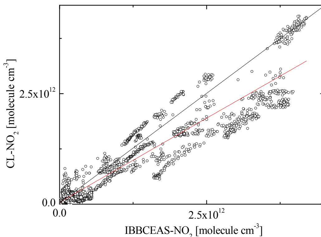
Figure 6.17 Overall comparisons of the IBBCEAS \text{NO}_2 measurements with those of the chemiluminescence detector. The linear fitting (red) has a slope=0.76 intercept: 4.36 \times 10^{10} and R^2=0.86 . The 1:1 ratio line is shown in black.
