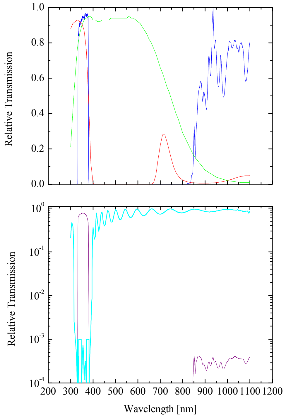
Figure 2.4 TOP: Filter transmission curves of Semrock 357 (blue), UG11 (red) and KG1 (green). BOTTOM: Calculated filter transmission curve of all three filters (purple) as well as the transmission curve of the optical cavity (cyan).
