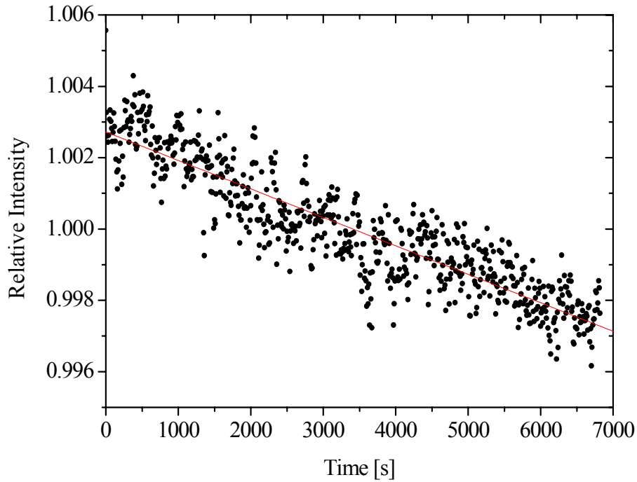
Figure 2.3 Temporal dependence of the intensity of the arc lamp output at 355 nm. The long term trend is given by a slope of 0.27% per hour and the short term fluctuations from the trend line are approximately 0.2%. The measurement plot of pixel at 355 nm was based on a 1 s integration time over 6820 s.
