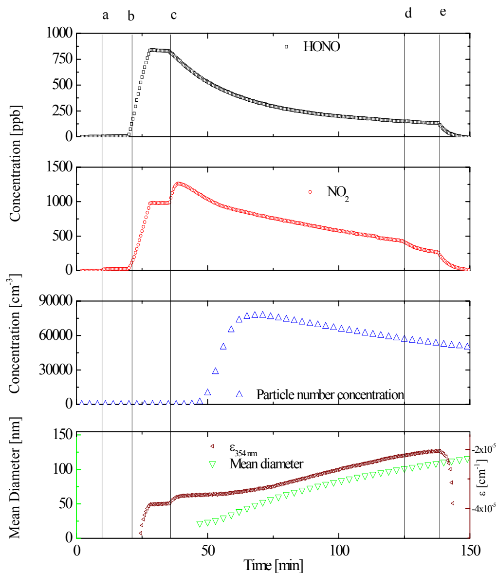
Figure 5.9 Temporal dependence of the concentrations of HONO, NO 2 , and total particle number concentration as well as the mean aerosol aerodynamic diameter and the aerosol extinction at 354 nm. Points (a) – (d) indicate changes in either the input concentrations or photolysis rate: (a) Addition of isoprene, (b) Introduction of HONO/NO/NO 2 , (c) Lamps switched on d) Lamps switched off, e) Flushing of chamber started.
