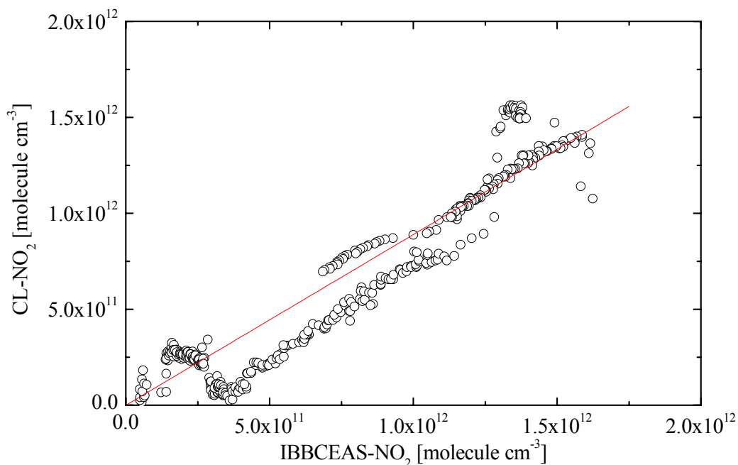
Figure 6.12 The \text{NO}_2 correlation between IBBCEAS and CL detector and linear fitting (red) with slope= 0.89 and R^2=0.95 .
