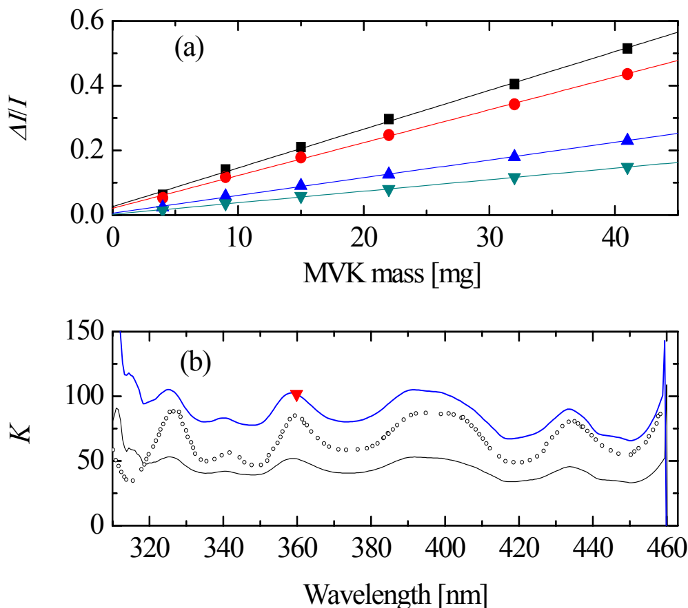
Figure 5.3 Calibration of the IBBCEAS simulation chamber instrument (a) Fractional absorption of MVK at 340 nm (black squares), 350 nm (red dots), 360 nm (blue triangles) and 370 nm (cyan triangles); linear regressions are also shown ( R^2_{340\text{nm}} = 0.9976 , R^2_{350\text{nm}} = 0.9982 , R^2_{360\text{nm}} = 0.9988 , R^2_{370\text{nm}} = 0.9989 ; y-intercepts are 0.026 at 340 nm, 0.020 at 350 nm, 0.006 at 360 nm and 0.003 at 370 nm). (b) The relative calibration from 320 to 450 nm using \text{NO}_2 (black line), and the absolute calibration at 360 nm after scaling to the reflectivity obtained from MVK (red triangle). The final scaled calibration is shown (blue line) along with the scaled transmission from the manufacturer's data (black dots).
