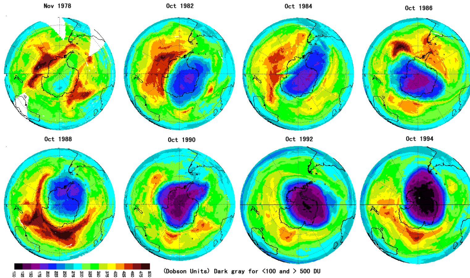
Figure 1.4 Evolution of the total ozone column abundance over the South Pole from 1978 to 1994, measured by the Solar Backscatter Ultraviolet and the Total Ozone Mapping Spectrometer (image courtesy of the NASA/Goddard Space Flight Centre).
