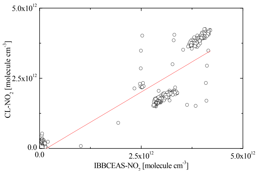
Figure 6.15 The \text{NO}_2 correlation between IBBCEAS and CL detector and linear fitting (red) with slope= 0.86 and R^2=0.77
