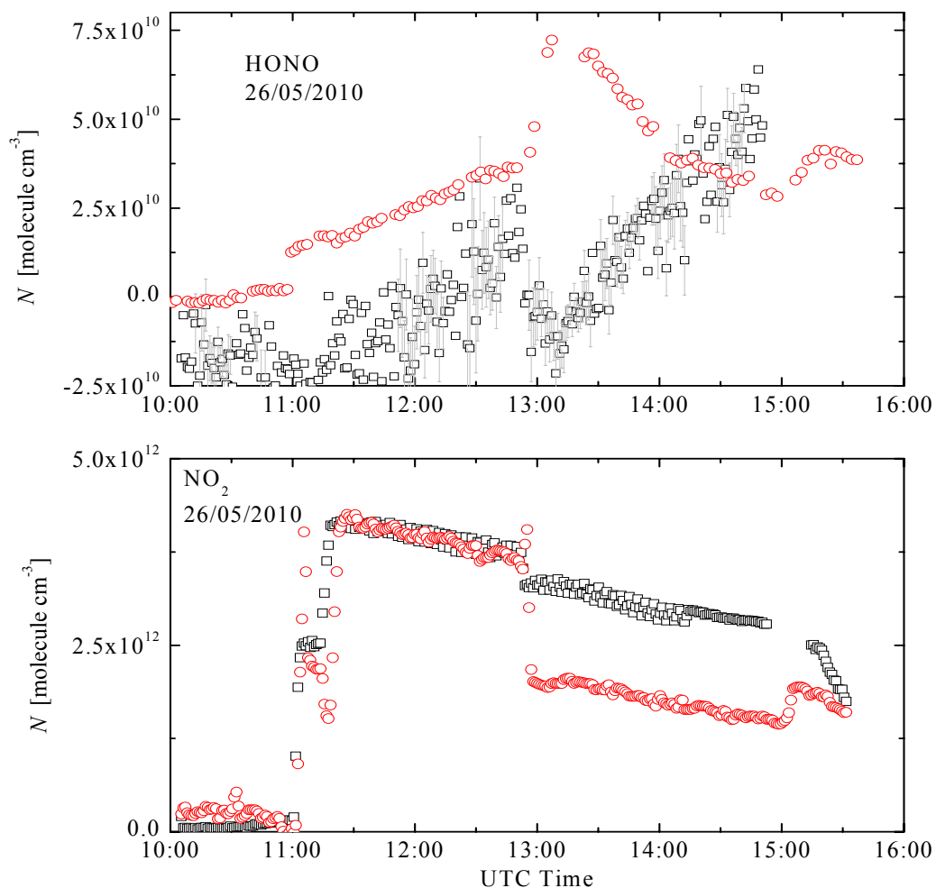
Figure 6.14 Results of IBBCEAS (black) and CEAM-DOAS and CL (red) measurements of HONO and NO 2 .
