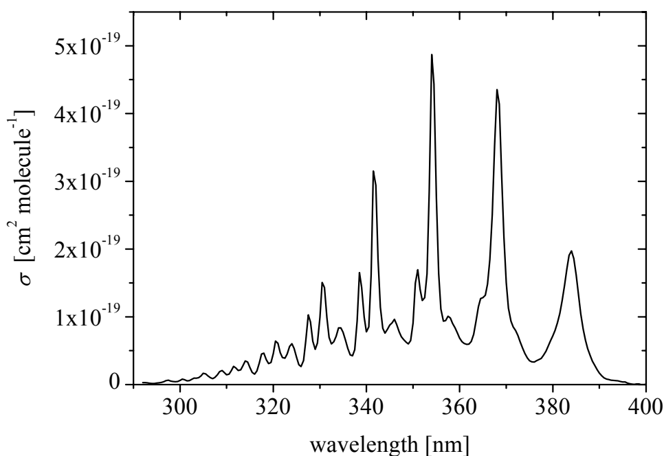
Figure 1.5 Nitrous acid absorption cross-section in the near-UV of \text{A}^1\text{A}' \leftarrow \text{X}^1\text{A}'' (Stutz et al., 2000).
