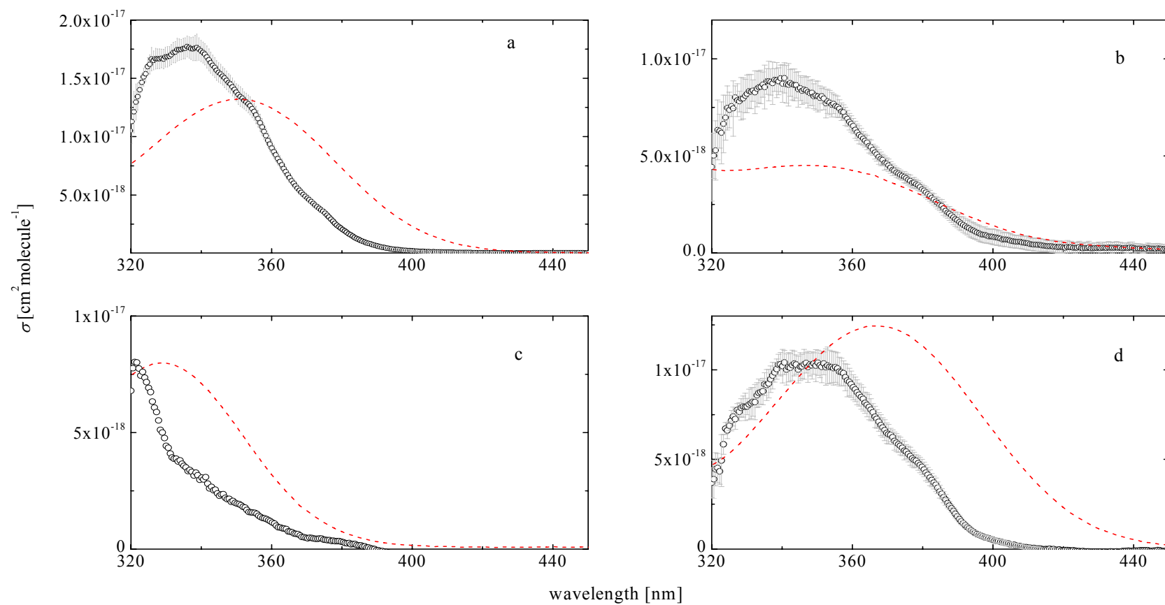
Figure 5.8 Nitrophenol absorption cross-sections in the gas phase (black cycle) with standard deviation (gray) and in acetonitrile solution (red dashes): a) 2-nitrophenol b) 3-methyl-2-nitrophenol c) 3-nitrophenol (arbitrarily scaled for the gas phase absorption) d) 4-methyl-2-nitrophenol.
