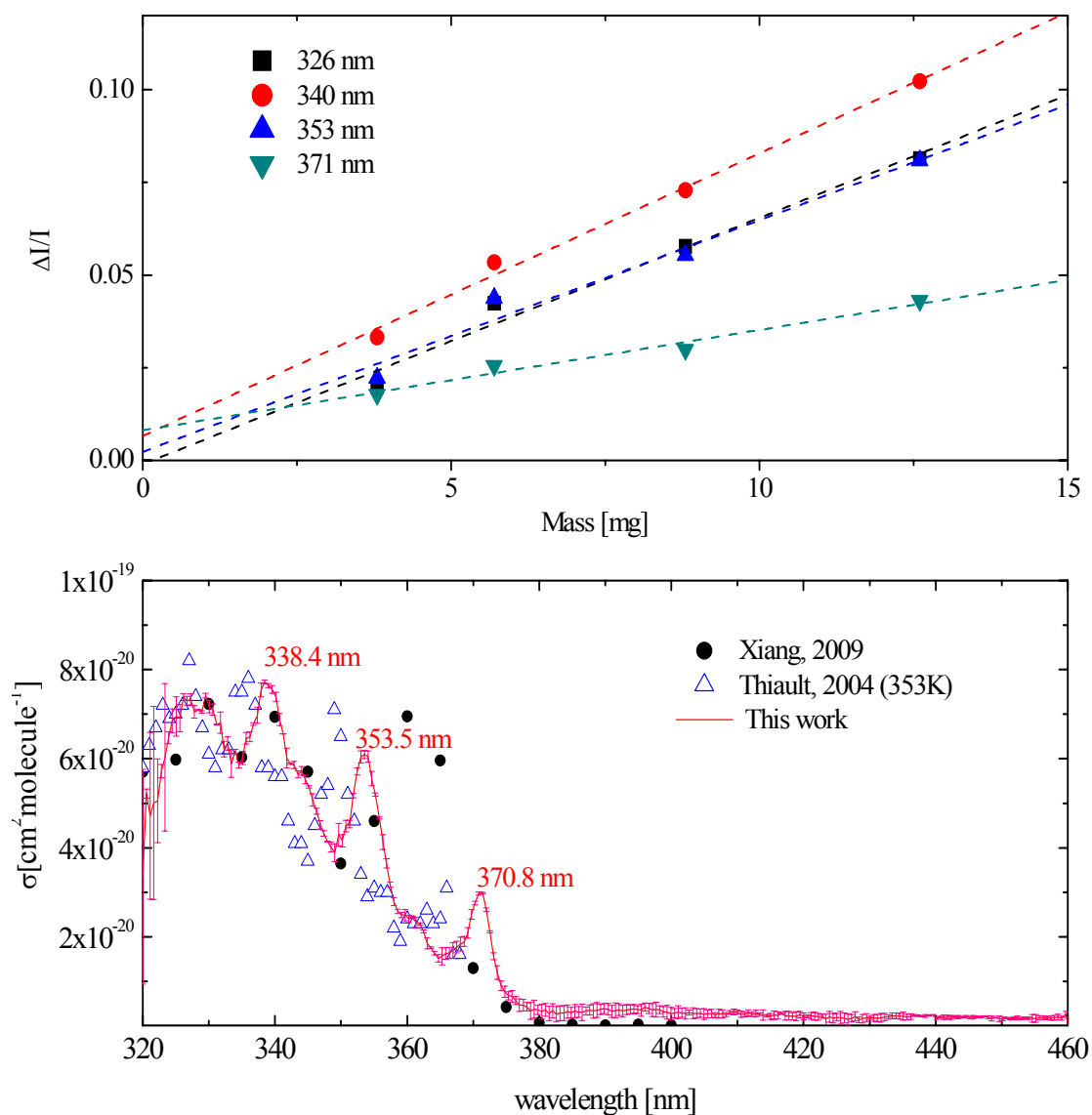
Figure 5.4 Top: Changes in the fractional absorption with increasing mass of benzaldehyde. Bottom: The benzaldehyde absorption cross-section and associated variation between different additions (error bars). Literature spectra covering the near-UV are also shown.
