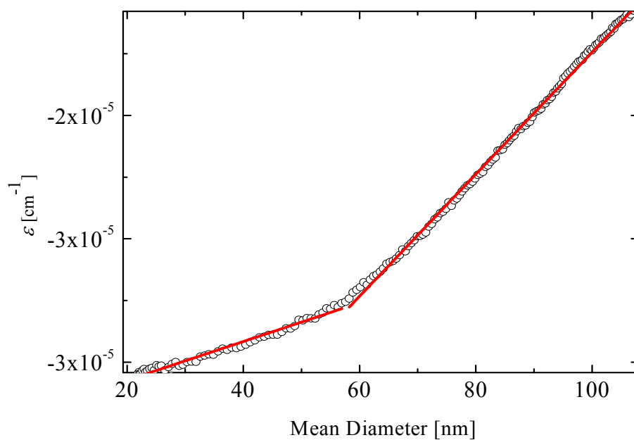
Figure 5.11 Correlation between the aerosol extinction at 354 nm and the mean diameter of the particles ( R^2 = 0.97 < 50 \text{ nm} and R^2 = 0.979 > 50 \text{ nm} ).
