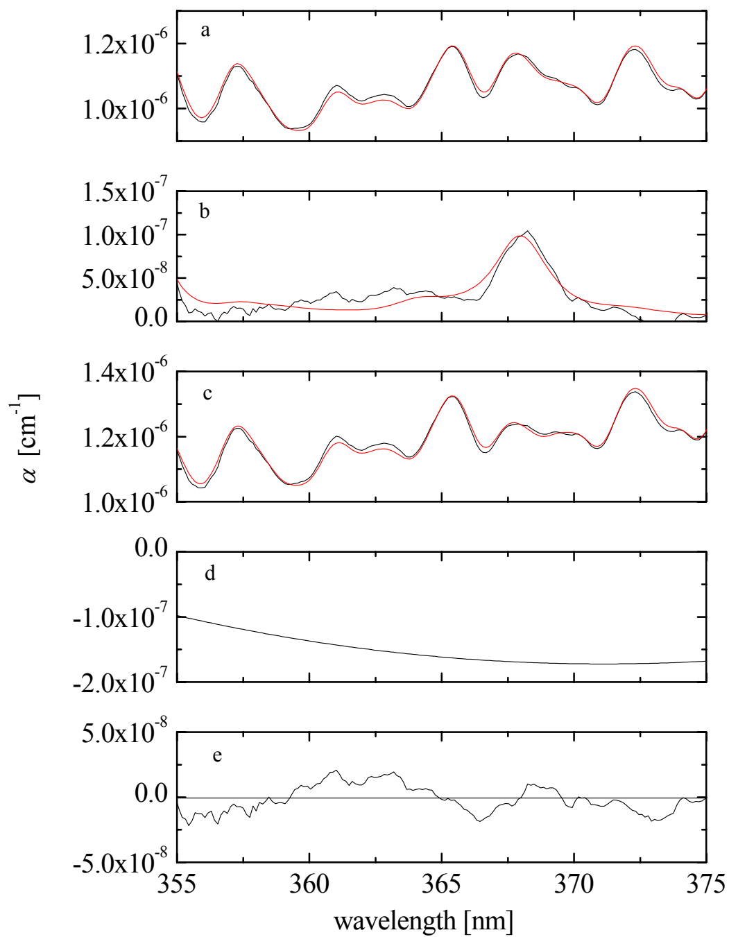
Figure 6.5 Experimental spectrum of HONO and NO 2 (black) as well as the fit result (red) The contribution of (b) HONO, (c) NO 2 , and (d) the polynomial base line are shown, as is the fitting residual in (e).
