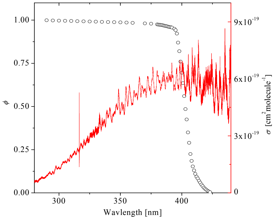
Figure 1.2 The recommended wavelength-dependent quantum yield of photolysis of NO_2 (black cycle) (DeMore et al., 1997) and absorption cross-section of NO_2 (red line) (Voigt et al., 2002)
