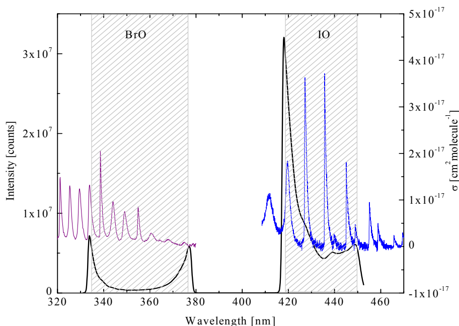
Figure 4.6 The dual cavity intensity (black) from 320 to 460 nm after 60 s acquisition time.
