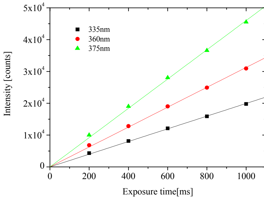
Figure 2.5 Linearity of the detector response to different integration times for several wavelengths.
