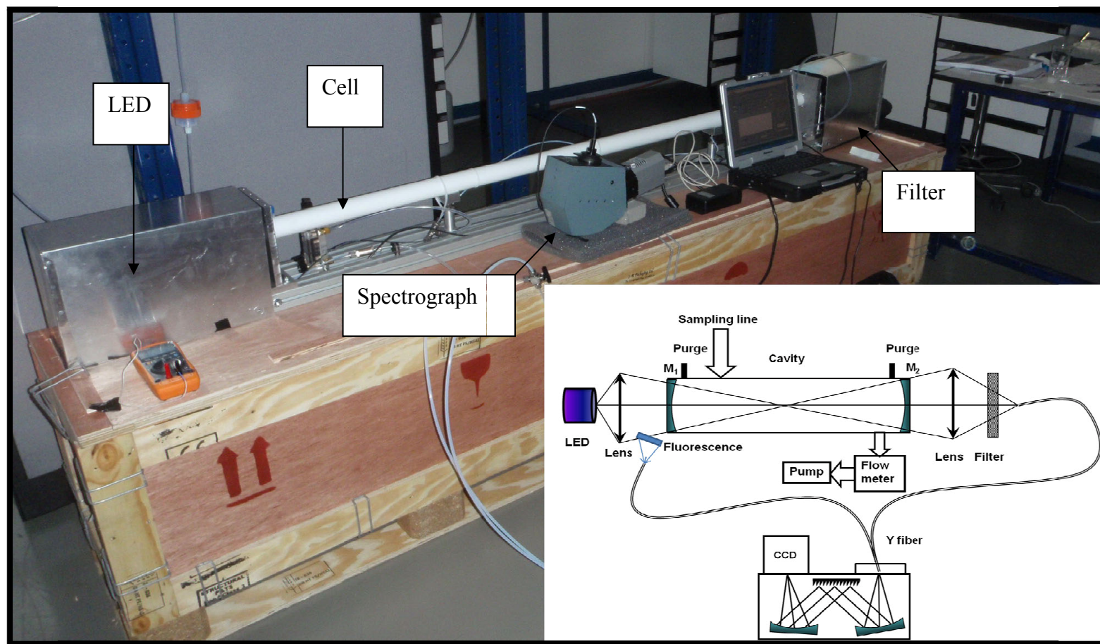
Figure 6.1 A photograph of the extractive IBBCEAS instrument during experiments in the EUPHORE Chamber. The inset shows a schema of the experimental system
