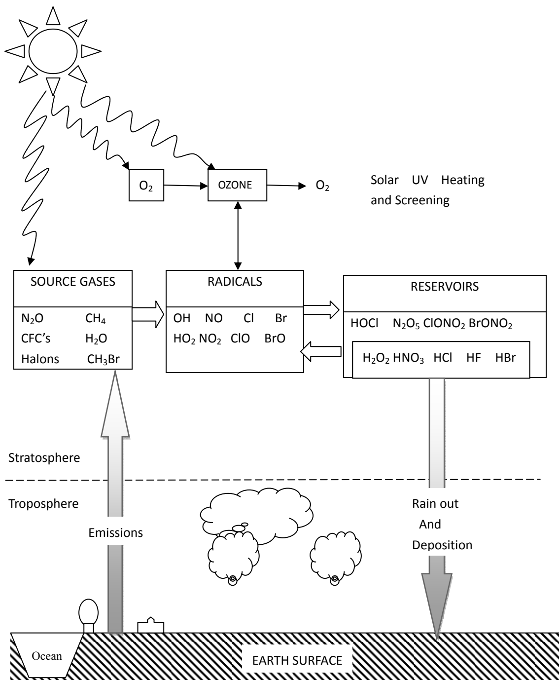
Figure 1.1 Schematic diagram of the chemistry of O_3 in the stratosphere..After Brasseur et al. 1999
