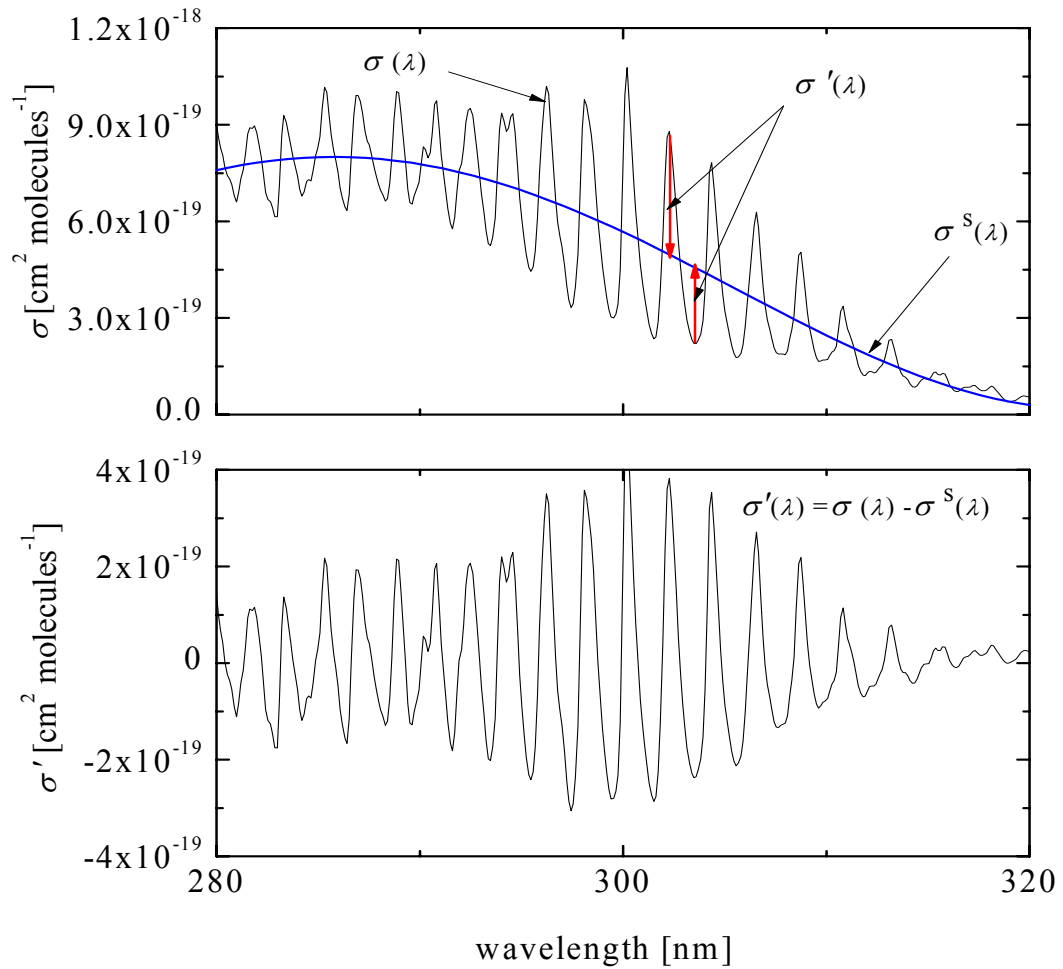
Figure 2.12 TOP: The absorption cross-section, \sigma(\lambda) , composed of a broadband (slow) component, \sigma^s(\lambda) , and a differential (fast) component, \sigma'(\lambda) , in the case of \text{SO}_2 (Bogumil et al.,
