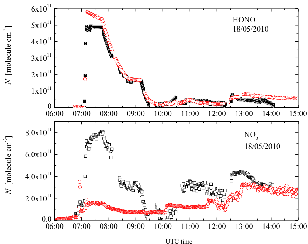
Figure 6.6 Results of IBBCEAS (black) and CEAM-DOAS and CL (red) measurements of HONO and NO 2
