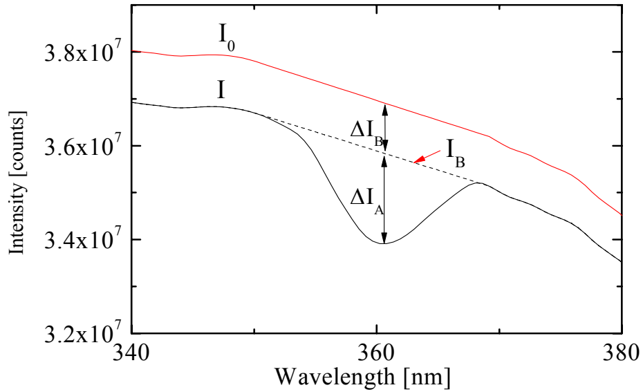
Figure 2.13 Calculation of the aerosol extinction based on a known structured absorption feature.
