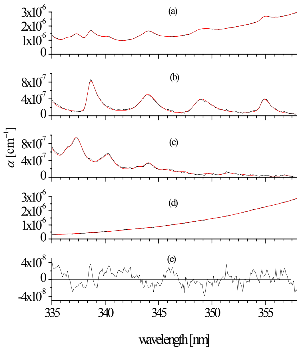
Figure 3.10 Absorption and fitted spectra for the \text{Br}_2 , \text{O}_3 , and \text{BrO} system. (a) Measured spectrum (black) and fitted result (red). The individual components of the spectrum are (b) \text{BrO} , (c) \text{O}_3 , and (d) \text{Br}_2 . (e) Residual of the fit.
