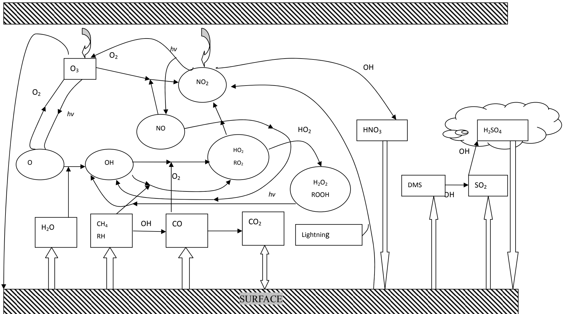
Figure 1.3 Schematic diagram of the relation between the constituents of the global troposphere. After Brasseur et. al. 1999
