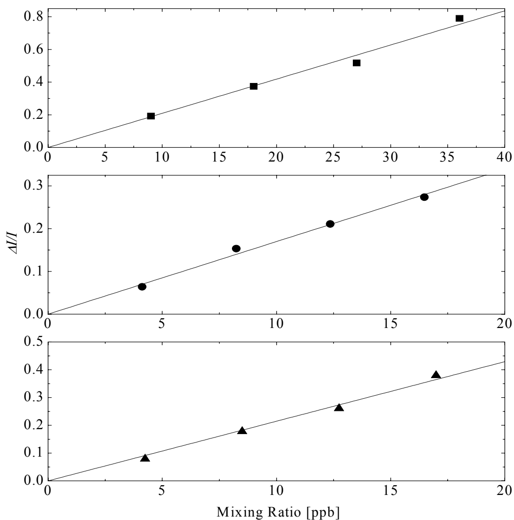
Figure 5.7 Linearity of the absorption with the nitrophenol concentration in the chamber. Top: 2-nitrophenol absorption at 335 nm. Middle: 3-methyl-2-nitrophenol absorption at 337 nm. Bottom: 4-methyl-2-nitrophenol absorption at 345 nm.
