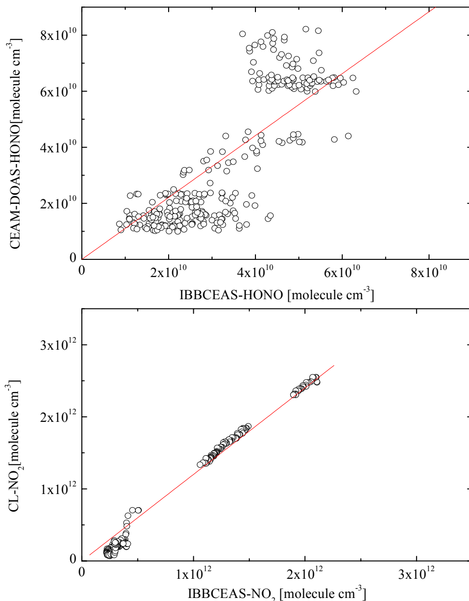
Figure 6.10 Top: the HONO correlation between IBBCEAS and CEAM-DOAS and linearfit (red) with slope=1.1 and R^2=0.89 . Bottom: the \text{NO}_2 correlation between IBBCEAS and CL detector and linear fitting (red) with slope=1.2 and R^2=0.99
