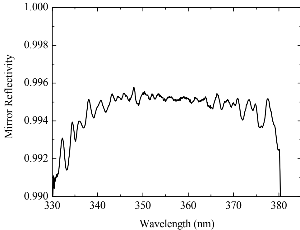
Figure 2.8 Mirror reflectivity calibrated by \text{NO}_2 in a low pressure system. Residual structures are evident in the reflectivity spectrum.
