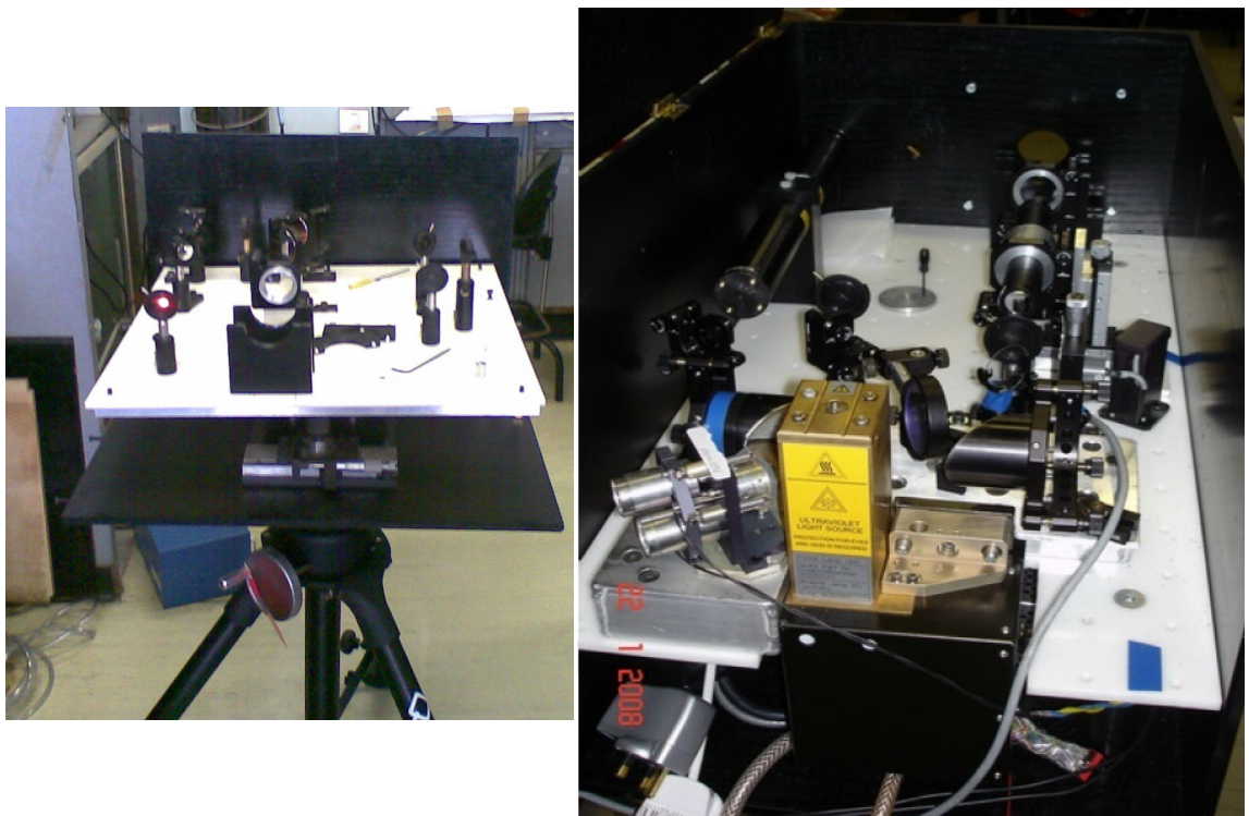
Figure 4.2 TOP: Schematic of the open path field IBBCEAS instrument for the COBRA campaign. BOTTOM: Photographs of the inside of both units (receiver on the left and transmitter on right)
