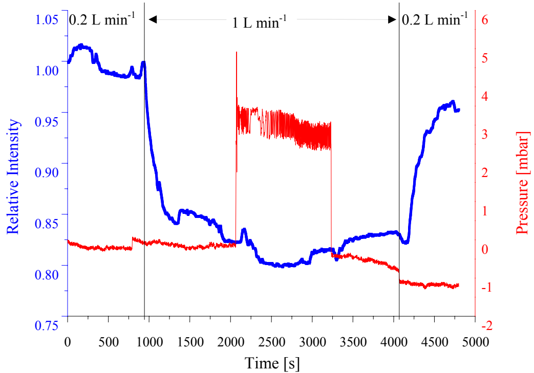
Figure 2.12 Relative intensity variations at 355 nm (blue) at different flow rates and pressures (red). The noise at high pressure is associated with bubbling from the submerged sample gas outlet.
