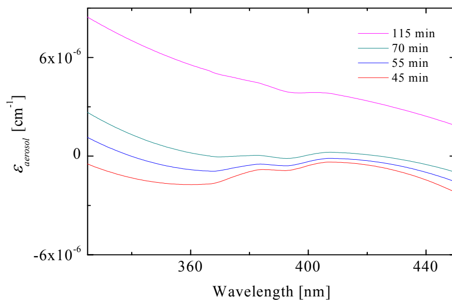
Figure 5.10 Wavelength-dependence of the aerosol extinction at different times
