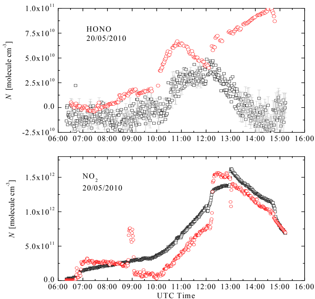
Figure 6.11 Results of IBBCEAS (black) and CEAM-DOAS and CL (red) measurements of HONO and NO 2 .
