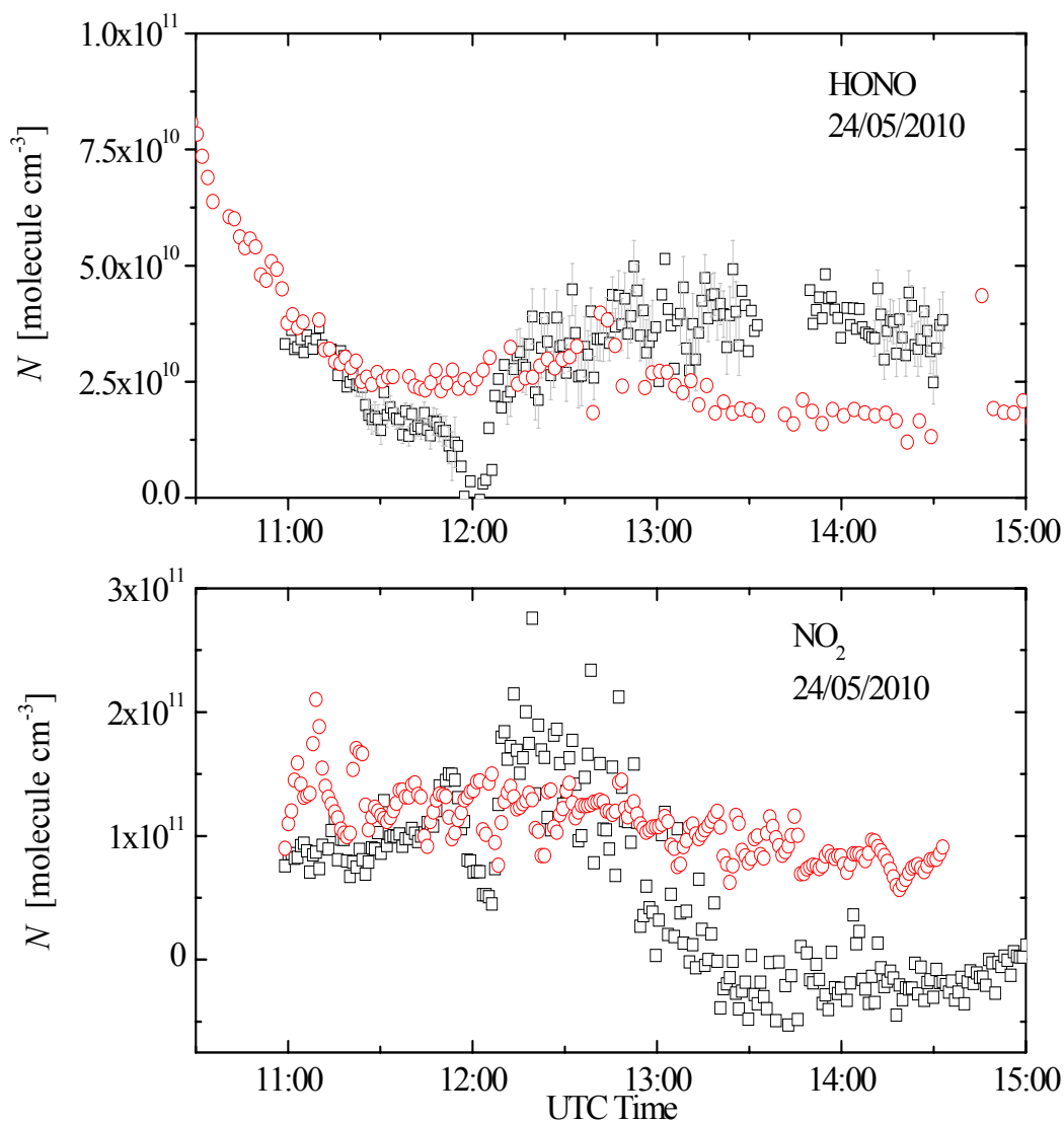
Figure 6.13 Results of IBBCEAS (black) and CEAM-DOAS and CL (red) measurements of HONO and NO 2 .
