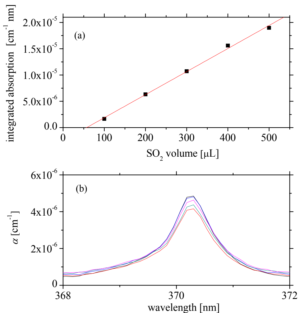
Figure 3.3 (a) Dependence of the \text{SO}_2 integrated absorption on the volume of \text{SO}_2 introduced into the inlet stream. The correlation coefficient of the linear regression is R^2 = 0.9961 . (b) Repeatability of five successive injections of 500 \mu\text{L} \text{SO}_2 into the inlet stream. The standard deviation is 5% at the absorption peak at 370.2 nm.
