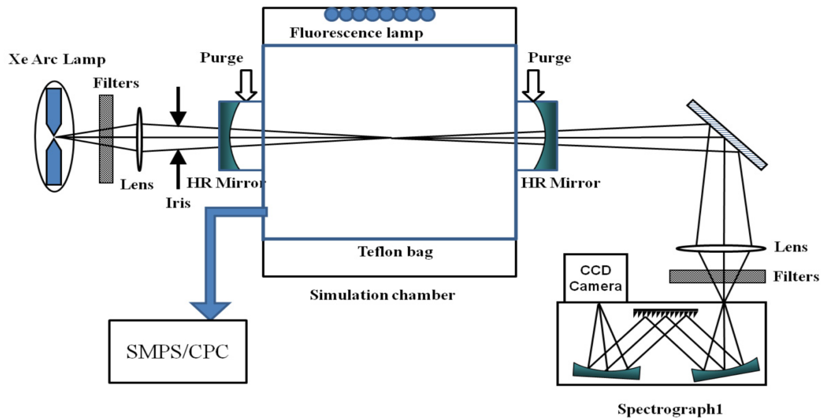
Figure 5.1 Schematic diagram of the IBBCEAS in-situ chamber setup.
