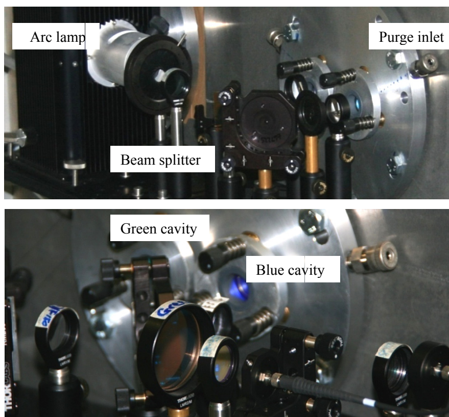
Figure 4.8 Dual cavity IBBCEAS instrument coupled onto the chamber in the Environmental Research Institute, Cork. The transmitter side with arc lamp (top) and the receiver side (bottom).
