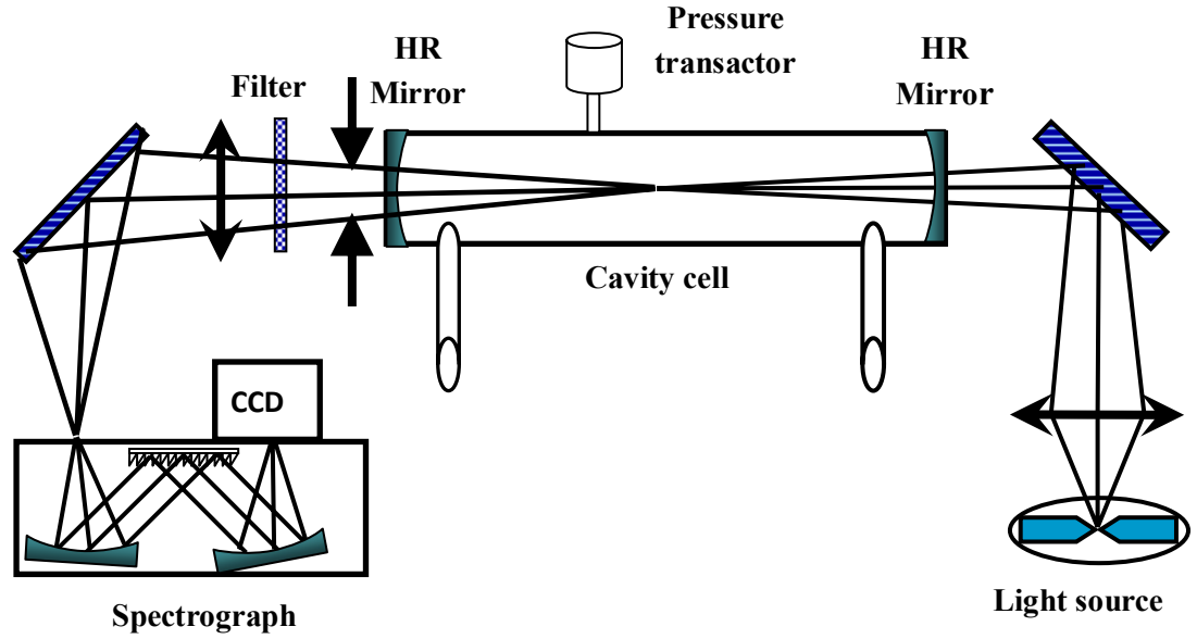
Figure 2.1 Schematic of an incoherent broadband cavity-enhanced spectroscopy system
