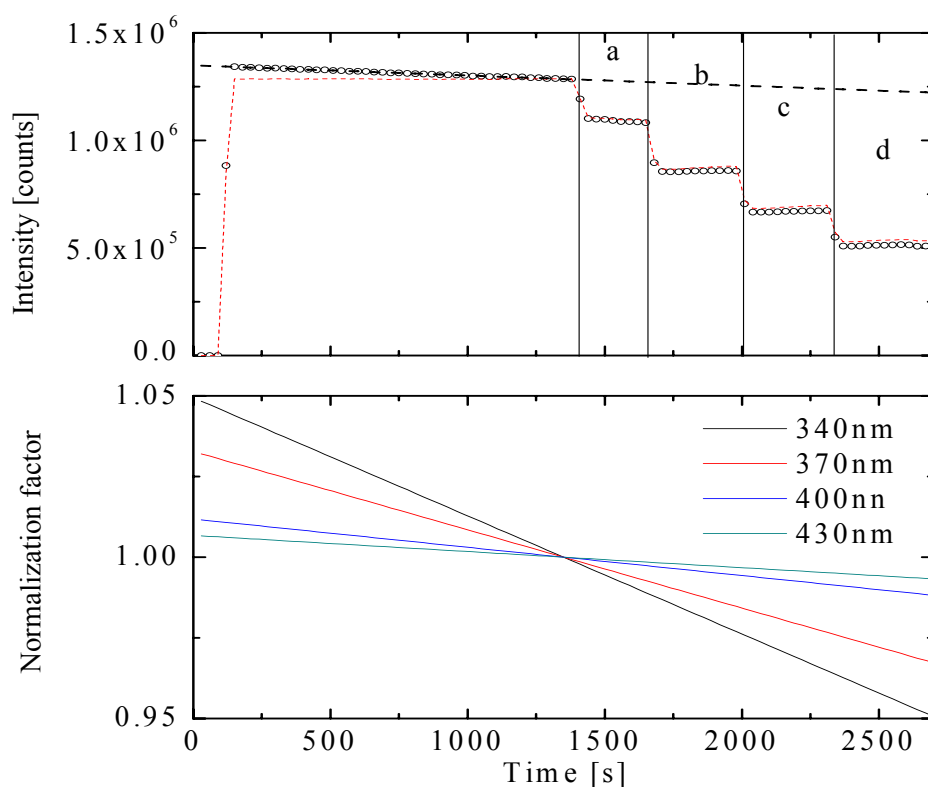
Figure 5.6 Top: The intensity at 340 nm as a function of time for several additions of 2-nitrophenol solution. Bottom: Normalization factors at 340 nm (black), 370 nm (red), 400 nm (blue) and 430 nm, (cyan) nm based on the fitted slope before 1350 s.
