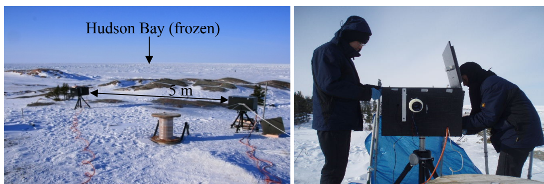
Figure 4.3 Campaign site (left) showing the IBBCEAS system with Hudson Bay in the background. Author and Dr. S. Vaughan aligning the IBBCEAS system (right).
