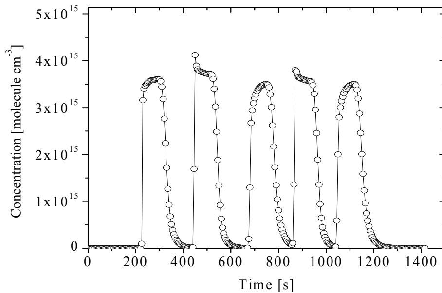
Figure 6.4 Residence time and repeatability of the extractive IBBCEAS instrument from five successive injections of 500 \mu\text{L} \text{SO}_2 .
