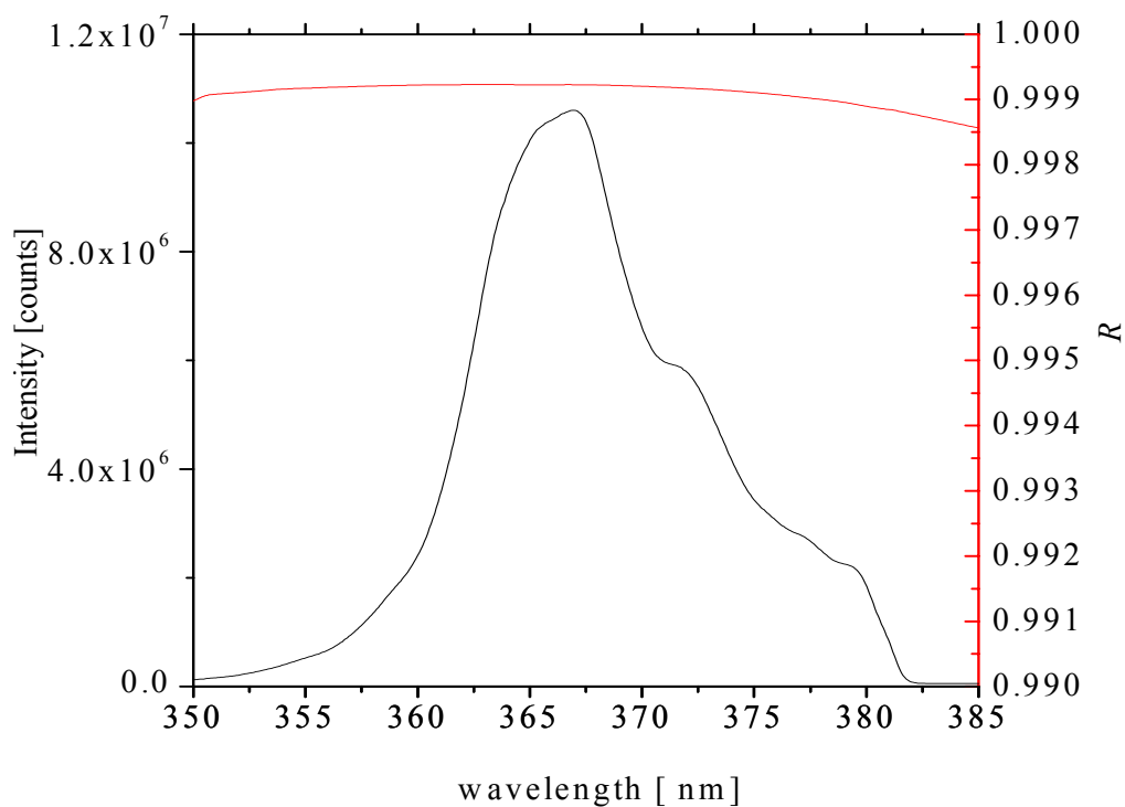
Figure 6.3 Cavity intensity and mirror reflectivity curve from 350 to 385 nm.
