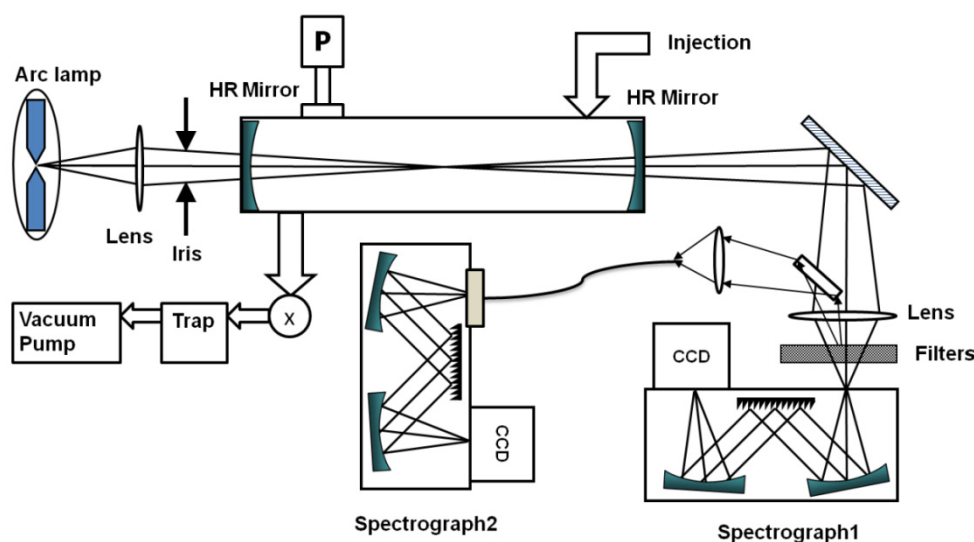
Figure 3.1 Schematic diagram of the IBBCEAS instrument. Spectrograph 1 recorded the IBBCEAS spectra, while spectrograph 2 recorded single-pass spectra outside of the cavity mirror reflectivity range.
