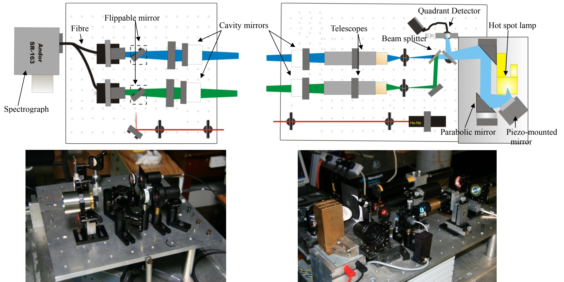
Figure 4.5 Schema (top) and photograph (bottom) of the dual cavity IBBCEAS instrument. The transmitter platform is shown on the right and receiver on the left.
