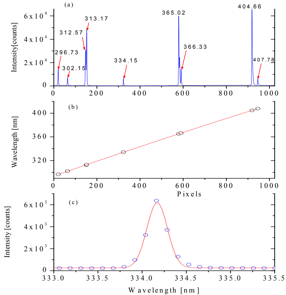
Figure 2.7 (a) A near-UV spectrum of the HgNe penray lamp as recorded by the spectrograph. (b) A 3 rd order polynomial fit of the wavelength to the pixels. The uncertainty is about 0.02 nm. (c) A Gaussian fit to the 334.15 nm mercury emission line showing a FWHM of 0.27 nm.
