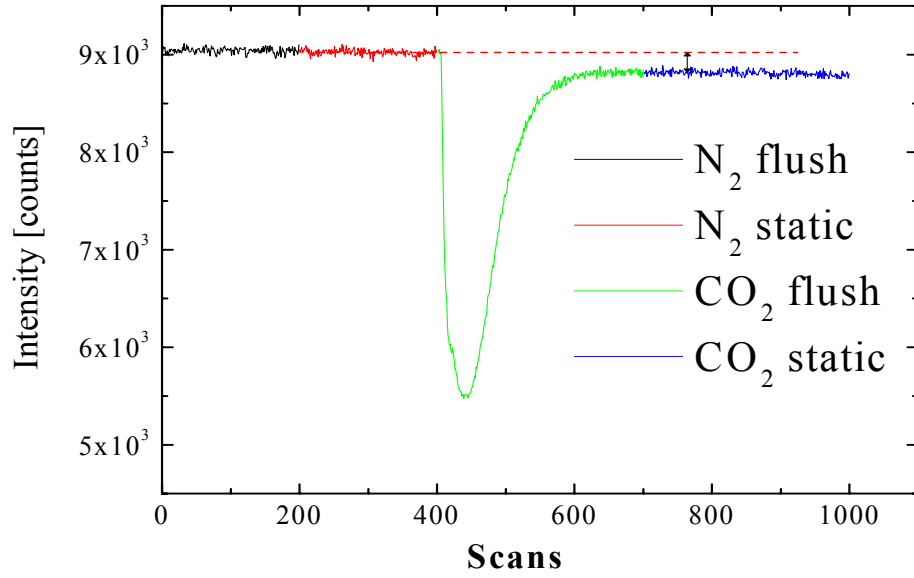
Figure 2.9 The calibration of the mirror reflectivity based on the different Rayleigh scattering of N_2 and CO_2 .
