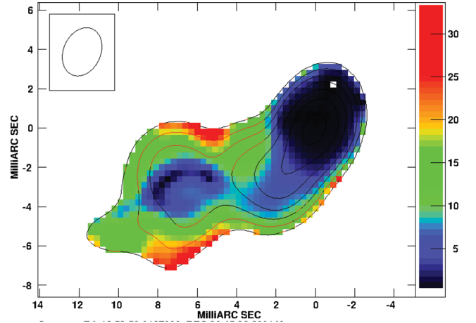
Figure 10. 6-cm total intensity contours given in Fig. 3 superposed with a colour image of the distribution of the degree of polarization. The increase in the degree of polarization towards the edges of the jet, also reported by Pushkarev et al. (2005), is clearly visible. The locations of the highest degrees of polarization do not coincide with those expected for curvature-induced polarization.
