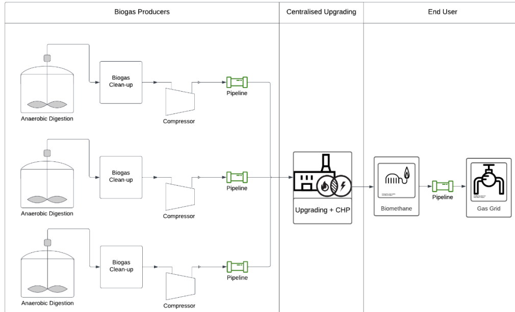
Figure 6-3 Centralised biomethane production diagram.
