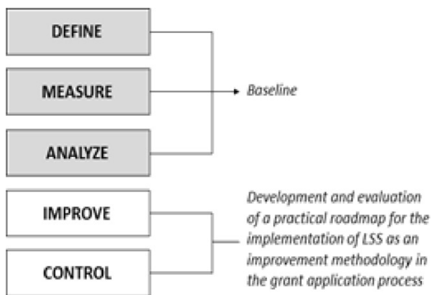
Fig. 1. DMAIC.
