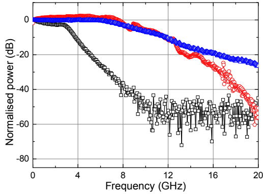
Fig. 2: S_{21} characterisation for: a typical directly modulated laser (black, squares), external modulator and 2µm detector at 1.5µm (blue, triangles) and at 2µm (red, circles).
