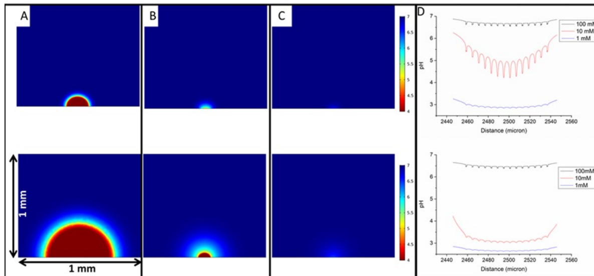
Fig. 4. Top Panel: Simulated pH profile after 1 s for an applied current of 100 nA with buffer concentration of 1 (A), 10 (B) and 100 (C) mM with (D) showing a plot of pH across the electrode surfaces; Bottom Panel: Simulated pH profile after 10 s for 100 nA with buffer concentration of 1 (A), 10 (B) and 100 (C) mM with (D) showing a plot of pH across the electrode surfaces.
