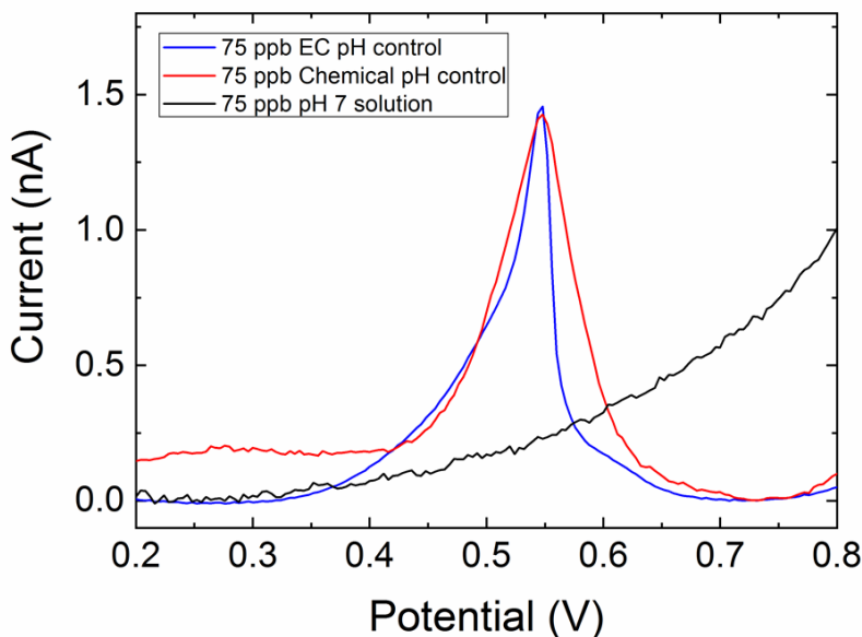
Fig. 7. SWV stripping peak of mercury in an untreated pH 7 solution, in a chemically acidified solution of pH 3.5, and a pH 7 solution with the protonator biased at 1.74 V.
