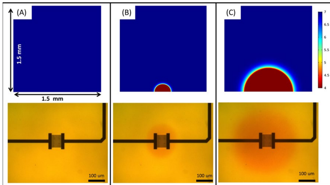
Fig. 6. Top panel: Simulated pH profile of proton generation at protonator electrodes at 0 (A), 1 (B) and 10 (C) seconds in 1 mM buffer; Bottom panel: Optical images of working electrode array as current applied at protonators at 0 (A), 1 (B) and 10 (C) seconds.
