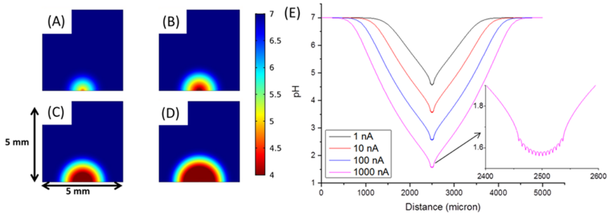
Fig. 1. The simulated pH profile after 10 s with applied current of (A) 1, (B) 10, (C) 100 and (D) 1000 nA at protonators (Surface Area 693 \mu\text{m}^2 ); (E) Plot of pH at electrode top surfaces versus width of model domain. Inset: Magnified image of region directly surrounding electrode array with an applied current of 1000 nA.
