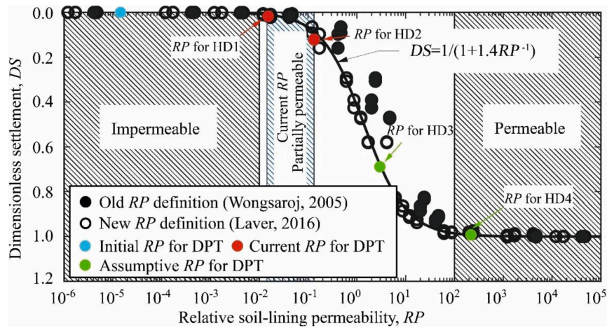
Fig. 5. Previous relative soil-lining permeability ratios (Laver et al., 2017; Wang et al., 2025; Wongsaroj, 2005).
