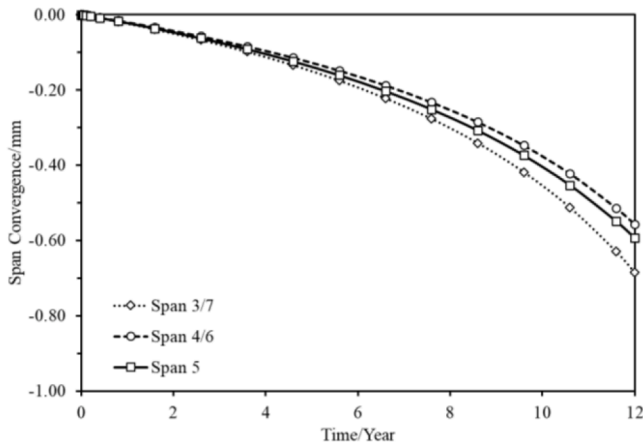
Fig. 17. Incremental tunnel convergence at DFOS spans during mechanical deterioration.
