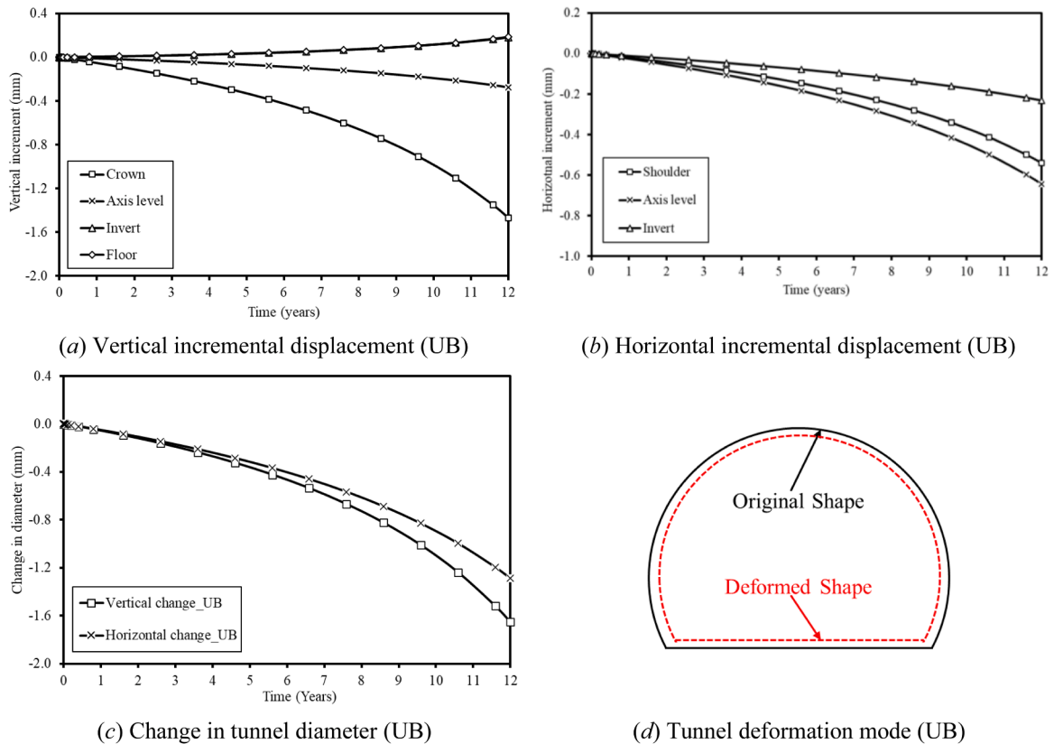
Fig. 16. Incremental tunnel deformation at geodetic locations during mechanical deterioration.
