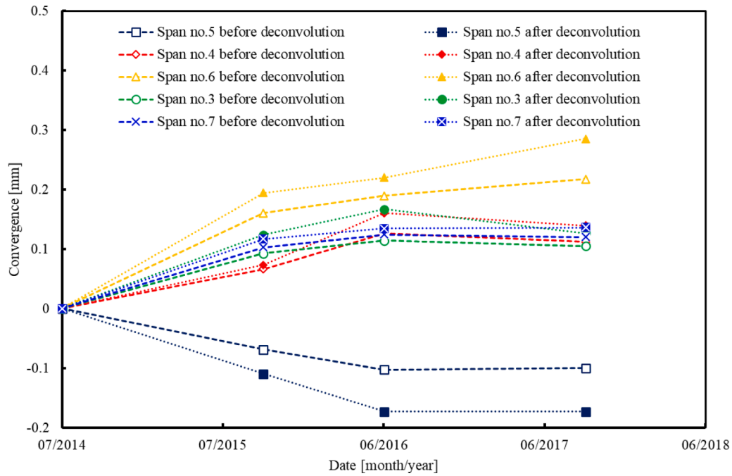
Fig. 11. Tunnel convergence converted from DFOS measurements.
