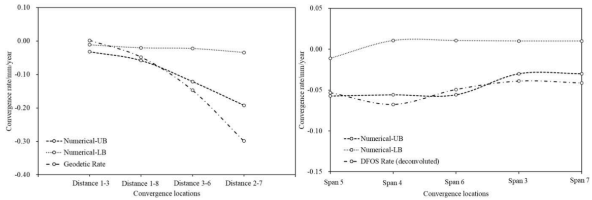
Fig. 21. Comparison between numerical and field deformation rates under hydromechanical deterioration.
