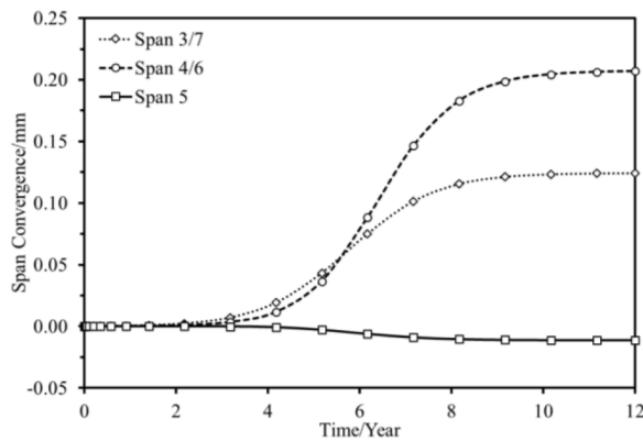
Fig. 14. Incremental tunnel deformation at DFOS spans during hydraulic deterioration.
