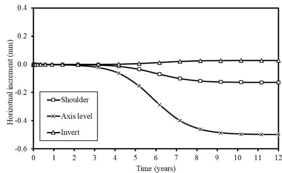
(b) Horizontal incremental displacement (UB)
