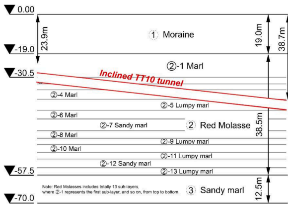
Fig. 3. Ground profile around a section of the TT10 tunnel.
