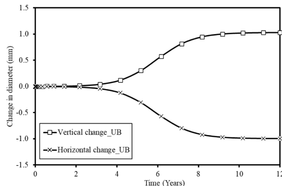
(c) Change in tunnel diameter (UB)
