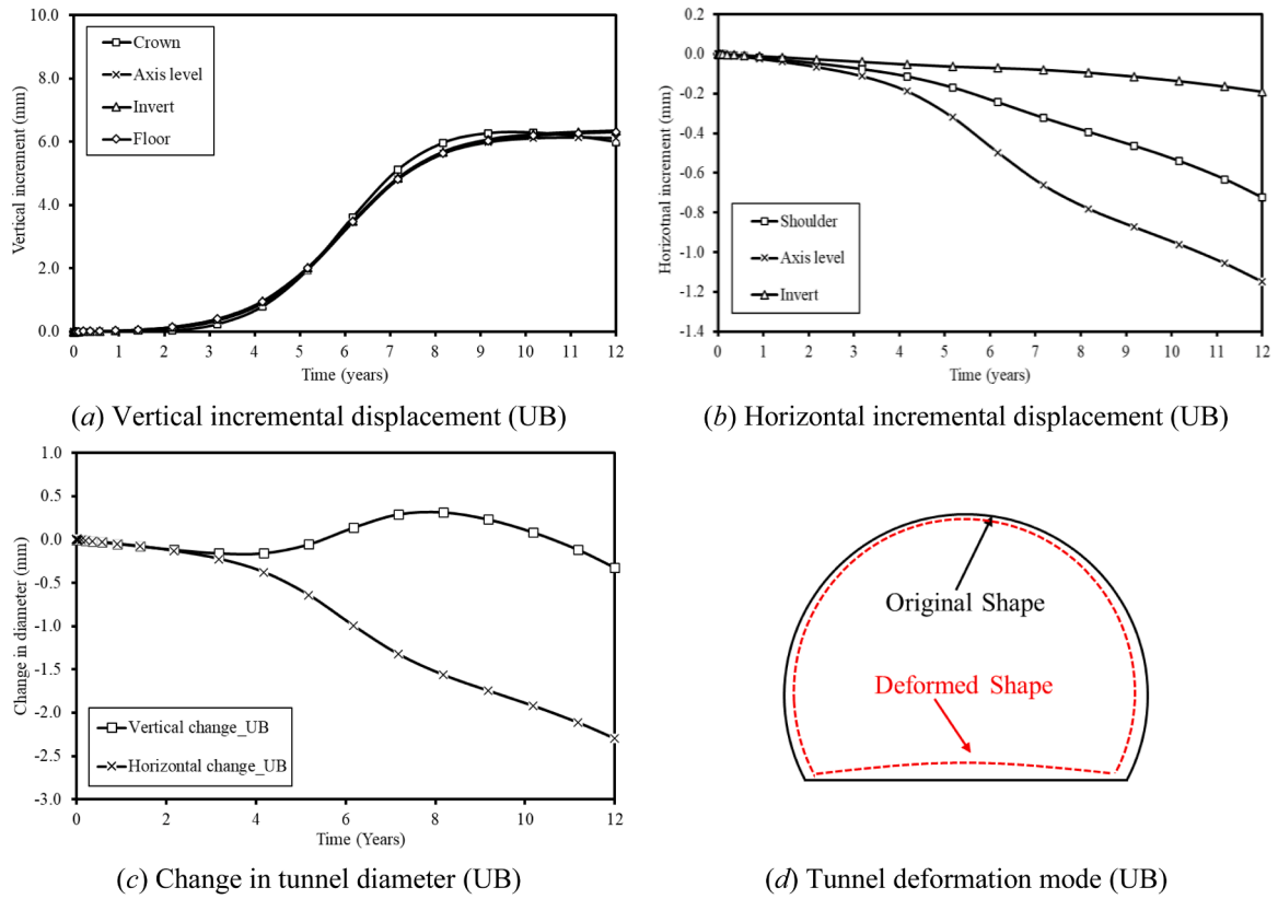
Fig. 19. Incremental tunnel deformation at geodetic locations during coupled hydromechanical deterioration.
