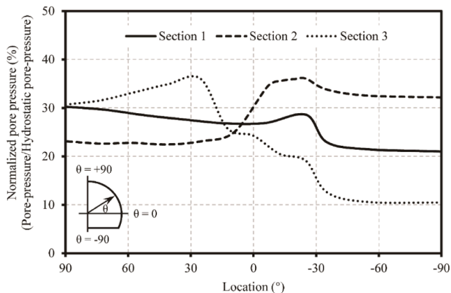
Fig. 26. Comparison of normalised pore water pressure distributions for the three tunnel cross-sections.
