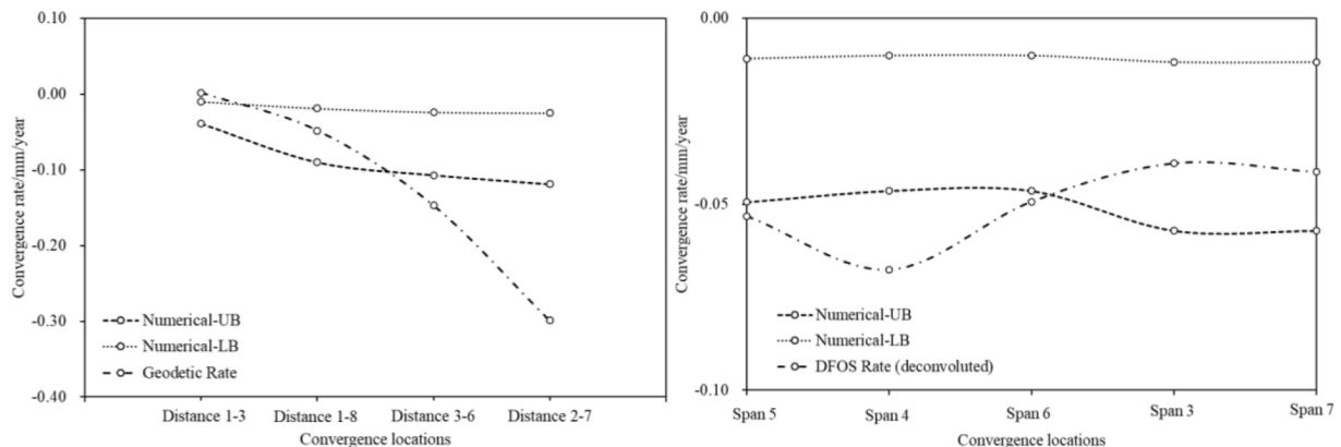
Fig. 18. Comparison between numerical and field deformation rates under mechanical deterioration.
