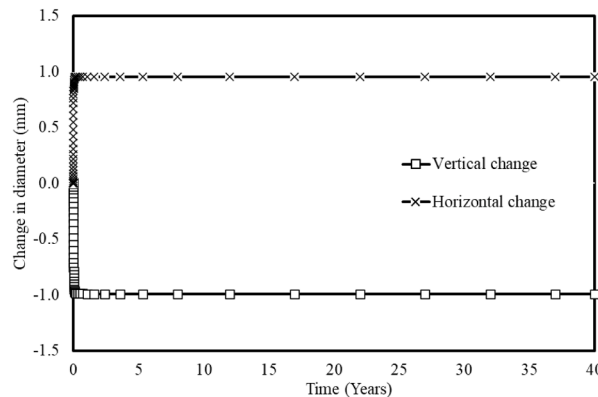
(c) Change in tunnel diameter and tunnel deformation mode
