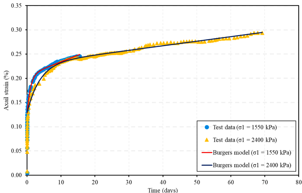
Fig. 7. The comparison between the Burgers model and the experiment curves.
