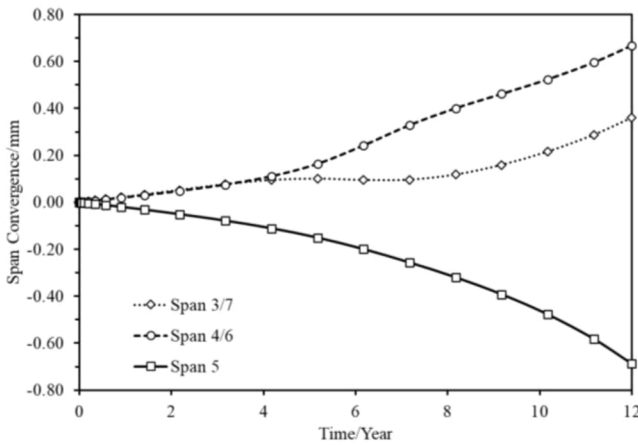
Fig. 20. Incremental tunnel convergence at DFOS spans during hydromechanical deterioration.
