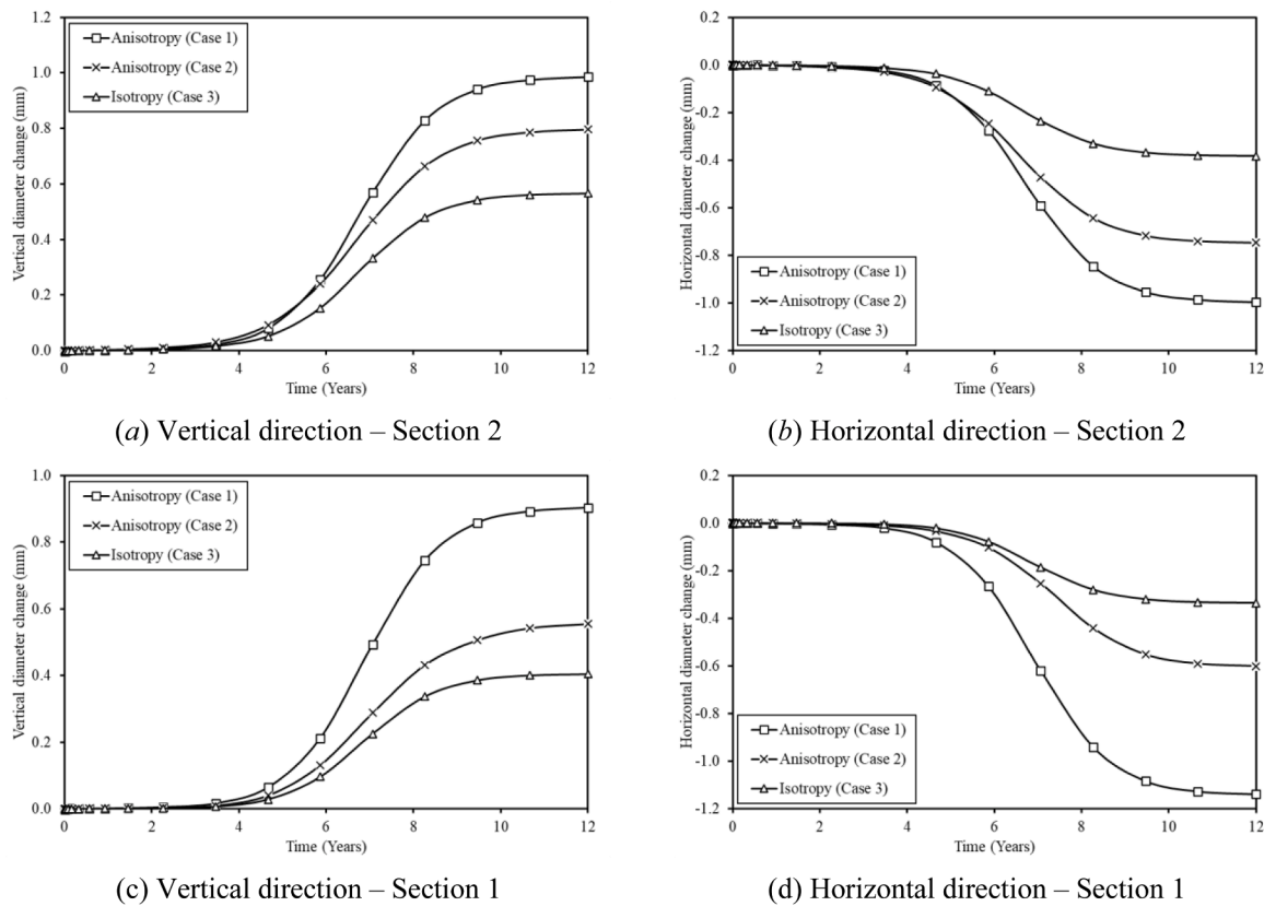
Fig. 28. Change in tunnel diameter for Sections 2 and 1 with permeability anisotropy of various ground unit during hydraulic deterioration stage.
