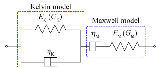
Fig. 6. Burgers model comprising of Kelvin and Maxwell model.
