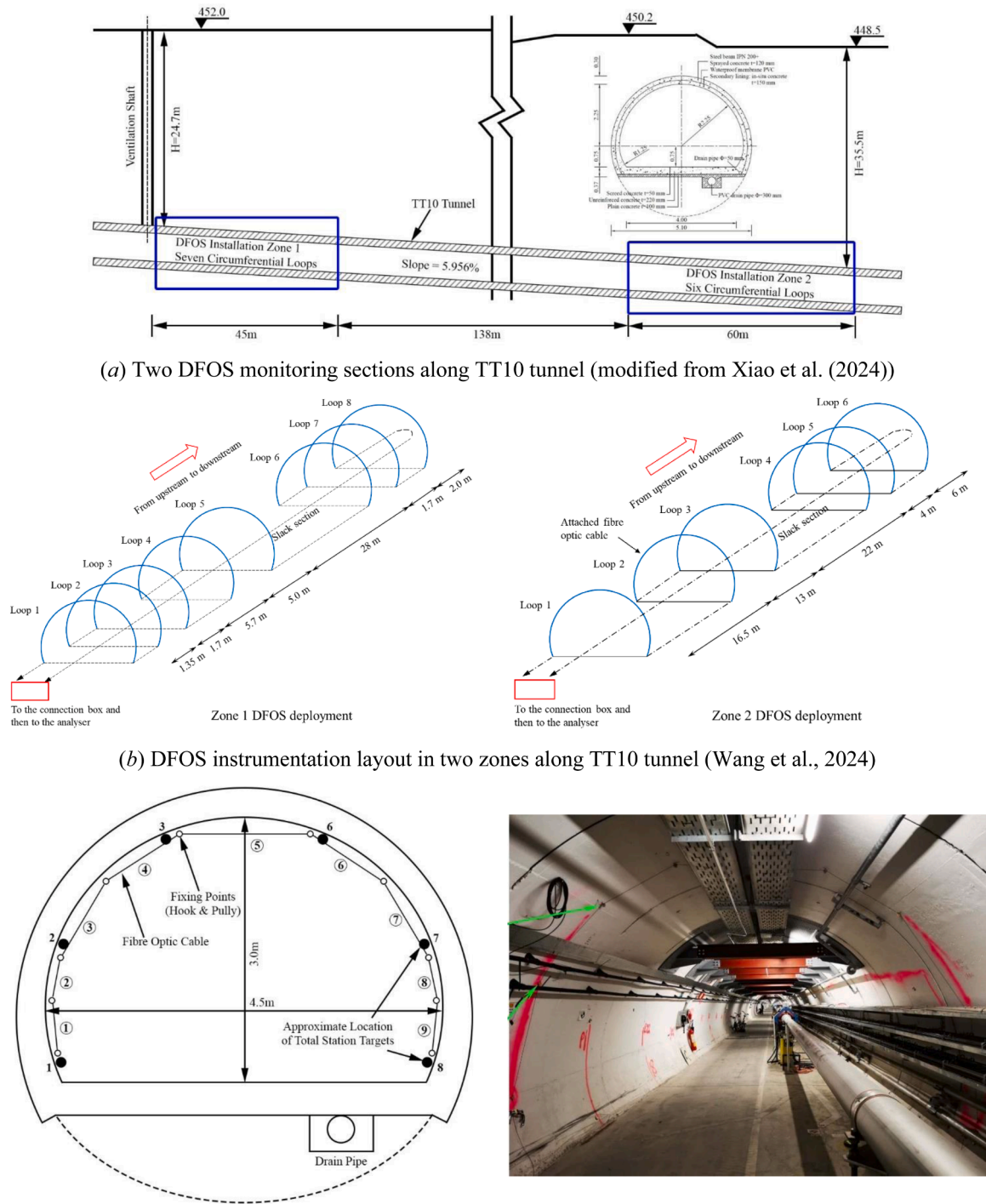
Fig. 10. Details of DFOS Monitoring along TT10 Tunnel.
