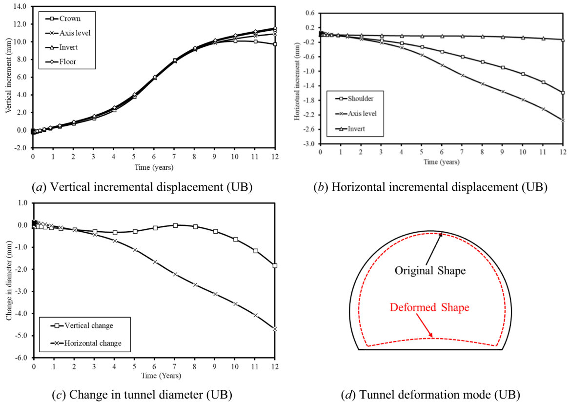
Fig. 22. Incremental tunnel deformation at geodetic locations subject to coupled marl swelling and tunnel hydromechanical deterioration.
