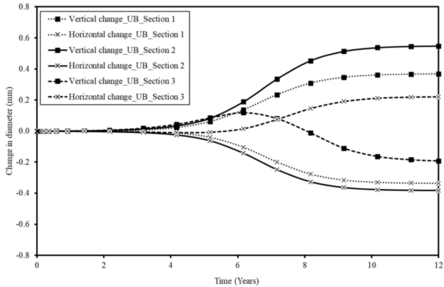
(b) without ground permeability anisotropy
