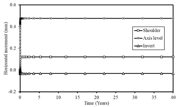
(b) Horizontal incremental displacement
