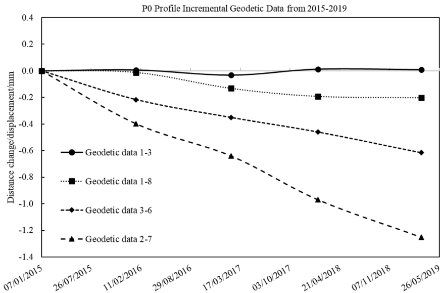
Fig. 9. Geodetic measurements for monitoring profile P0.
