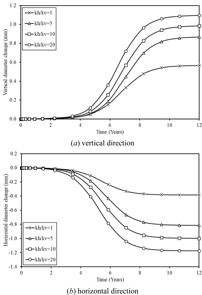
Fig. 27. Change in tunnel diameter with various permeability anisotropy during hydraulic deterioration.
