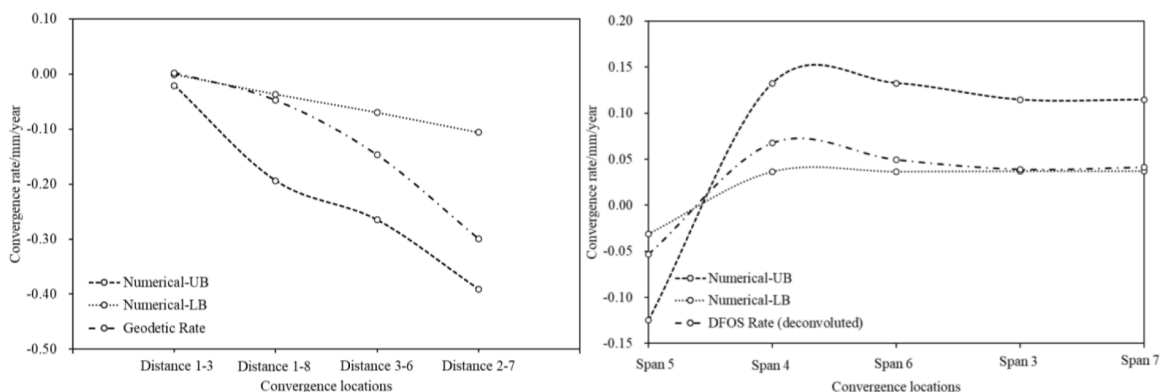
Fig. 24. Comparison between numerical and field deformation rates under coupled marl swelling and hydromechanical deterioration.
