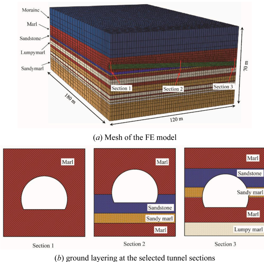
Fig. 4. Finite element model of TT10 tunnel and three representative sections.
