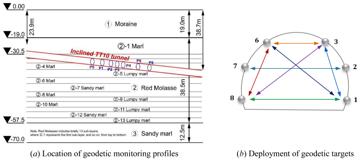
Fig. 8. Geodetic measuring location and deployment along TT10 tunnel.
