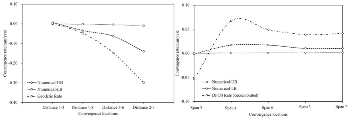
Fig. 15. Comparison between numerical and field deformation rates under hydraulic deterioration.
