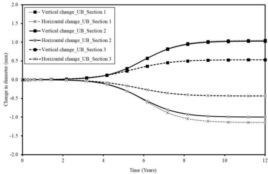
(a) with ground permeability anisotropy ( k_h/k_v=10 )
