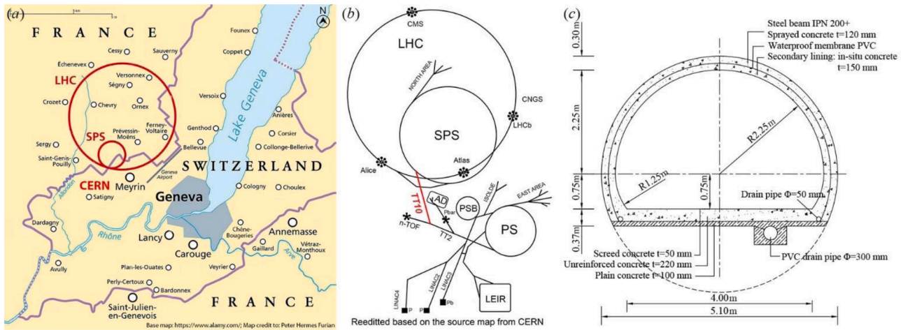
Fig. 1. TT10 tunnel location and cross-section (adapted from Wang et al. (2024)).
