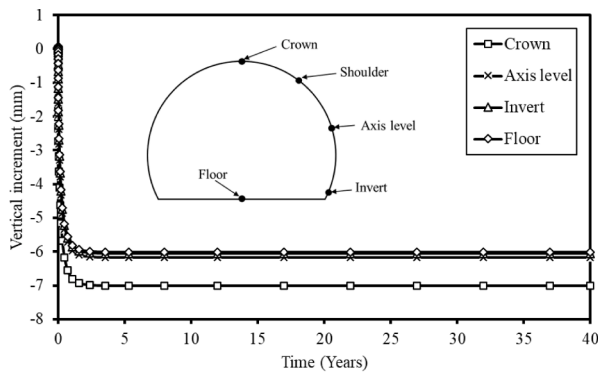
(a) Vertical incremental displacement
