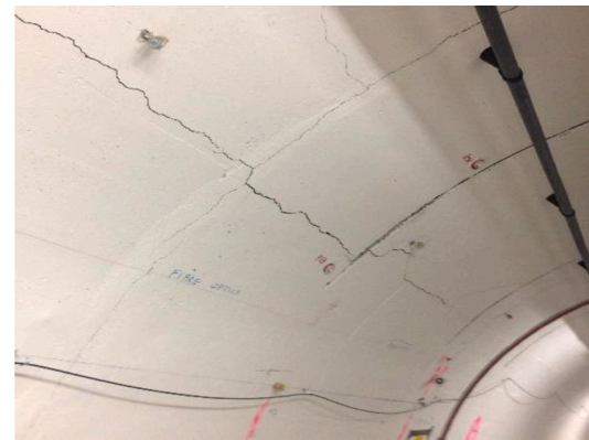
(b) longitudinal cracks at tunnel axis level
