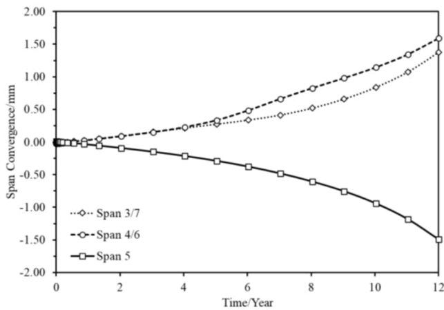
Fig. 23. Incremental tunnel convergence at DFOS spans subject to coupled marl swelling and tunnel hydromechanical deterioration.
