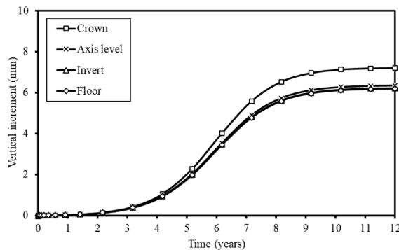
(a) Vertical incremental displacement (UB)
