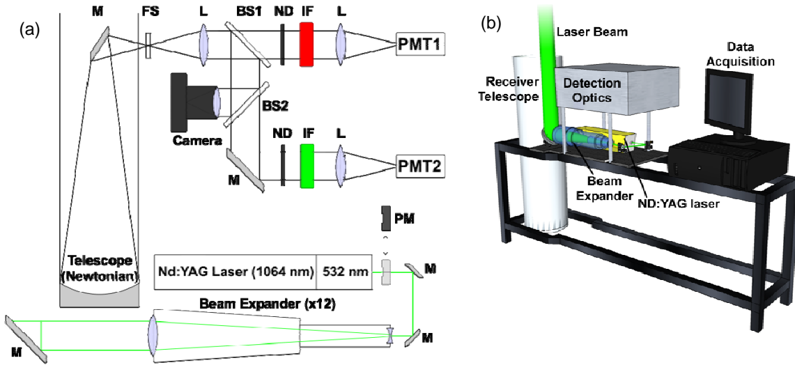
Fig. 1. (a) Schematic of the Rama lidar system UCLID: PM: power meter (optional) FS: Field stop (diameter 0.9 – 5 mm, corresponding FOV 0.6 – 3.33 mrad). L: Lens collimates the beam onto a wavelength dependent beam splitter, BS1. Dichroic beam splitter, BS2: Beam splitter (50:50 ratio). Camera: CMOS is used to monitor the fieldstop. ND: neutral density filters (optional), IF: Interference filter (narrow band), PMT: photomultiplier tube (1:cooled GaAsP, 2:uncooled bi-alkali). (b) UCLID setup, computer (data acquisition), beam expander and Nd:YAG laser, detection optics aligned with the output of the receiver telescope.
