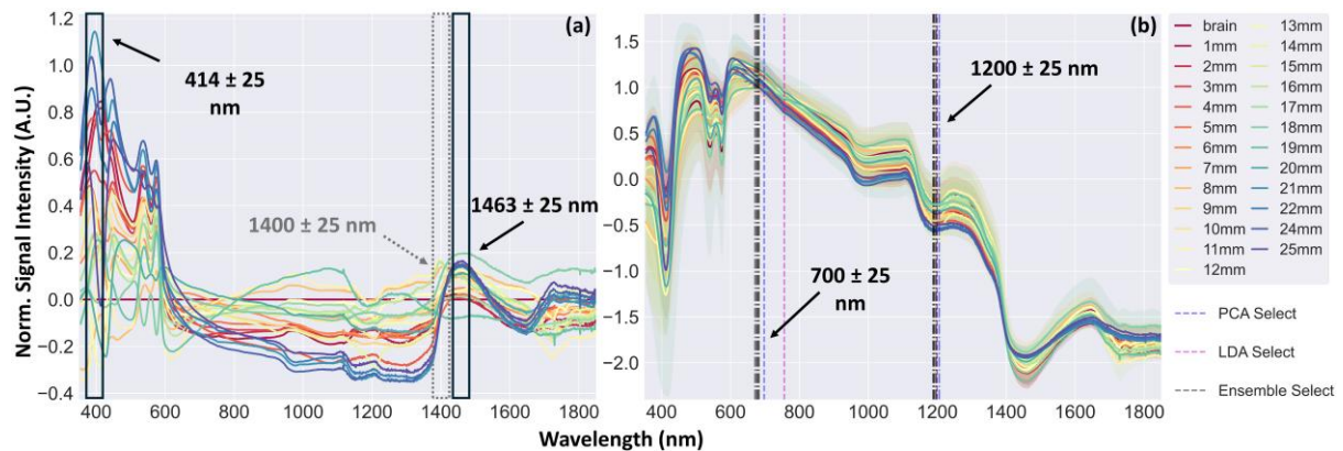
Figure 4.4.1 The selected wavelength features for the OvR binary classification on the SNV-transformed DRS dataset between brain and cranial bone implementing (a) calculation of spectral difference showing features that satisfy user-defined criteria, with one additionally identified feature; and (b) feature selection frameworks based on PCA, LDA and ensemble approach. Number of pig heads = 5; number of drilled holes = 11; number of DRS measurements = 102.
