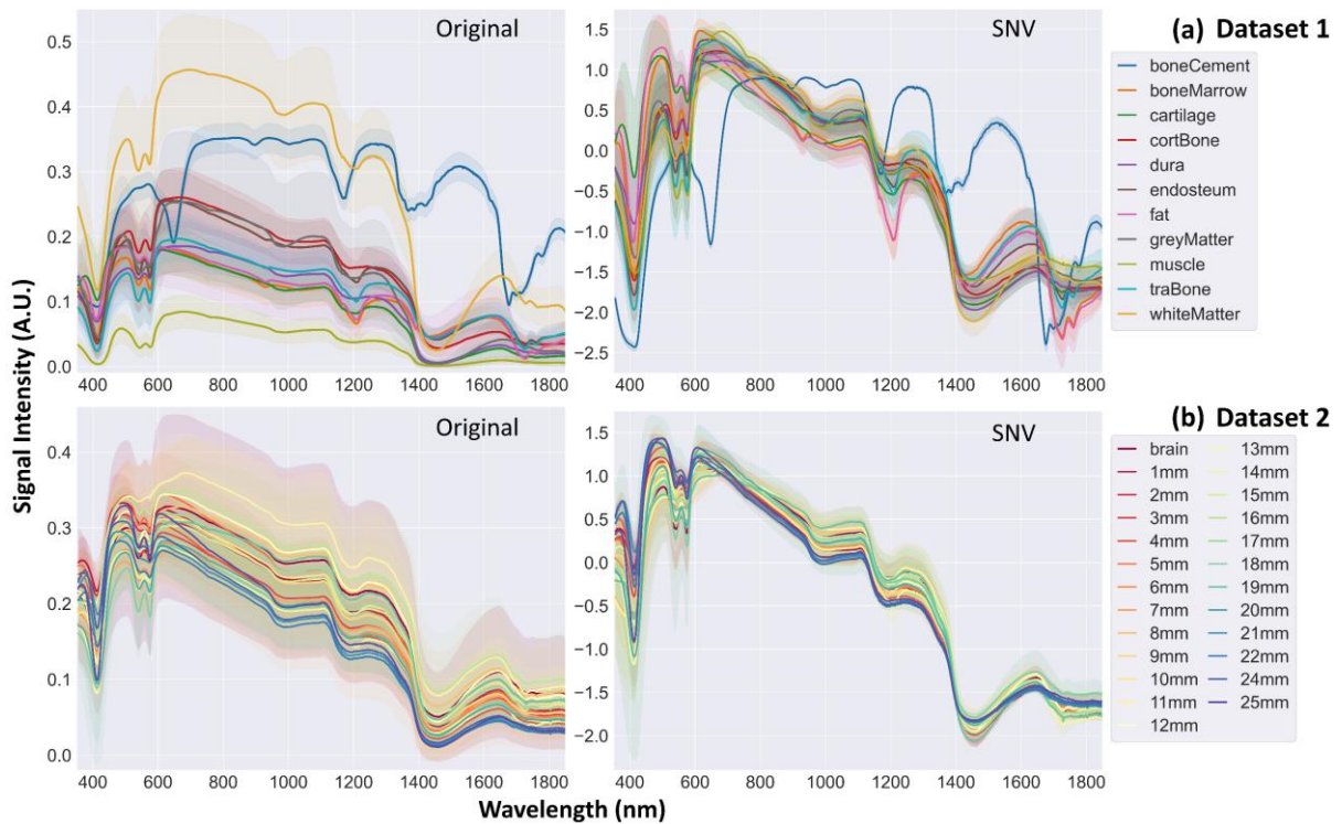
Figure 2.3.1 The averaged EWDRS spectra for all labels in (a) Dataset 1 and (b) Dataset 2 showing the original spectra (left) and the SNV transformed spectra (right). SDs are shown by shaded error bands. Spectral range beyond 1850 nm was trimmed off.
