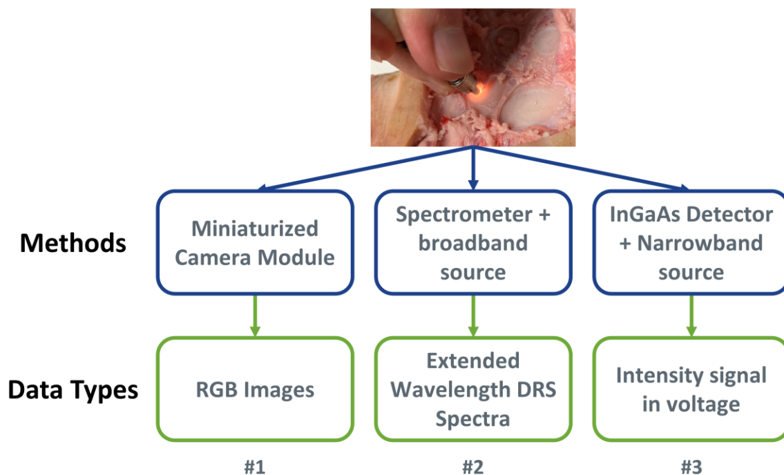
Figure 5.2.3 Workflow of the rTHA simulation experiment consisting of three different methods generating corresponding data types.
