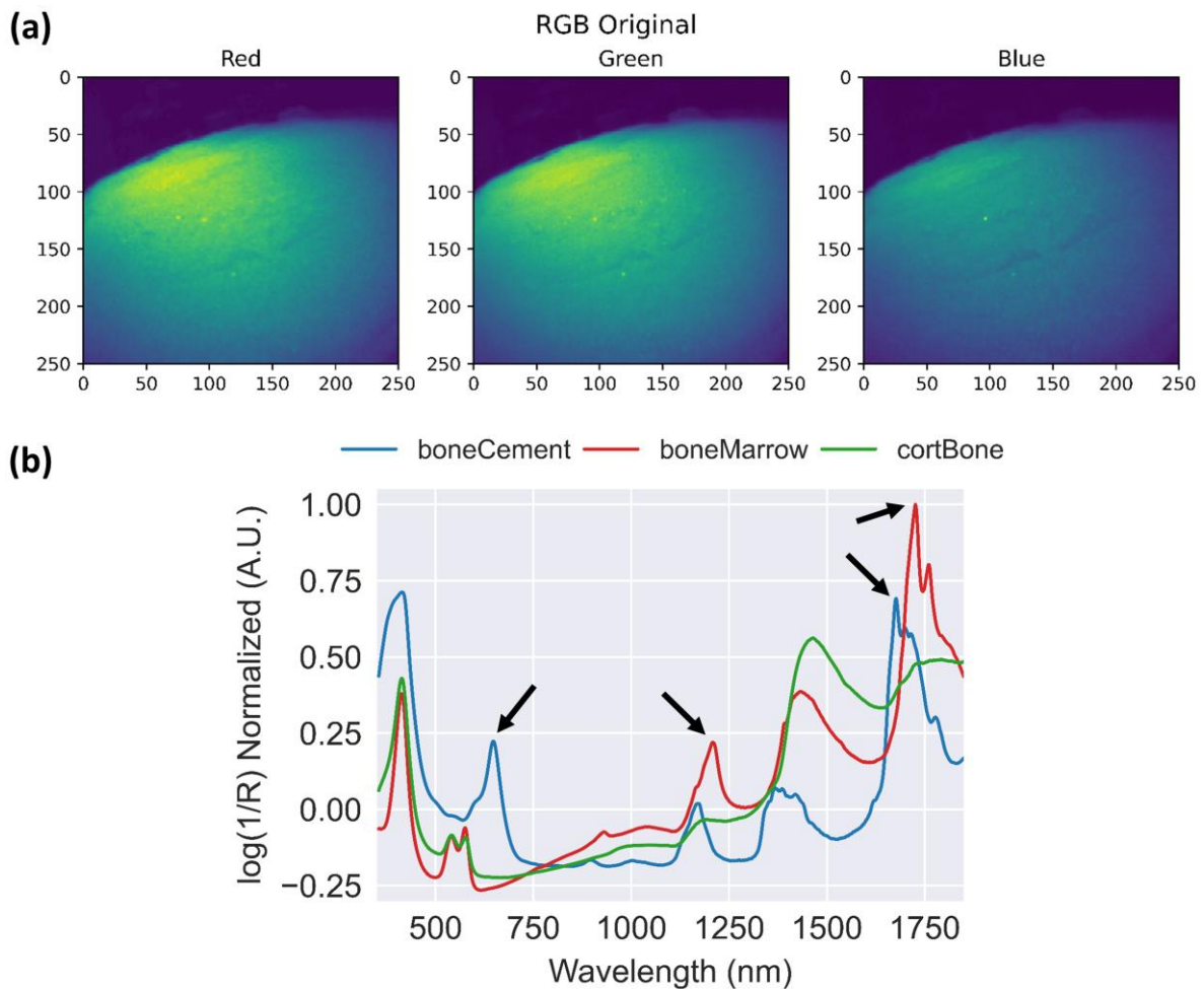
Figure 5.2.4 Initial experiment to test the optical probe. (a) Images showing the original RGB channels from the miniature camera. (b) DRS spectral measurements of bone cement, bone marrow and cortical bone samples. Black arrows indicate the spectral features that could be used to differentiate different tissue types and bone cement.
