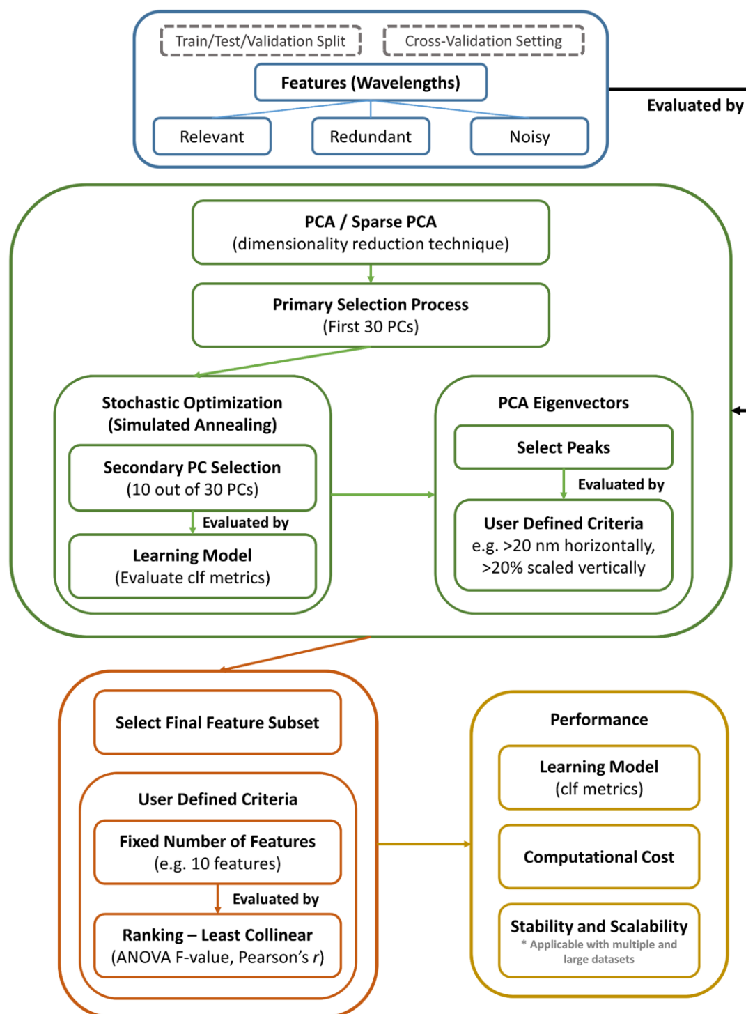
Figure 3.3.3 FS framework implementing PCA/Sparse PCA to process the EWDRS dataset. Acronyms: FS for feature selection; PCA for principal component analysis; PC for principal component; EWDRS for extended-wavelength diffuse reflectance spectroscopy.
