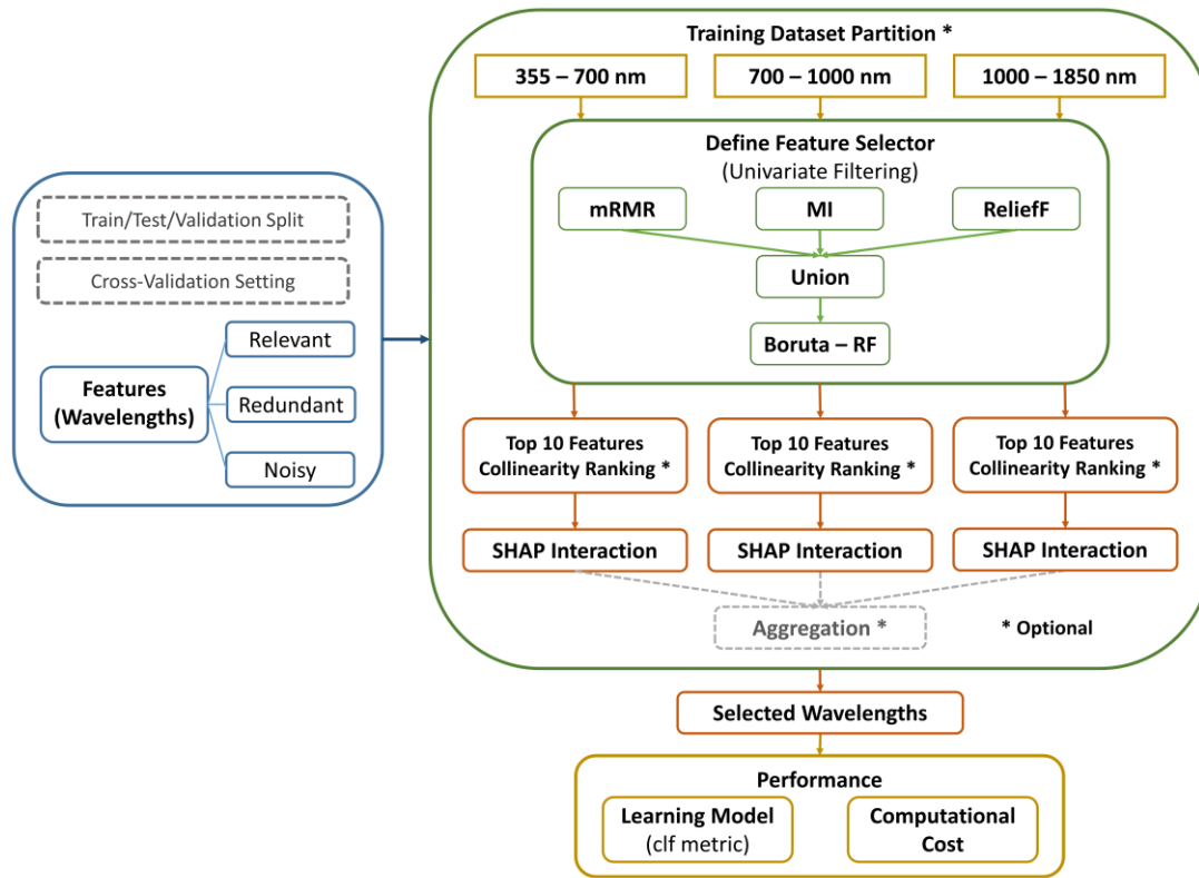
Figure 3.3.6 Ensemble feature selection (EFS) framework. Optional steps are labelled with asterisks, including training dataset partition, sequential removal of collinear features by ranking and aggregation of results from all partitions. Acronyms: mRMR for Maximum Relevance – Minimum Redundancy; MI for Mutual Information; Boruta – RF for Boruta – Random Forest; SHAP for SHapley Additive exPlanations; clf for classification.
