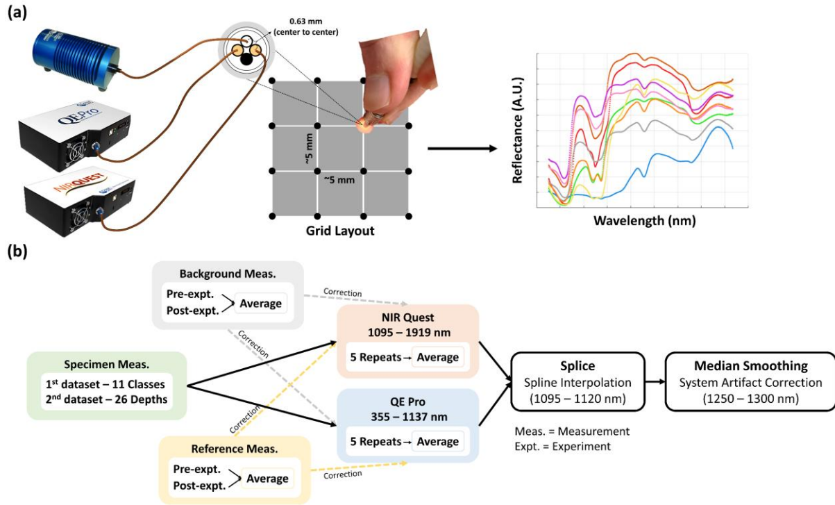
Figure 2.2.1 EWDRS dataset collection and pre-processing workflow. (a) Modified from the publication 186 . Experimental setup included two commercialized spectrometers and a tungsten-halogen broadband light source. The source-detector separations were 0.63 mm from center to center. The locations of measurements followed a grid layout of approximately 5 mm apart for all specimens. (b) Data pre-processing consisted of background correction, reference calibration, spectral splicing using spline interpolation and median smoothing.
