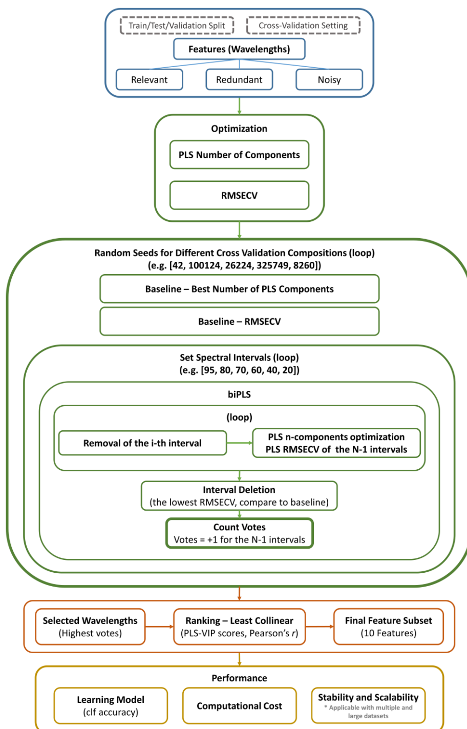
Figure 3.3.5 biPLS FS framework showing the workflow to process EWDRS dataset. Acronyms: biPLS for backward interval partial least squares; FS for feature selection; EWDRS for extended-wavelength diffuse reflectance spectroscopy; PLS for partial least squares; PLS-VIP for PLS-Variable Importance in Prediction; RMSECV for root mean square error of cross-validation; clf for classification.
