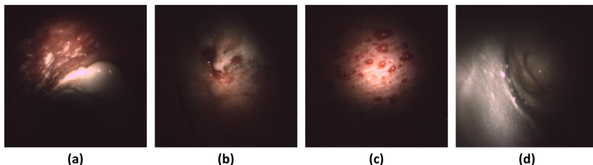
Figure 5.2.6 RGB images acquired by the miniature camera module showing (a) bone-to-cement boundary, (b) distal cement plug, (c) blood drops on trabecular bone and (d) surface characteristics of bone cement.
