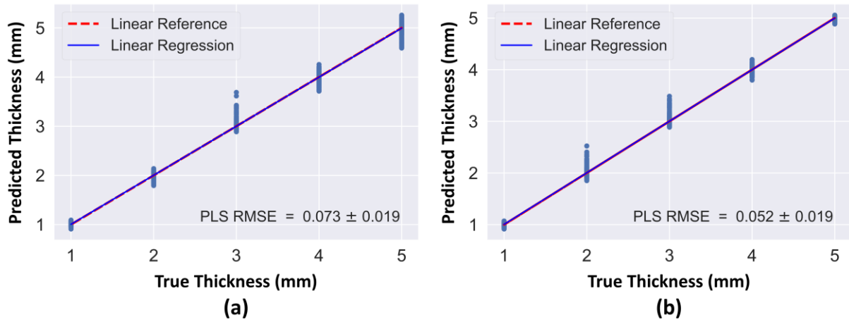
Figure 4.4.3 PLS regression showing the predicted compared to the true thickness of the cranial bone ranging from 1 to 5 mm on the ROSE-SMOTE oversampled dataset with (a) all features and (b) selected features.
