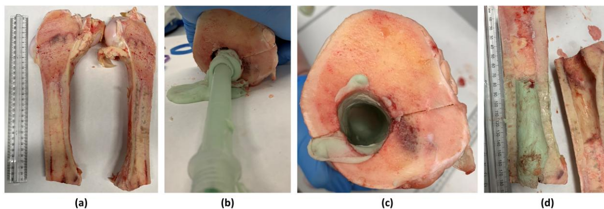
Figure 5.2.2 Bovine femur specimen used in the rTHA simulation experiment showing (a) the original bovine femur cross-sectioned longitudinally, (b) bone cement injection into the femoral column after removal of bone marrow, (c) cemented femoral canal and (d) inside of the bovine femur once the cement was cured.
