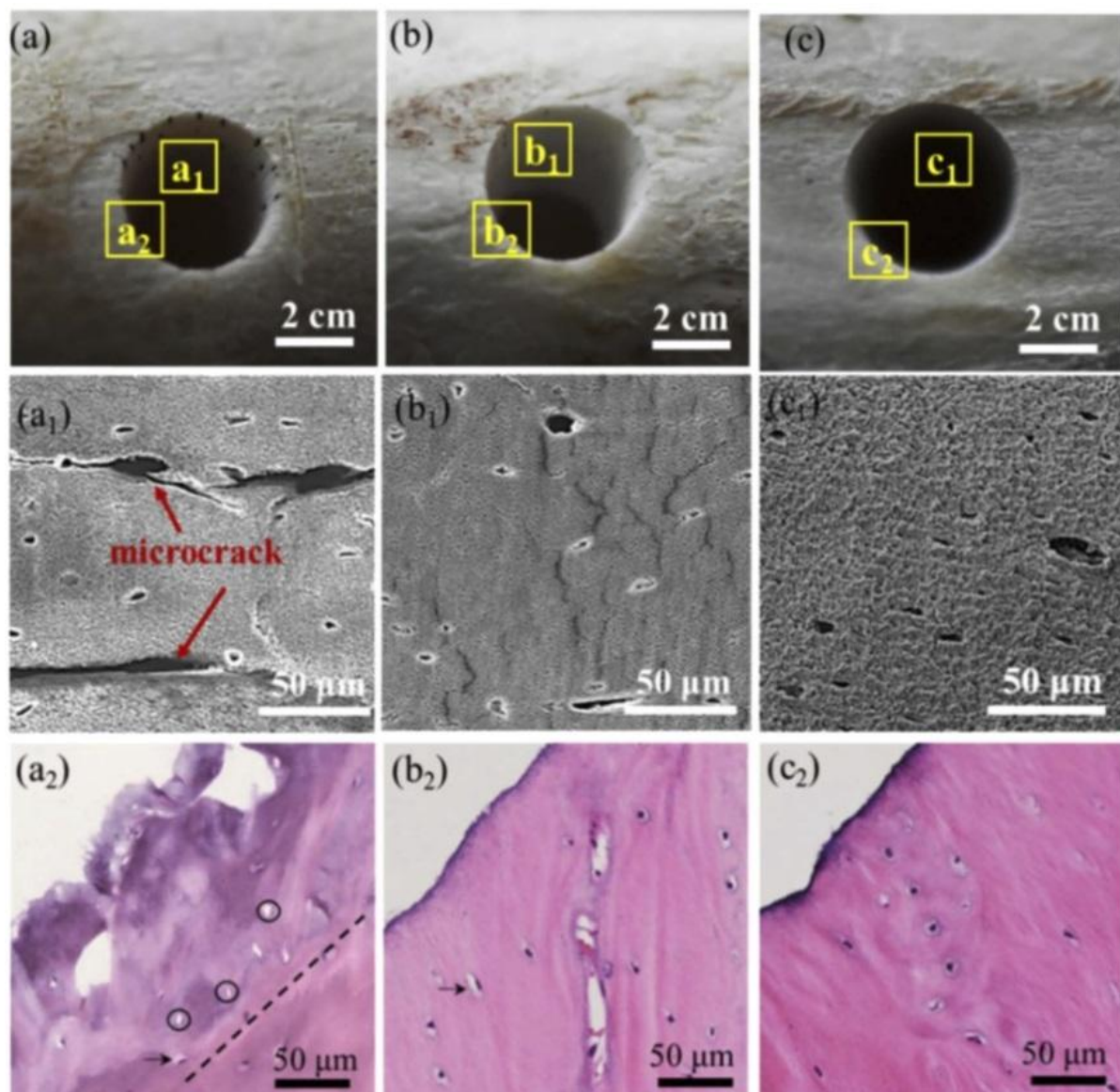
Figure 1.4.2 Morphology of laser-drilled bone tissues under different environmental cooling conditions. Vertical panels (a–c) correspond to without cooling, gas cooling and water cooling; horizontal panels (subscript: none, 1, 2) correspond to white light, SEM and histology images. Adapted from 87 .
