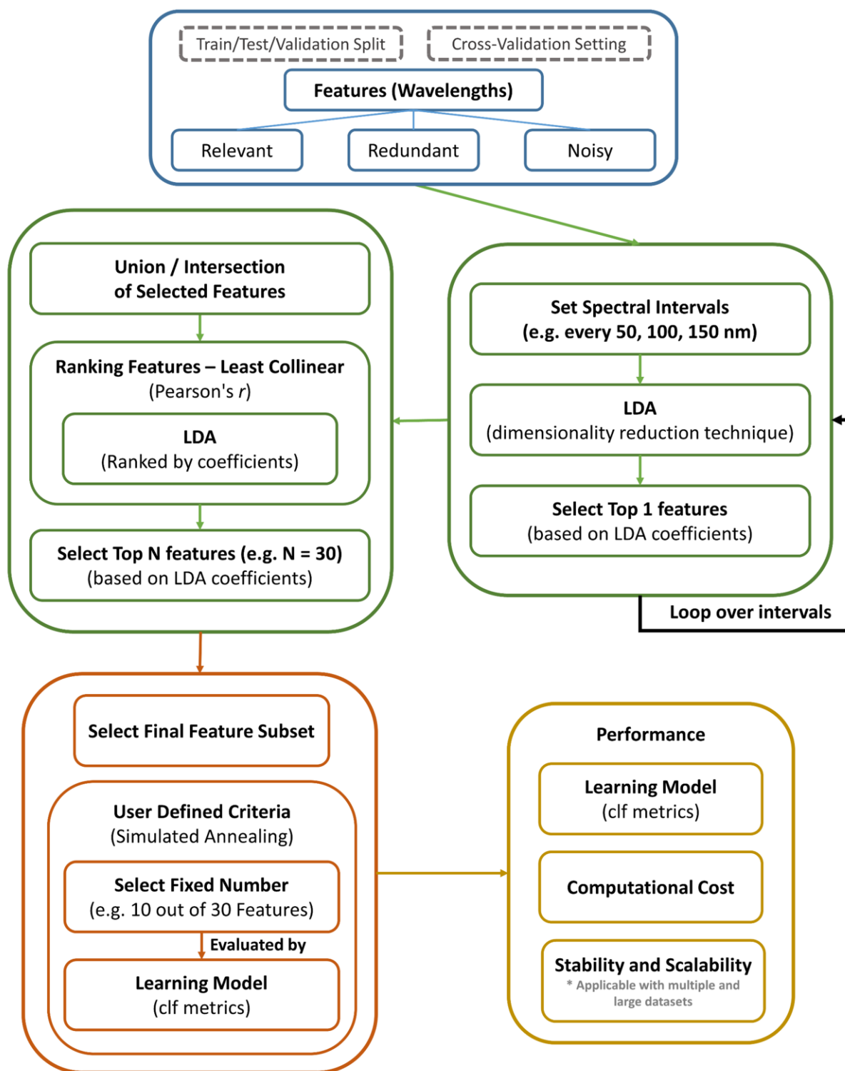
Figure 3.3.4 FS framework implementing LDA to process the EWDRS dataset. Acronyms: FS for feature selection; LDA for linear discriminant analysis; EWDRS for extended-wavelength diffuse reflectance spectroscopy.
