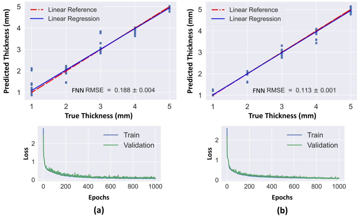
Figure 4.4.4 FNN showing the predicted compared to the true thickness of the cranial bone ranging from 1 to 5 mm on the ROSE-SMOTE oversampled dataset with (a) all features and (b) selected features. Validation loss is shown on the bottom panel.
