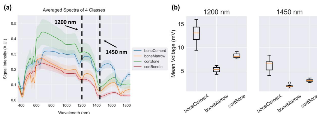
Figure 5.2.7 Results obtained from the optical probe in the rTHA simulation experiment showing (a) broadband DRS from bone cement, bone marrow, cortical bone and inside of cortical bone for 355-1850 nm highlighting lipid absorption at 1200 nm and water absorption at 1450 nm, and (b) mean voltage signals from narrowband DRS at 1200 and 1450 nm for bone cement, bone marrow and cortical bone.
