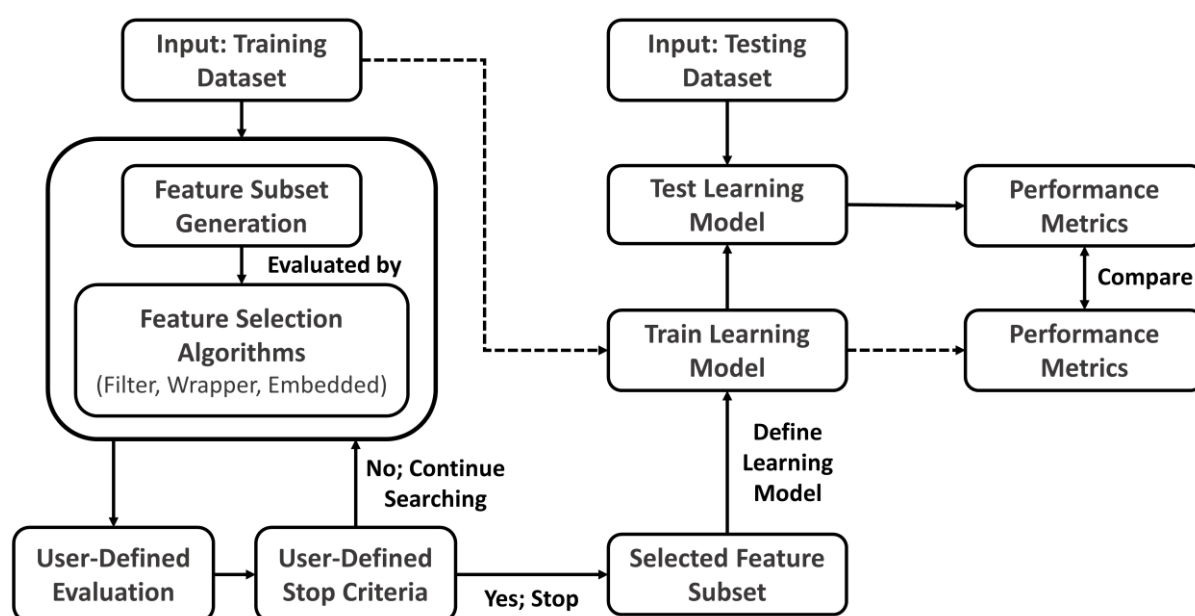
Figure 3.3.2 Overview of a typical feature selection (FS) workflow.
