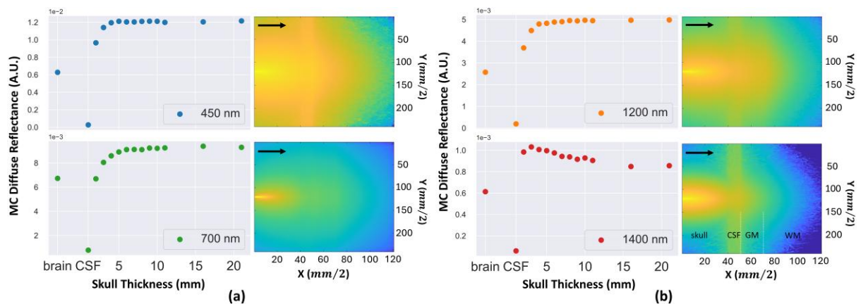
Figure 4.4.2 Monte Carlo simulations of diffuse reflectance as a function of skull thickness (left) and fluence rate distribution (right) at (a) 450, 700, (b) 1200 and 1400 nm in the four-layered head model with separations shown at the bottom right.
