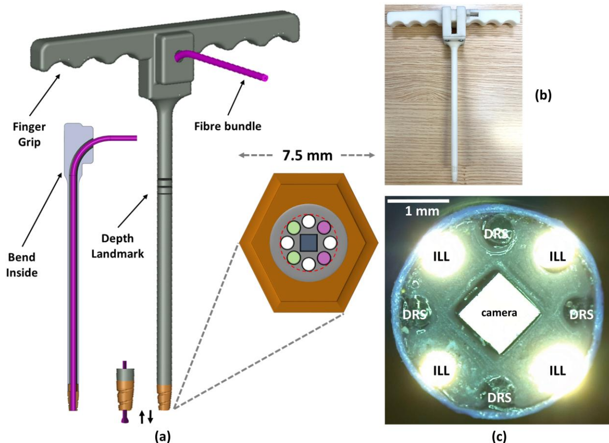
Figure 5.2.1 The optical reamer system for bone cement removal during rTHA. (a) Schematic showing the concept design of the reamer and the optical sensing unit. The miniature camera module (blue square) is positioned in the center of 8 fiberoptic channels arranged equidistantly in a circle (Blue: camera module; green and magenta: DRS acquisition pairs; white: camera illumination (ILL)). (b) 3D printed mock-up reamer. (c) Probe footprint with illumination on.
