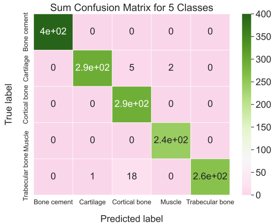
Figure 5.3.5 Confusion matrix for multi-class classification using LDA summed over 100 runs of CV for bone cement, cartilage, cortical bone, muscle and trabecular bone.
