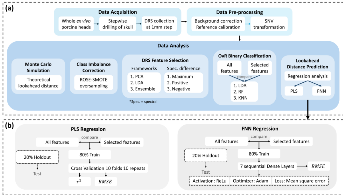
Figure 4.3.1 Experimental workflow. (a) Flowchart of data acquisition, pre-processing and analysis. DRS feature selection frameworks can be found in 200 . (b) Model summary for PLS regression and FNN.
