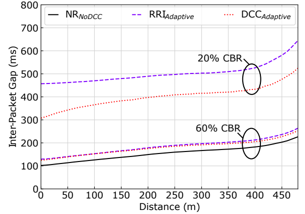
Fig. 5: Comparative Inter-Packet Gap.
