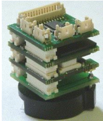
Figure D.1 – TyndallI25 Mote
