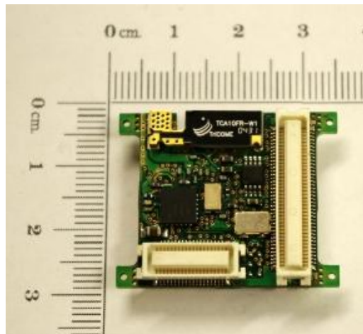
Figure 4.5 – Transceiver Layer
