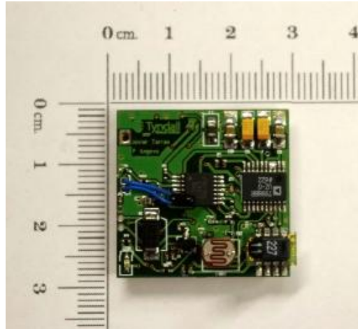
Figure 4.4 – Multi-Sensor Layer
