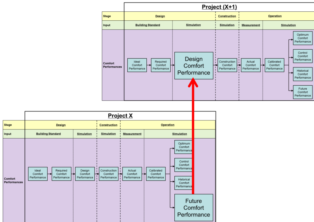
Figure 3.7 – The FCP and DCP Connection
