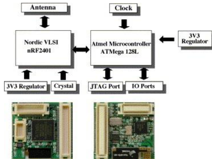
Figure D.2 – Block diagram and final implementation of RF transceiver/microcontroller layer
