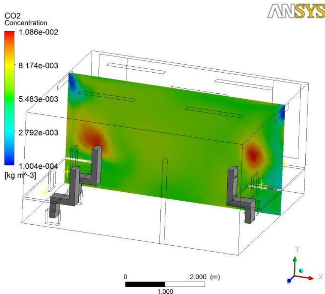
Figure 5.6 – Image of CO 2 Concentration Contour Plot in the Room
