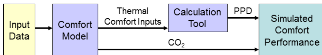
Figure 3.6 - Comfort Performance Creation using the Comfort Model
