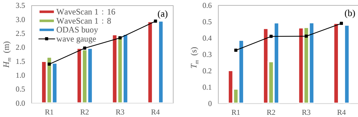
Figure 3 measurements for H_m (a) and T_m (b) during regular wave states(R1-R4)
