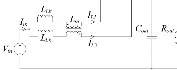
Figure 3.8. CL boost converter operating in regions D_2 and D_4 .
