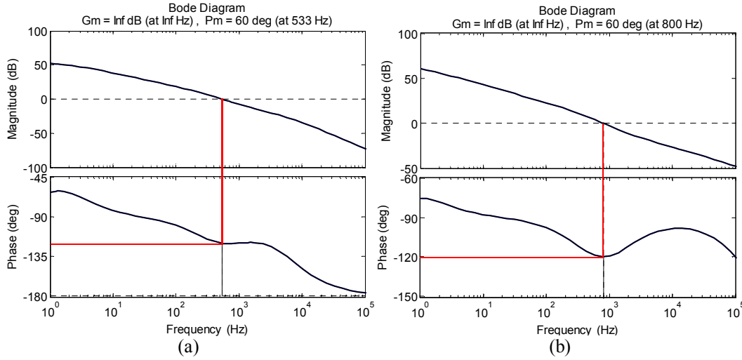
Figure 5.19. Open-loop frequency response of the inner current loop utilising a Type II compensator during (a) DCM 3 and (b) DCM 8.
