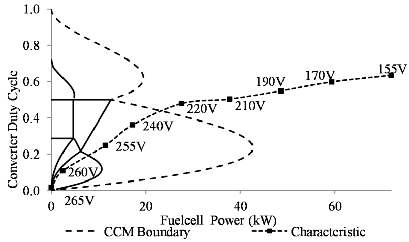
Figure 2.27. CCM-DCM operating mode map for 72 kW CL boost converter.
