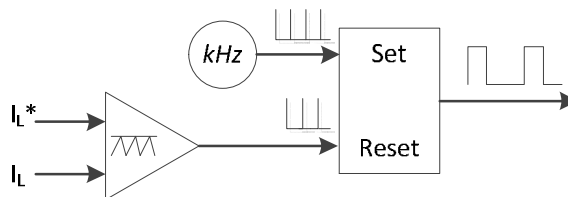
Figure 4.5. Comparator diagram of peak-current mode control
