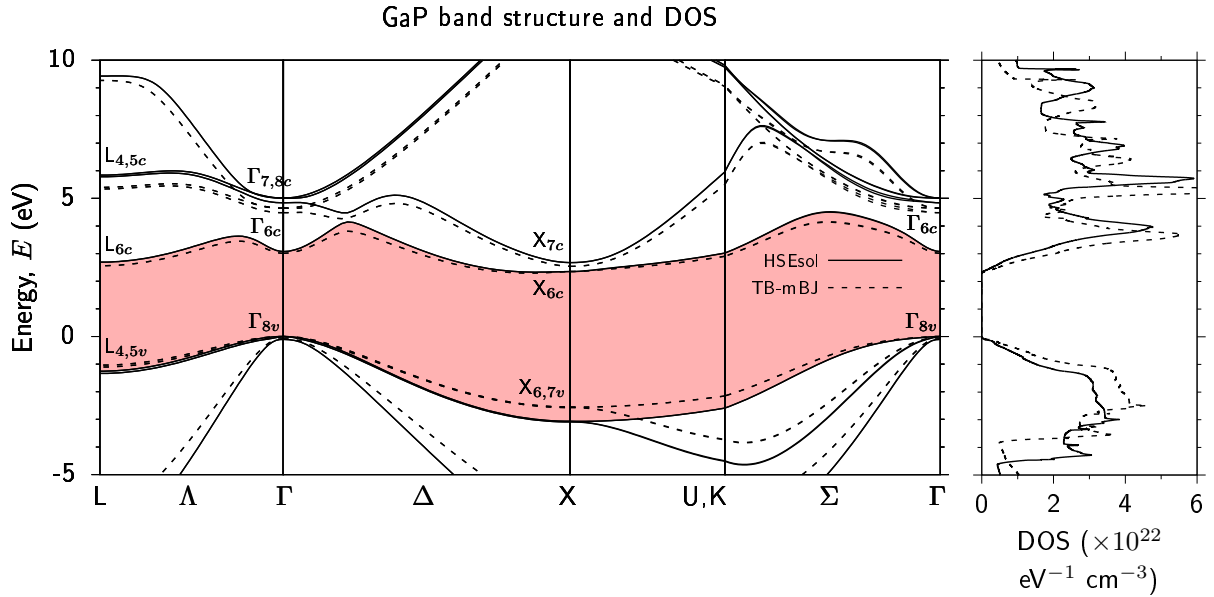
FIGURE 6.2: DFT-calculated band structure (left panel) and density of states (DOS; right panel) of GaP, calculated using the HSEsol (solid lines) and TB-mBJ (dashed lines) XC functionals. The exact exchange mixing in the HSEsol calculation ( \alpha = 0.314 ), and the Becke-Roussel mixing in the TB-mBJ calculation ( c = 1.193 ), were adjusted to fit to the experimental zero-temperature fundamental (indirect) X_{6c} - \Gamma_{8v} band gap of 2.35 eV [44]. The zero of energy is set at the valence band maximum.
