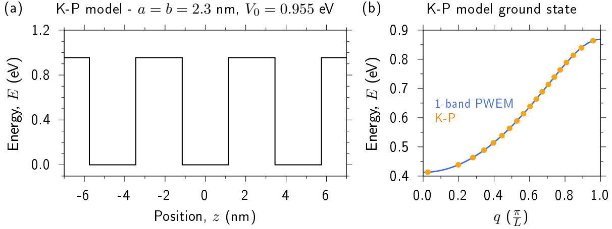
FIGURE 2.1: (a) Potential profile for a Kronig-Penney superlattice having equal well and barrier thicknesses ( a = b = 2.3 nm), and barrier potential energy depth V_0 = 0.955 eV. (b) Solution for the energy dispersion (band structure) of the lowest energy bound states in the superlattice of (a) as a function of wave vector q – obtained using the Kronig-Penney model (filled orange circles) and the 1-band plane wave expansion method (solid blue line).
