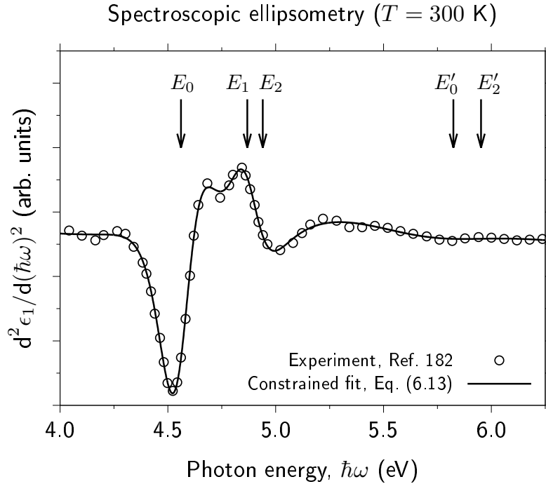
FIGURE 6.4: Second derivative with respect to photon energy \hbar\omega of the real part \epsilon_1 of the dielectric function of AlP, computed from the measured spectroscopic ellipsometry data of Ref. [182] (open circles), and calculated via a constrained fit (solid line) employing Eq. (6.13) with fixed critical point energies E_j ( j = 1, \dots, 5 ; vertical arrows) obtained from the HSEsol-calculated AlP band structure (cf. Fig. 6.1).
