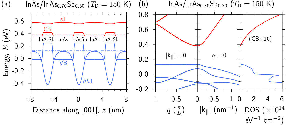
FIGURE 5.3: (a) Calculated CB (red) and VB (blue) offsets, illustrated for three periods of an InAs/InAs 0.70 Sb 0.30 ( x = 30\% ) SBSL with \lambda_{\text{cut}} = 5 \mu\text{m} having respective InAs and InAs 1-x Sb x layer thicknesses t_0 = 3.57 \text{ nm} and t_x = 1.67 \text{ nm} (SL period L = t_0 + t_x = 5.24 \text{ nm} ). The dash-dotted red (blue) line denotes the energy of the lowest energy bound electron state e1 (highest bound hole state hh1 ). The corresponding e1 ( hh1 ) probability density at \mathbf{k}_{\parallel} = q = 0 is shown using a solid red (blue) line, shifted so that the zero of probability density lies at the e1 ( hh1 ) energy. (b) Calculated band structure and density of states (DOS) at temperature T_D = 150 \text{ K} for the SBSL of (a). The left-hand, centre and right-hand panels respectively show the calculated miniband ( q ) dispersion, in-plane ( \mathbf{k}_{\parallel} ) band dispersion and DOS.
