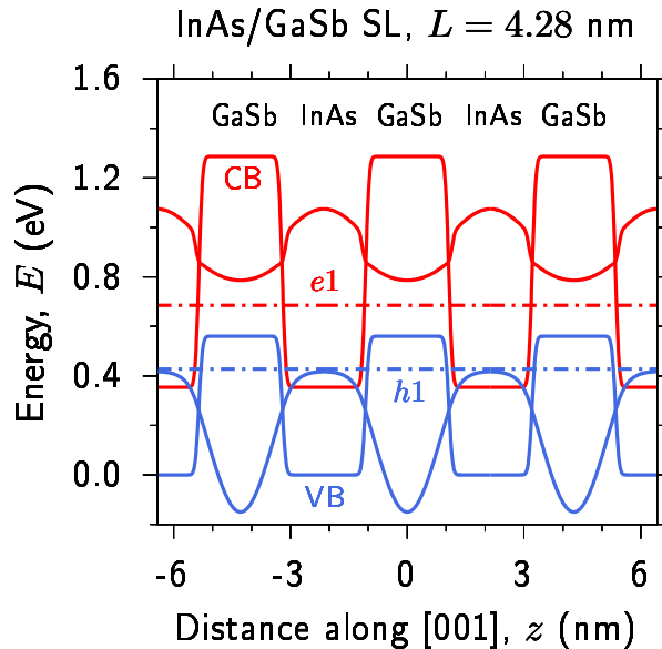
FIGURE 4.3: Calculated CB (solid red line) and VB (solid blue line) offsets, illustrated for three periods of a InAs/GaSb SL having equal InAs and GaSb layer thickness t = 2.14 nm (SL period L = 4.28 nm). The dash-dotted red (blue) line denotes the energy of the lowest energy bound electron state e1 (highest energy bound hole state h1 ). The e1 ( h1 ) probability density is shown using a solid red (blue) line, shifted so that the zero of probability density lies at the e1 ( h1 ) energy.
