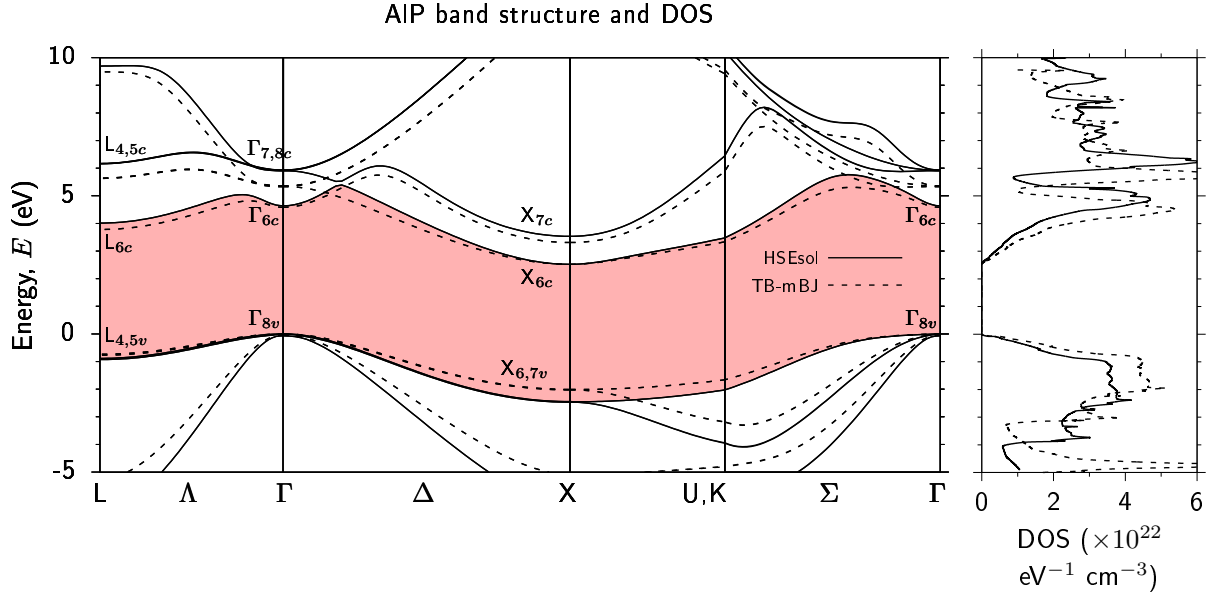
FIGURE 6.1: DFT-calculated band structure (left panel) and density of states (DOS; right panel) of AlP, calculated using the HSEsol (solid lines) and TB-mBJ (dashed lines) XC functionals. The exact exchange mixing in the HSEsol calculation ( \alpha = 0.363 ), and the Becke-Roussel mixing in the TB-mBJ calculation ( c = 1.218 ), were adjusted to fit to the experimental zero-temperature fundamental (indirect) X_{6c} - \Gamma_{8v} band gap of 2.52 eV [44]. The zero of energy is set at the valence band maximum.
