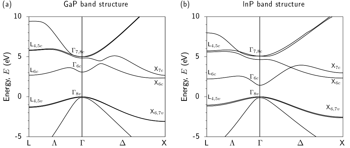
FIGURE 1.3: DFT-calculated band structure for (a) GaP and (b) InP. Calculated using HSEsol exchange-correlation functionals. The exact exchange mixing was adjusted to fit to the experimental zero-temperature fundamental indirect (direct) band gap in GaP (InP), taken from Ref. [44]. The zero of energy is set at the valence band maximum in both (a) and (b). Further details regarding these calculations follow in Chapter 6.
