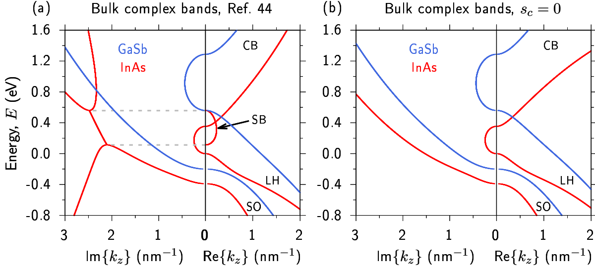
FIGURE 4.1: (a) Complex band structure of bulk InAs (solid red lines) and GaSb (solid blue lines) along [001], using an 8-band \mathbf{k} \cdot \mathbf{p} Hamiltonian with the parameters of Ref. [44]. The arrow highlights the real k_z component of a spurious band (SB) lying close in energy to the InAs CB edge, with the imaginary component of the SB lying in the same energy range in the left-hand panel. (b) As in (a), but using renormalised parameters in which s_c = 0 .
