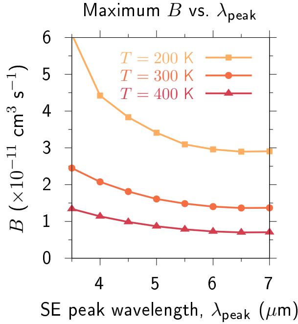
FIGURE 4.8: Maximised radiative recombination coefficient B as a function of emission wavelength \lambda_{\text{peak}} , for temperature T = 200 \text{ K} (closed orange squares), 300 \text{ K} (closed dark orange circles), and 400 \text{ K} (closed red triangles).
