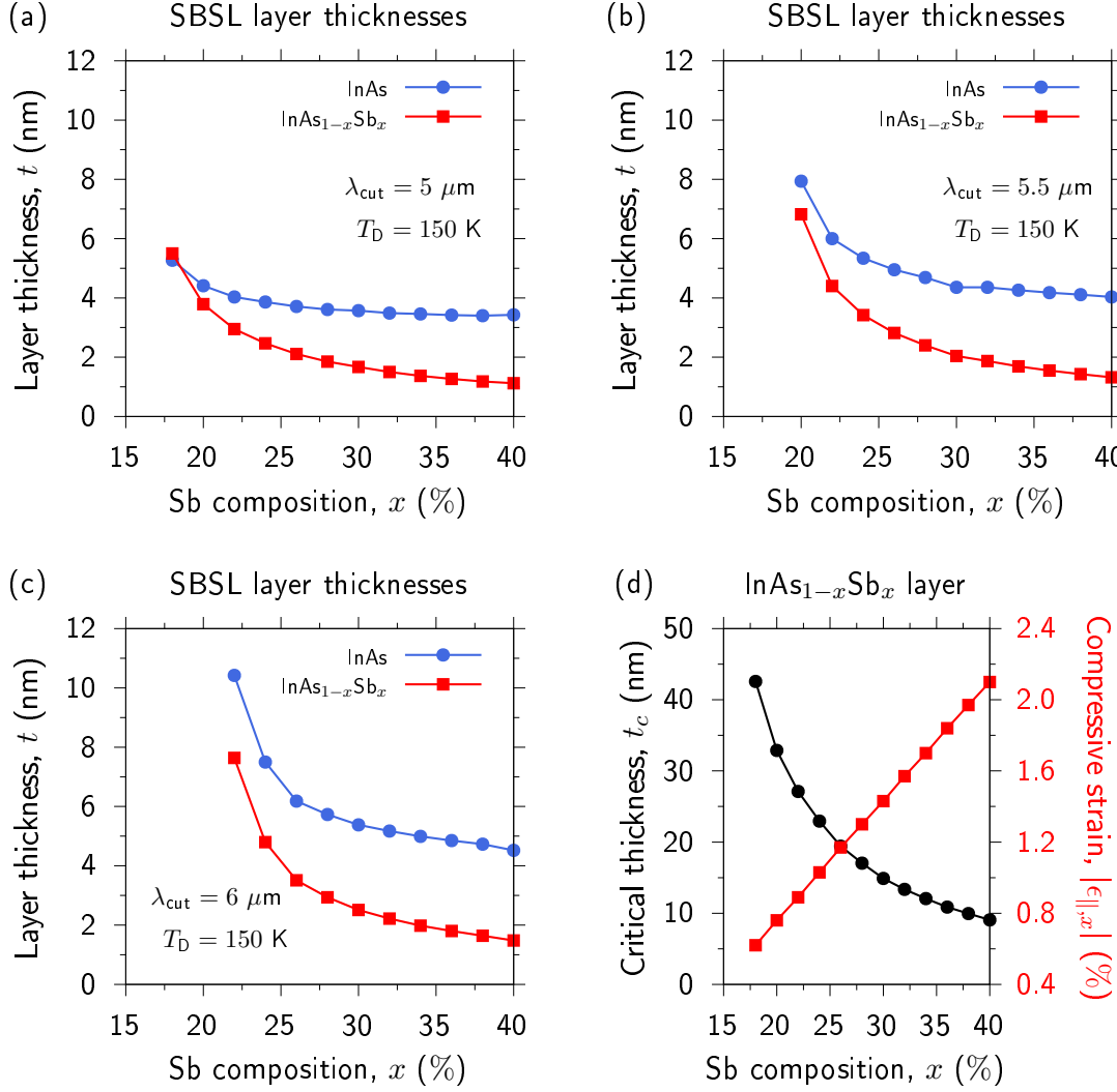
FIGURE 5.2: (a) Calculated \text{InAs} (closed blue circles) and \text{InAs}_{1-x}\text{Sb}_x (closed red squares) layer thicknesses for SBSLs having fixed cut-off wavelength \lambda_{\text{cut}} = 5 \mu\text{m} as a function of Sb composition x . (b) Equivalent to (a) for SBSLs having \lambda_{\text{cut}} = 5.5 \mu\text{m} . (c) Equivalent to (a) for SBSLs having \lambda_{\text{cut}} = 6 \mu\text{m} . (d) Calculated critical thickness t_c (closed black circles and left-hand vertical axis) and compressive in-plane strain \epsilon_{||,x} (closed red squares and right-hand vertical axis) as a function of Sb composition x .
