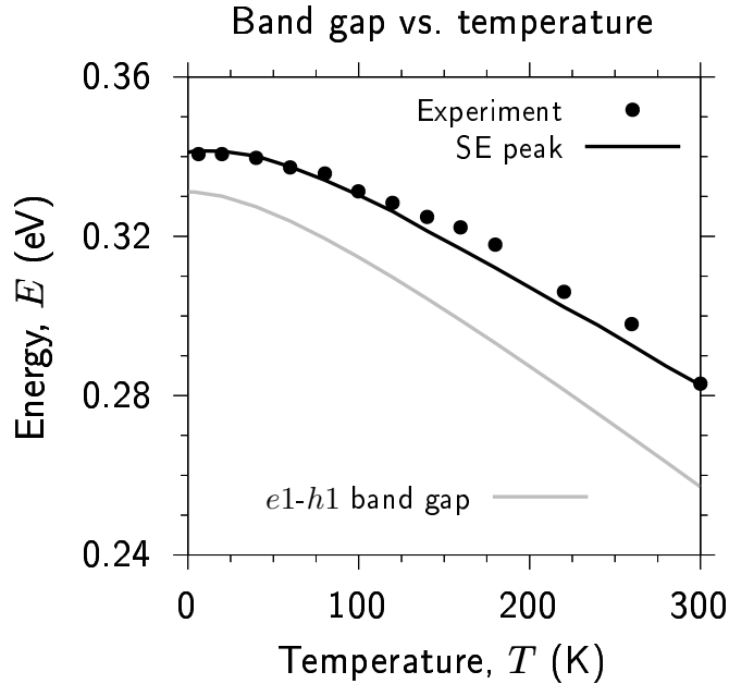
FIGURE 4.2: Theory vs. experiment comparison of the dependence of the emission energy vs. temperature T for an InAs/GaSb SL having equal InAs and GaSb layer thicknesses t = 2.14 nm (SL period L = 2t = 4.28 nm). The solid black line shows the calculated SE peak energy vs. T at injected electron and hole carrier densities n = p = 10^{17} \text{ cm}^{-3} . The solid grey line shows the calculated SL ( e1-h1 ) band gap at \mathbf{k} = 0 . Experimental data (closed black circles) are from Ref. [16].
