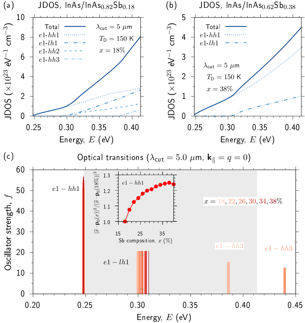
FIGURE 5.6: (a) Calculated JDOS of an InAs/InAs 0.82 Sb 0.18 ( x = 18\% ) SBSL with \lambda_{\text{cut}} = 5 \mu\text{m} , including contributions from all conduction and valence subband pairs (solid blue line). Dotted, dashed and dash-dotted lines show contributions to the JDOS from individual subband pairs, which in this SBSL corresponds to one bound electron state e1 and four bound hole states hh1 , lh1 , hh2 and hh3 (in order of decreasing energy at \mathbf{k}_{\parallel} = q = 0 ). (b) As in (a), but for an InAs/InAs 0.62 Sb 0.38 SBSL supporting two bound hole states hh1 and lh1 . (c) Calculated \mathbf{k}_{\parallel} = q = 0 squared optical (momentum) matrix elements |\hat{x} \cdot \mathbf{p}_0|^2 , scaled as the oscillator strength f vs. inter-band transition energy E for a selection of SBSLs having \lambda_{\text{cut}} = 5 \mu\text{m} and Sb compositions x = 18, 22, 26, 30, 34 and 38\% (darkening red). Shaded region highlights the \hbar\omega = 0.248 - 0.413 \text{ eV} photon energy ( \lambda = 3 - 5 \mu\text{m} wavelength) range used in evaluation of the IQE. Inset: \mathbf{k}_{\parallel} = q = 0 e1-hh1 squared optical matrix elements vs. x for \lambda_{\text{cut}} = 5 \mu\text{m} . The squared optical matrix elements are shown relative to their calculated value at x = 18\% .
