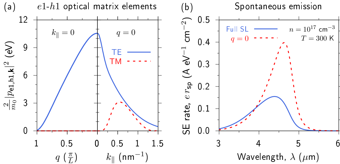
FIGURE 4.5: (a) Calculated TE-polarised (solid blue line) and TM-polarised (dashed red line) squared optical (momentum) matrix elements between the e1 and h1 subbands, as a function of the SL wave vector q (left-hand panel) and in-plane wave vector k_{\parallel} (right-hand panel). (b) Comparison of SE spectra for an InAs/GaSb SL having equal InAs and GaSb layer thicknesses t = 2.14 \text{ nm} (SL period L = 2t = 4.28 \text{ nm} ), calculated at temperature T = 300 \text{ K} and injected carrier density n = 10^{17} \text{ cm}^{-3} , directly using Eq. (4.4) (solid blue line) and via a simplified calculation neglecting miniband dispersion by fixing q = 0 (dashed red line).
