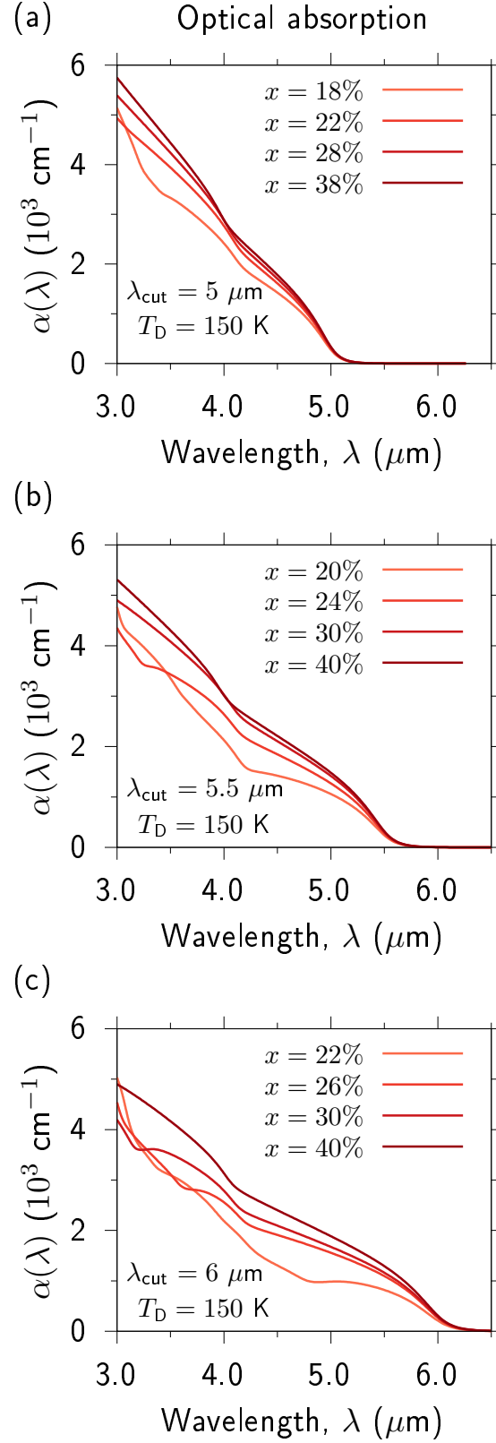
FIGURE 5.4: (a) Calculated optical absorption spectra \alpha(\lambda) for \text{InAs}/\text{InAs}_{1-x}\text{Sb}_x SBSLs with \lambda_{\text{cut}} = 5 \mu\text{m} having Sb compositions x = 18, 22, 28 and 38\% (darkening red lines), at temperature T_D = 150 \text{ K} . (b) and (c) are as in (a), but for respective cut-off wavelengths \lambda_{\text{cut}} = 5.5 and 6 \mu\text{m} , and for Sb compositions x = 20, 24, 30 and 40\% and x = 22, 26, 30 and 40\% .
