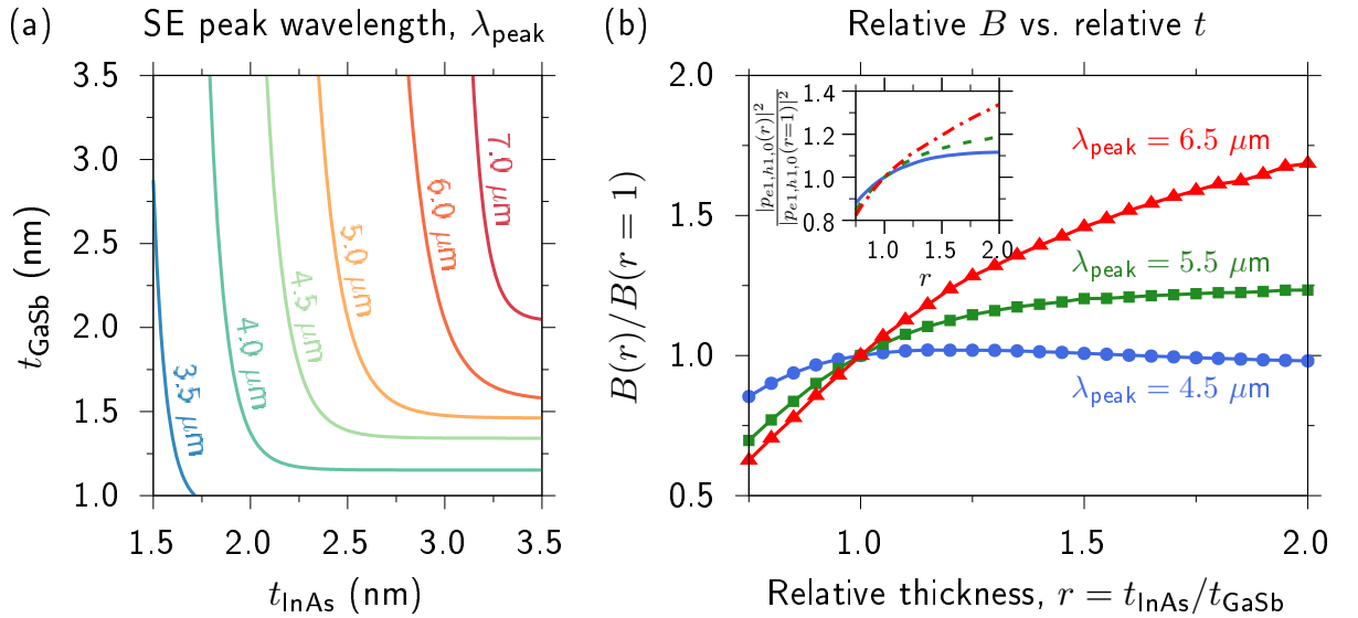
FIGURE 4.7: (a) Contour map denoting combinations of InAs and GaSb layer thicknesses t_{\text{InAs}} and t_{\text{GaSb}} that maintain fixed peak SE wavelengths \lambda_{\text{peak}} ranging from 3.5 \mu\text{m} (blue) to 7 \mu\text{m} (red), at temperature T = 300 \text{ K} and carrier density n = p = 10^{17} \text{ cm}^{-3} . (b) Calculated variation of the radiative recombination coefficient B as a function of the relative InAs and GaSb layer thickness r = t_{\text{InAs}}/t_{\text{GaSb}} , for \lambda_{\text{peak}} = 4.5 \mu\text{m} (closed blue circles), 5.5 \mu\text{m} (closed green squares), and 6.5 \mu\text{m} (closed red triangles). For a given \lambda_{\text{peak}} , B values are shown relative to their calculated value in an equal thickness structure having r = 1 . Inset: relative squared TE-polarised optical matrix element vs. r for the same \lambda_{\text{peak}} as in the main figure.
