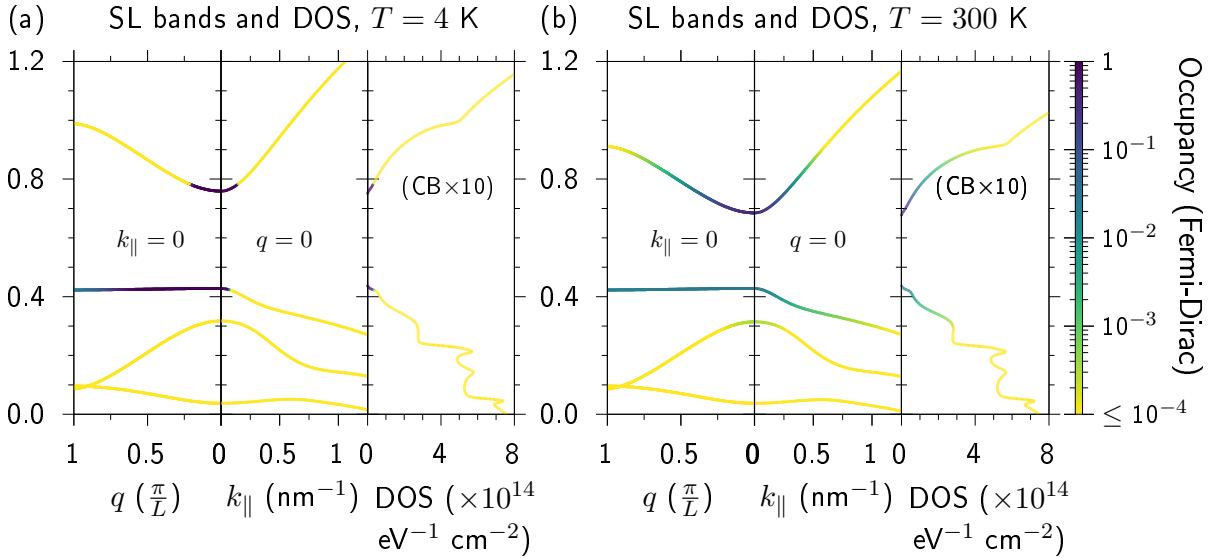
FIGURE 4.4: (a) and (b) Calculated band structure and DOS at temperature (a) T = 4 K, and (b) T = 300 K, for the equal layer thickness SL of Fig. 4.3. The left-hand, centre and right-hand panels in (a) and (b) respectively show the calculated miniband dispersion, in-plane band dispersion and DOS. The CB DOS is scaled \times 10 to enhance visibility. The line colour is weighted by the Fermi-Dirac occupancy, for injected electron and hole carrier densities n = p = 10^{17} \text{ cm}^{-3} .
