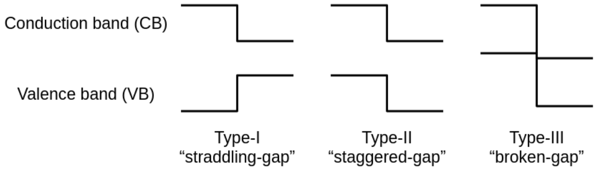
FIGURE 1.2: Illustration of the three types of heterojunction band offsets, in the absence of lattice mismatch. Moving left to right: type-I (“straddling-gap”), type-II (“staggered-gap”) and type-III (“broken-gap”) band alignment.
