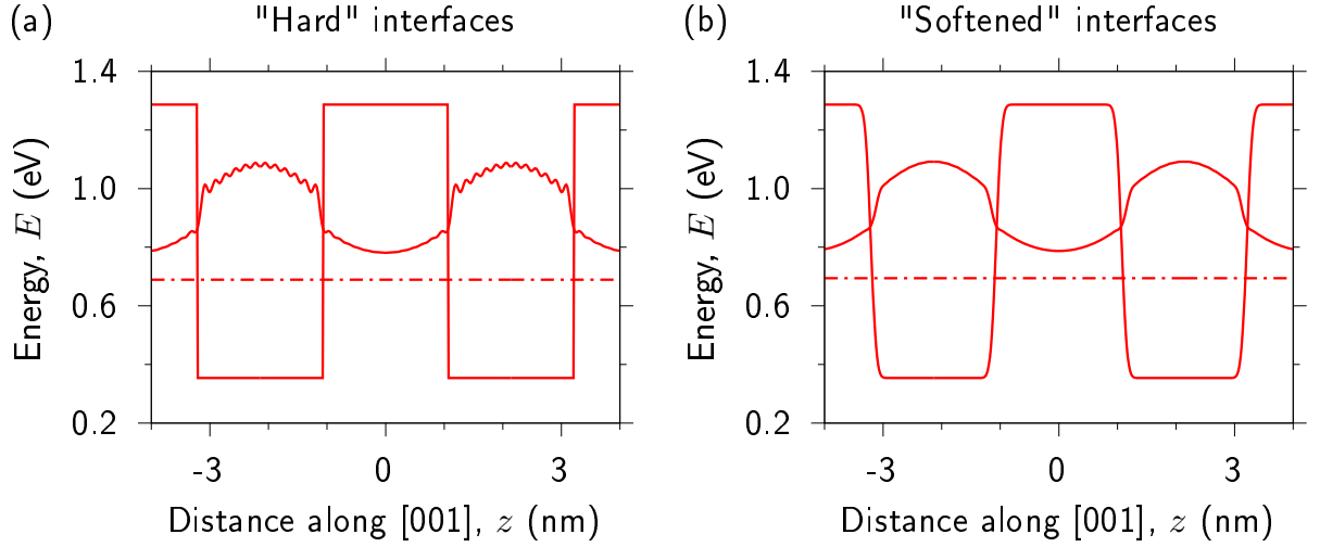
FIGURE B.1: (a) With no interface softening implemented – i.e. “hard” interfaces – calculated conduction band (solid red line) offsets, illustrated for two periods of a InAs/GaSb SL having equal InAs and GaSb layer thickness t = 2.14 nm (SL period L = 4.28 nm), and total number of plane waves 2M + 1 = 51 ( M = 25 ). The dash-dotted red line denotes the energy of the lowest energy bound electron state e1 . The e1 probability density is shown using a solid red line, shifted so that the zero of probability density lies at the e1 energy. (b) Same as in (a) with interface softening implemented – i.e. “softened” interfaces.
