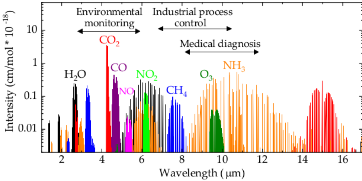
FIGURE 1.1: Mid-infrared absorption spectra of selected molecules with their relative intensities. Water ( \text{H}_2\text{O} ), carbon dioxide ( \text{CO}_2 ), carbon monoxide ( \text{CO} ), nitric oxide ( \text{NO} ), nitrogen dioxide ( \text{NO}_2 ), methane ( \text{CH}_4 ), ozone ( \text{O}_3 ), ammonia ( \text{NH}_3 ). Figure reprinted from Popa et al., Sensors 19 , 2076 (2019). Copyright 2019 MDPI.
