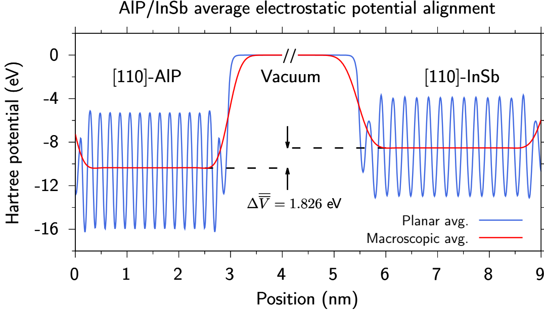
FIGURE 6.5: Schematic illustration of the alignment of the average electrostatic (Hartree) potential \bar{V} between [110]-oriented AlP (left) and InSb (right) slabs. Solid blue and red lines respectively show the planar and macroscopic averages \bar{V}(z) and \bar{\bar{V}} calculated using Eqs. (6.30) and (6.31). The vacuum energy is aligned in each slab, shown here by setting the zero of energy at the vacuum level, allowing extraction of \Delta\bar{\bar{V}} between the two materials.
