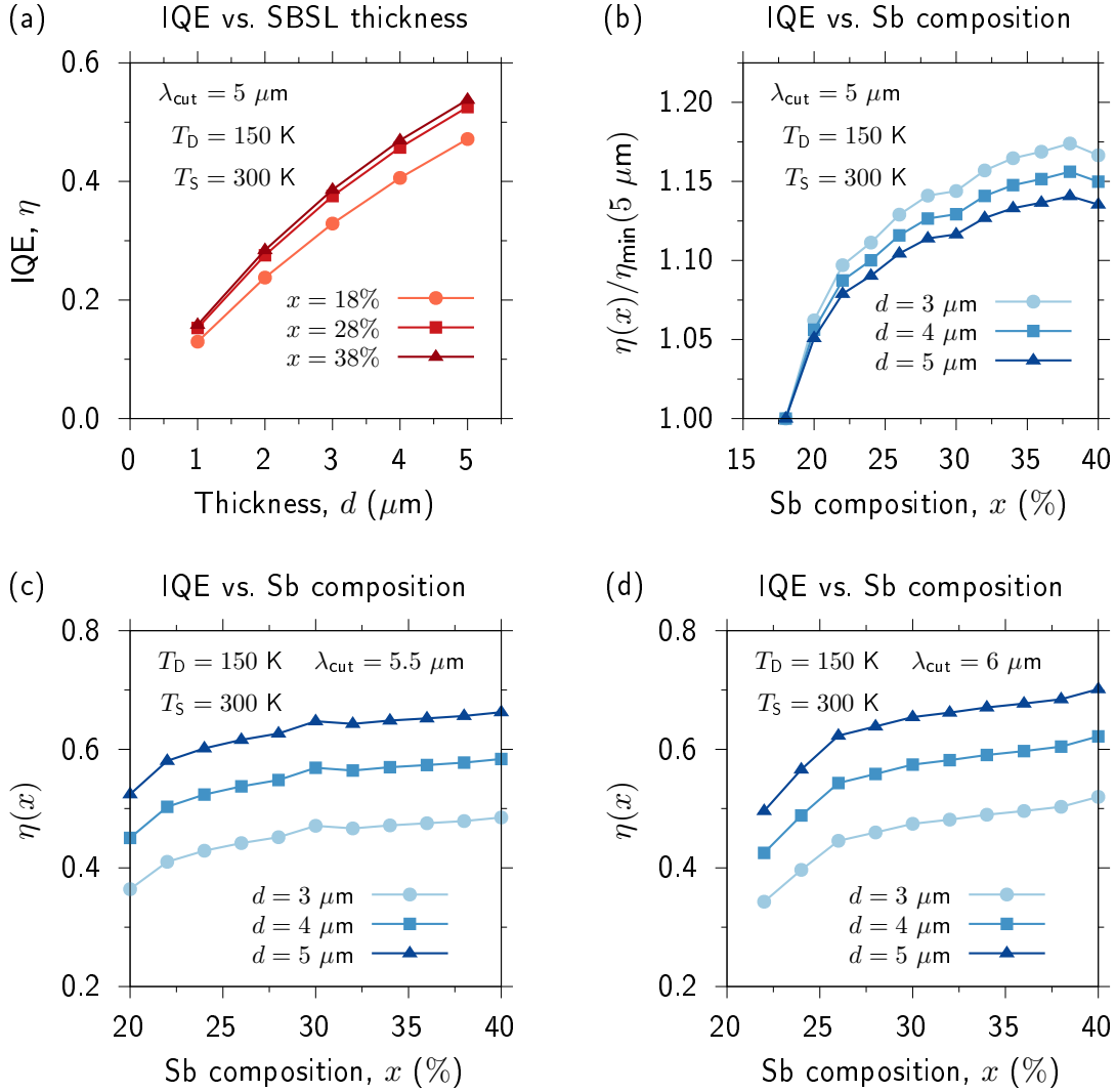
FIGURE 5.5: (a) Calculated IQE \eta vs. total SBSL absorber thickness d for InAs/InAs 1-x Sb x SBSLs having \lambda_{\text{cut}} = 5 \mu\text{m} , for Sb compositions x = 18\% (closed orange circles), 28\% (closed red squares) and 38\% (closed dark red triangles), calculated assuming detector operating temperature T_D = 150 \text{ K} for the absorption of 3 - 5 \mu\text{m} wavelength radiation emitted by a blackbody source at temperature T_S = 300 \text{ K} . (b) Calculated IQE \eta vs. Sb composition x for SBSLs having \lambda_{\text{cut}} = 5 \mu\text{m} for absorber thicknesses d = 3 \mu\text{m} (closed light blue circles), 4 \mu\text{m} (closed blue squares) and 5 \mu\text{m} (closed dark blue triangles), with T_D = 150 \text{ K} and T_S = 300 \text{ K} . In each case the IQE is shown relative to its calculated value at x = 18\% . (c) Calculated IQE \eta vs. Sb composition x for SBSLs having \lambda_{\text{cut}} = 5.5 \mu\text{m} for absorber thicknesses d = 3 \mu\text{m} (closed light blue circles), 4 \mu\text{m} (closed blue squares) and 5 \mu\text{m} (closed dark blue triangles), with T_D = 150 \text{ K} and T_S = 300 \text{ K} . (d) Equivalent to (c) for SBSLs having \lambda_{\text{cut}} = 6 \mu\text{m} . In each case the IQE is calculated with \hbar\omega_{\text{min}} = 0.248 \text{ eV} and \hbar\omega_{\text{max}} = 0.413 \text{ eV}
