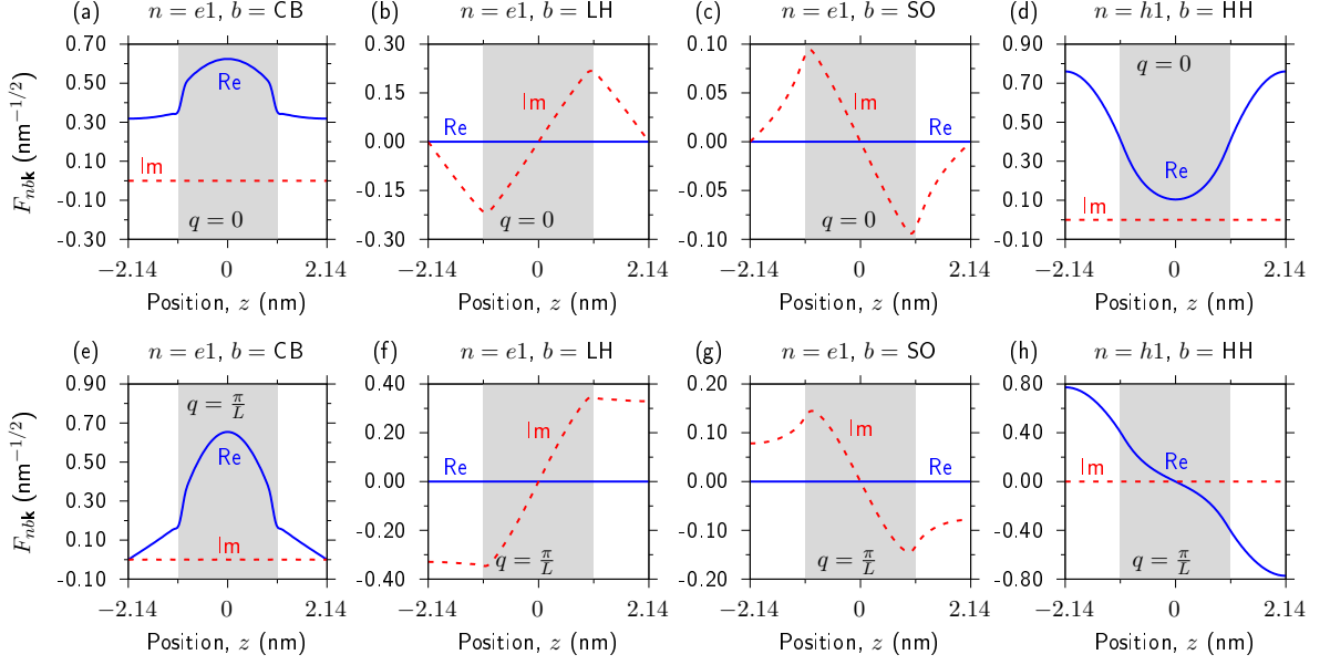
FIGURE A.1: Top row: real (solid blue lines) and imaginary (dashed red lines) parts of the q = 0 envelope function Bloch components F_{nb\mathbf{k}}(z) for the \mathbf{k}_{\parallel} = 0 e1 and h1 eigenstates of the exemplar equal layer thickness InAs/GaSb SL considered in Sec. 4.3 (having SL period L = 2t = 4.28 nm). (a) CB component of e1 , (b) LH component of e1 , (c) SO component of e1 , and (d) HH component of h1 . Bottom row: as in the top row, but for q = \pi/L . Shaded (unshaded) regions denote the electron-confining InAs (hole-confining GaSb) layers.
