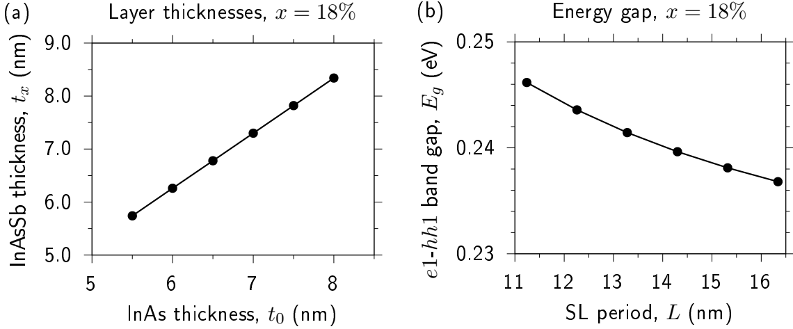
FIGURE 5.1: (a) Computed InAs 0.82 Sb 0.18 layer thicknesses t_x as a function of InAs layer thicknesses t_0 , specifying identified InAs/InAs 0.82 Sb 0.18 ( x = 18\% ) SBSLs computed via Eq. (5.3). (b) Calculated e1-hh1 energy gap E_g as a function of SL period L of the SBSLs detailed in (a).
