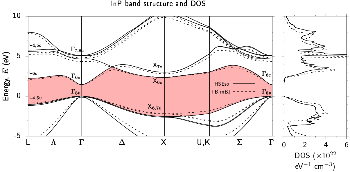
FIGURE 6.3: DFT-calculated band structure (left panel) and density of states (DOS; right panel) of InP, calculated using the HSEsol (solid lines) and TB-mBJ (dashed lines) XC functionals. The exact exchange mixing in the HSEsol calculation ( \alpha = 0.273 ), and the Becke-Roussel mixing in the TB-mBJ calculation ( c = 1.166 ), were adjusted to fit to the experimental zero-temperature fundamental (direct) \Gamma_{6c} - \Gamma_{8v} band gap of 1.424 eV [44]. The zero of energy is set at the valence band maximum.
