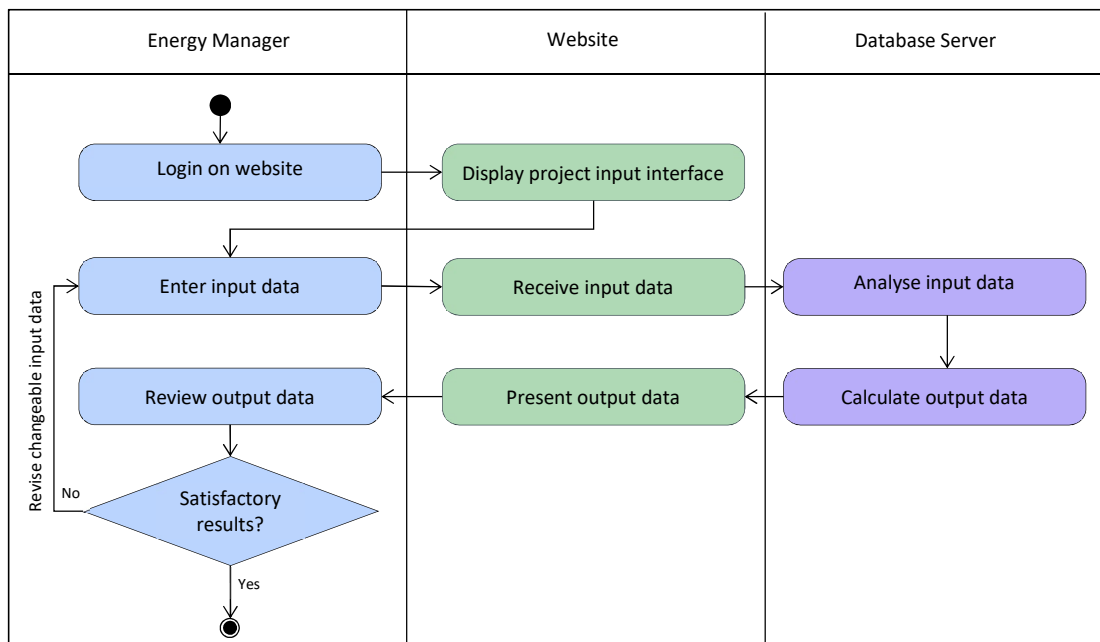
Figure 6.3: Activity diagram
