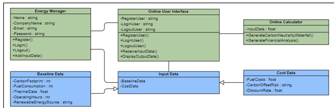
Figure 5.2: Class diagram
