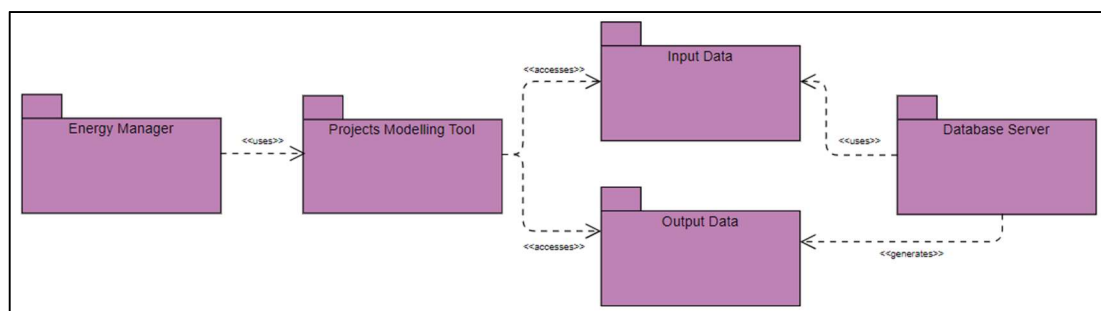
Figure 6.1: Package diagram
