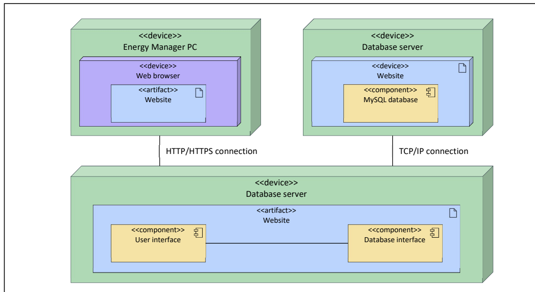
Figure 5.4: Deployment diagram
