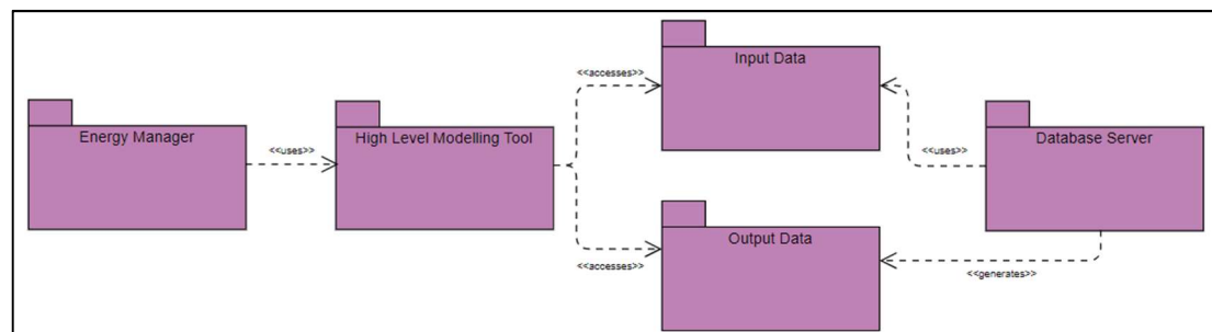
Figure 5.3: Package diagram
