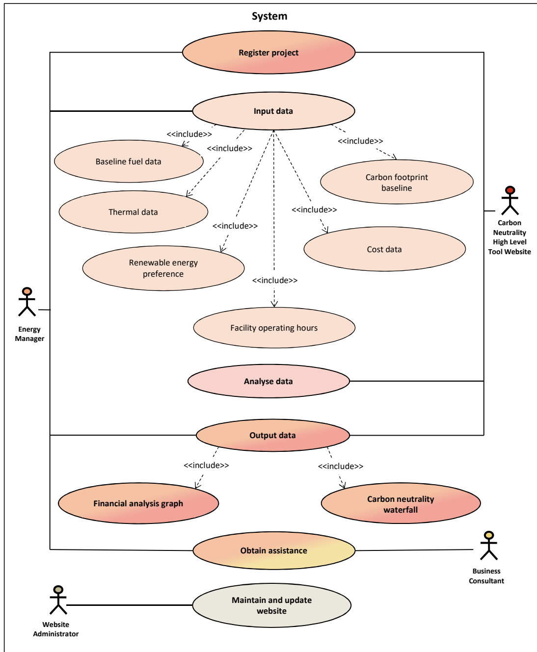
Figure 5.6: Use Case diagram
