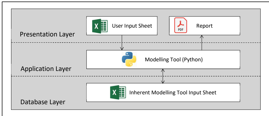
Figure 5.1: Modelling tool architecture diagram
