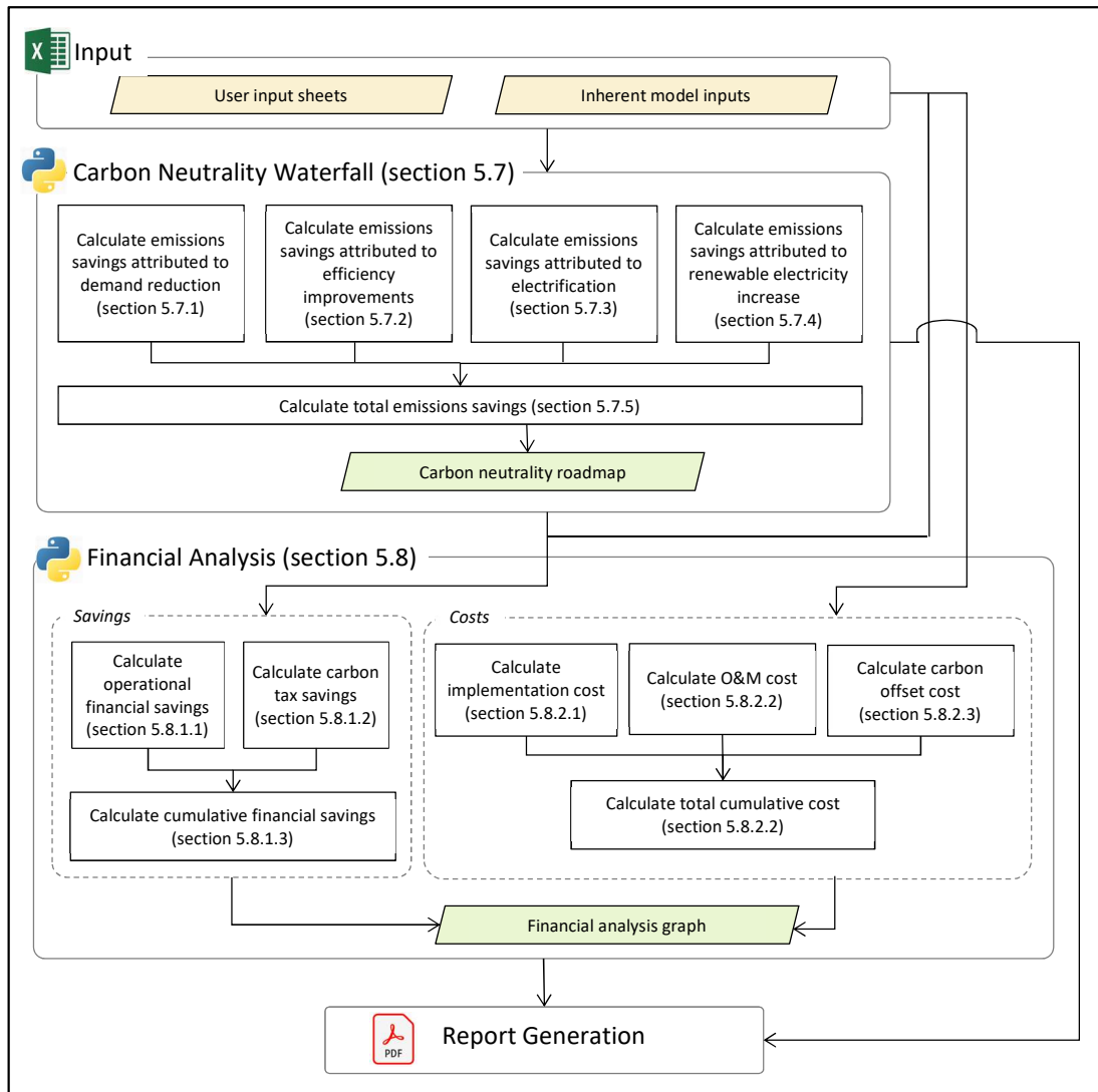
Figure 5.10: Flowchart of modelling methodology – High Level modelling tool
