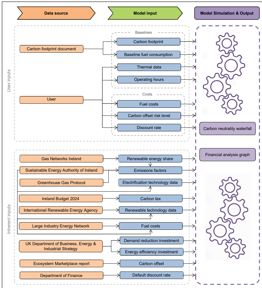
Figure 5.8: Model description – High Level Modelling Tool
