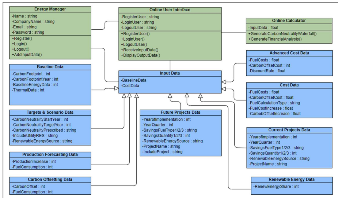
Figure 6.2: Class diagram
