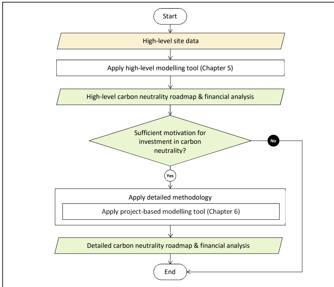
Figure 4.1: High-level methodology
