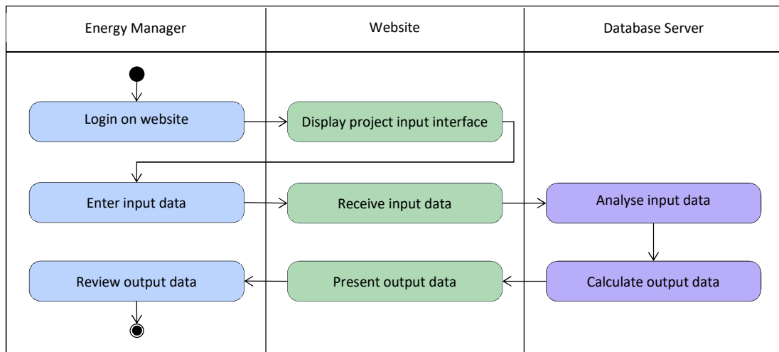
Figure 5.5: Activity diagram
