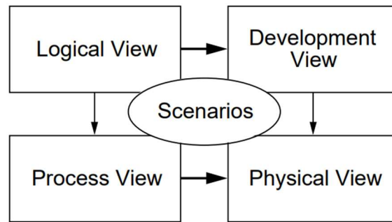
Figure 2.12: 4+1 View Model [137]
