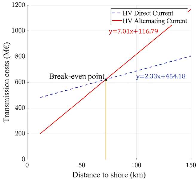
Fig. 3. Electrical infrastructure costs (M€) for HVDC and HVAC. The break-even point is estimated at \sim 72 km.
