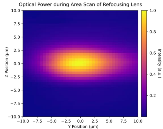
Fig. 6: Optical power distribution in the PD of the PIC while scanning the refocusing lens in Y and Z axes. See Fig. 1 for the orientation of Y and Z axes.
