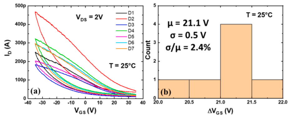
Fig. 5. (a) I_D - V_{GS} curves at V_{DS} = 2\text{V} after stabilization with applying V_{GS} = 35\text{V} and (b) histogram of the hysteresis-induced \Delta V_{GS} shift across seven devices at 25^\circ\text{C} .
