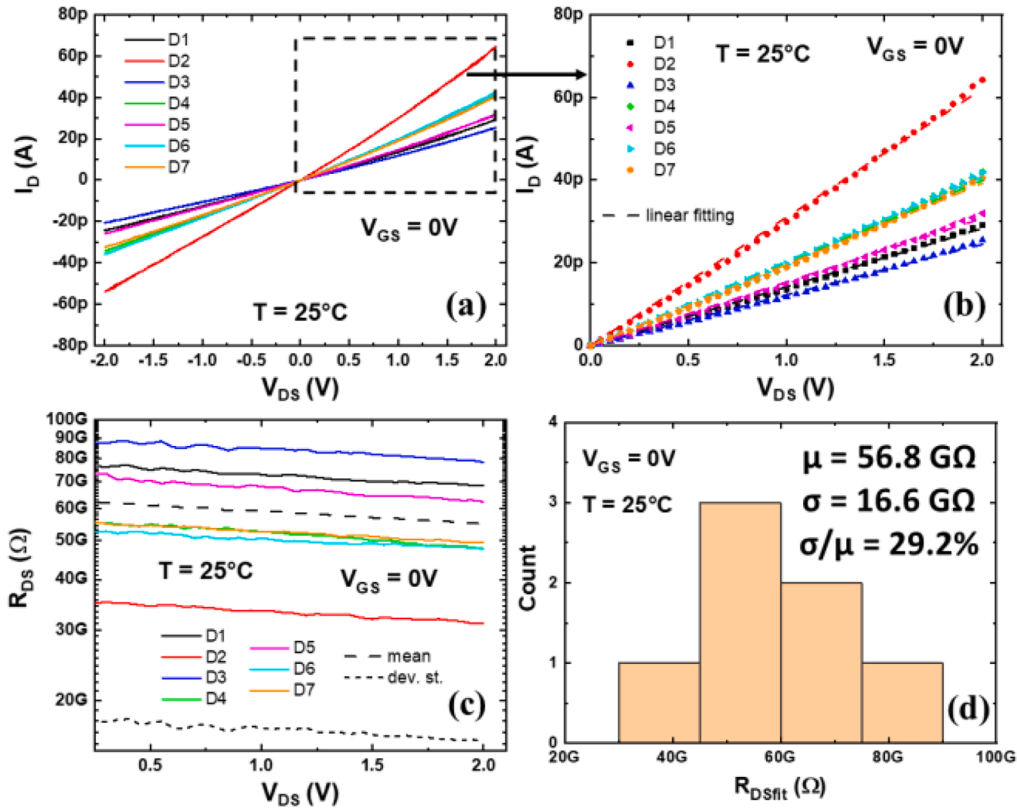
Fig. 6. Output characteristics of seven devices at 25^\circ\text{C} and zero- V_{GS} without any initial stabilization: (a) I_D - V_{DS} curves, (b) detail of I_D - V_{DS} curves for V_{DS} between 0 V and 2 V along with linear fitting, (c) R_{DS} versus V_{DS} , (d) histogram of the fitting R_{DS} , i.e., R_{DSfit} , as extracted from the slope of linear fitting shown in (b).
