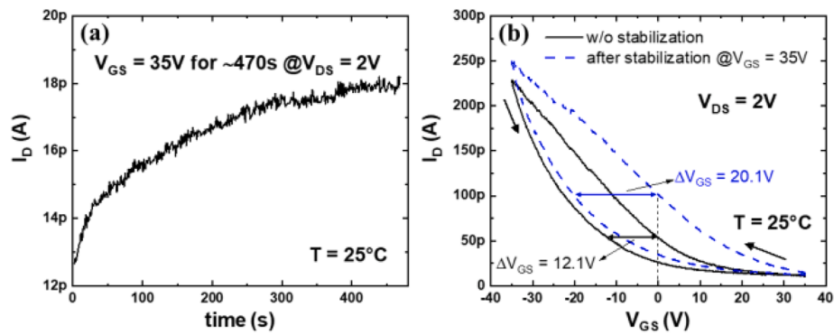
Fig. 4. (a) Time evolution of I_D during stabilization with V_{GS} = 35\text{V} and V_{DS} = 2\text{V} for about 470 s and (b) I_D - V_{GS} curves at V_{DS} = 2\text{V} obtained without and with stabilization for one typical device at 25^\circ\text{C} .
