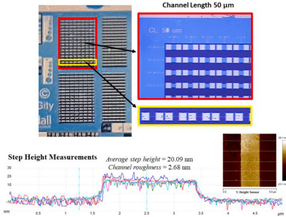
Fig. 3. Sample photo (top) and AFM analysis of a typical device (bottom).
