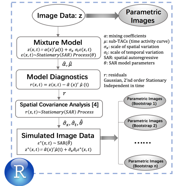
Fig. 2: Model-based Bootstrapping of Dynamic PET
