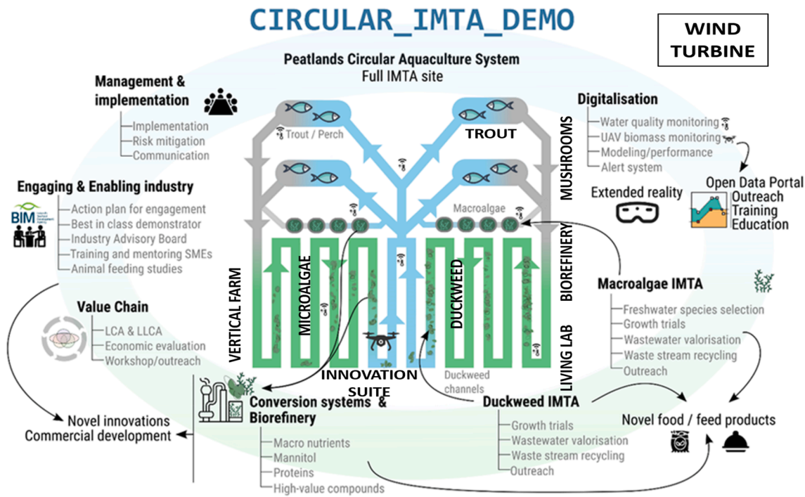
Fig. 2. Schematic of IMTA process for resilient foods in Irish peatlands.
