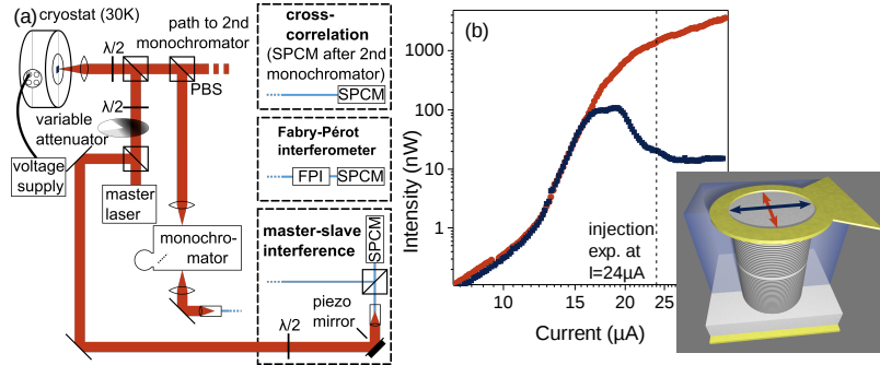
Fig. 1. (a) Experimental setup: The master laser is optically injected in the electrically driven micropillar laser. After spectral filtering using a monochromator, the micropillar emission is analyzed by either CCD, a Fabry-Pérot interferometer, a fiber-coupled cross-correlation configuration, or by interference measurements of master and microlaser emission. (b) Input-output characteristics of both micropillar modes. The SM (red) shows the typical s-shaped behavior of high- \beta microlasers while the WM (dark blue) first increases after threshold and reaches a maximum around 20 \mu\text{A} before it decreases in intensity. Inset: Schematic view of an electrically driven QD-micropillar laser. The polarization of the two orthogonal fundamental micropillar modes are indicated by the red and blue arrows.
