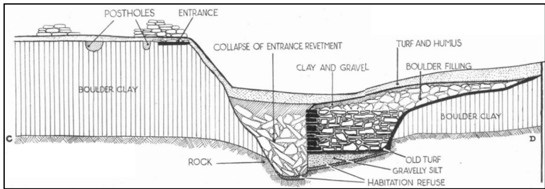
Figure CO.22: Section through the entrance of the fort showing the midden Habitation Refuse (O'Kelly 1952, Plate VIII).
