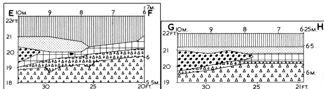
Figure DU.6: Left: East/west section through north-western trenches. Right: East/west section through southwest trenches (Mitchell 1952, Fig. 4).
