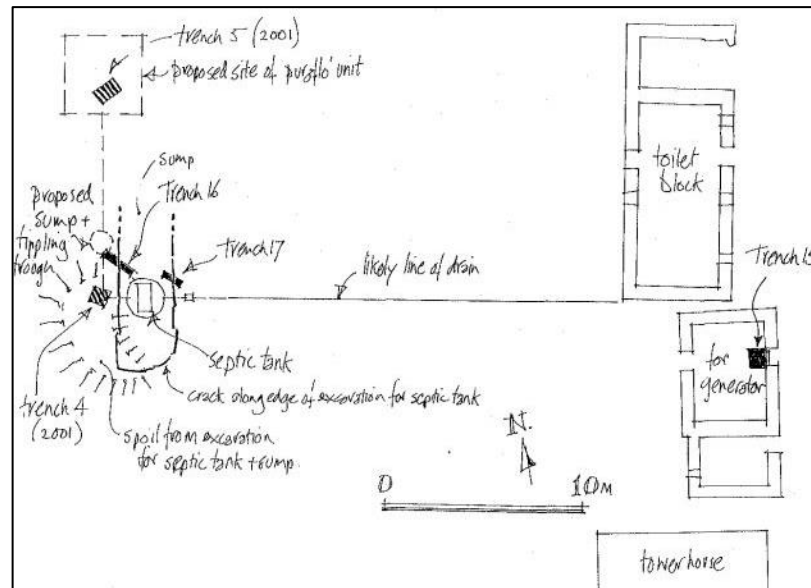
Figure CE.31: Plan of trenches 15-17 (Pollock 2002b, 2).
