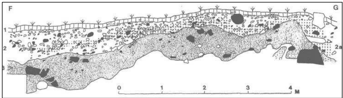
Figure AN.7: Section drawing of the exposed cliff face (Simpson et al. 1993, 118)
