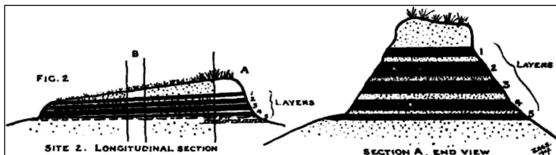
Figure AN.13: Sections of the site as investigated by Davison (Davison et al. 1927, 280).
