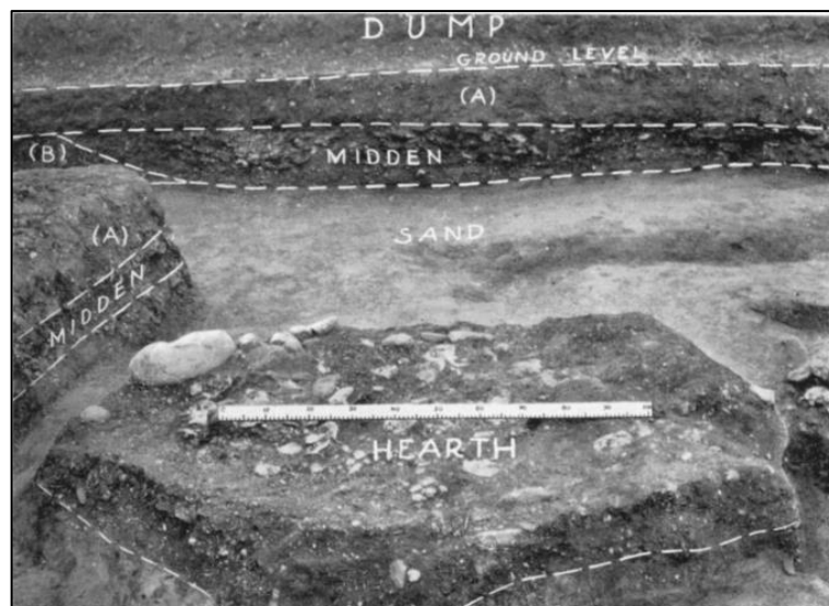
Figure DW.2: Stratigraphy in Trench C showing topsoil (A), Raised Beach (B), and the midden (Movius et al. 1940, 122).
