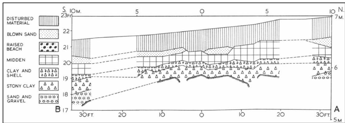
Figure DU.4: North/south stratigraphy of the site with legend (Mitchell 1952, Fig. 4).
