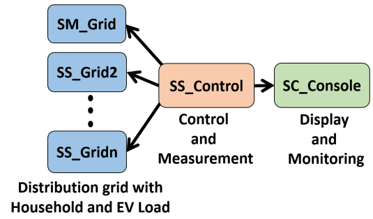
Figure 6: An overview of modelling a test system into several subsystems in RT-LAB Platform.
