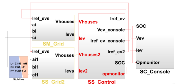
Figure 7: High-level system view of the model.
