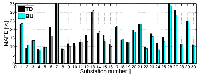
Fig. 15: Summary of 24 hour ahead forecasting errors at secondary substations with 20% EV penetration.
