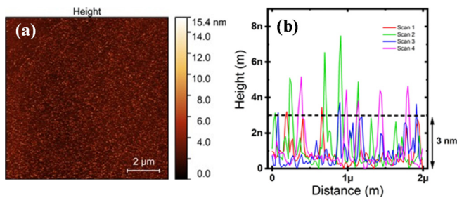
FIG. 2. (a) Representative 10 \times 10 \mu\text{m}^2 scan cross-sectional AFM image of \text{WS}_2 pre-device processing. (b) Graph of 4 (of 20) line profiles from (a) with a length of 2 \mu\text{m} .
