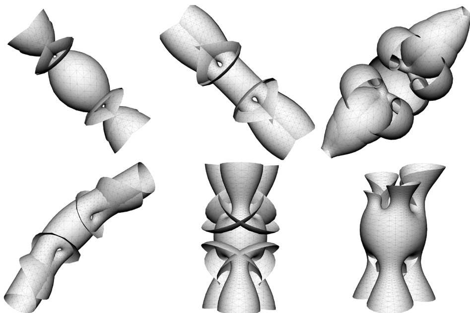
Figure 1. Parts of CMC cylinders with two irregular ends. Each cylinder can be thought of as a surface with a Delaunay centerpiece of one period and two irregular ends. In the first row, 2-legged irregular surfaces emerge from a Delaunay unduloid, cylinder and nodoid. The third surface is cut away to show the internal nodoidal structure. In the second row, the first two surfaces have 1-legged and 3-legged irregular ends respectively. For the first five, f(z) = a + b(z^n + z^{-n}) with (n, a, b) respectively
