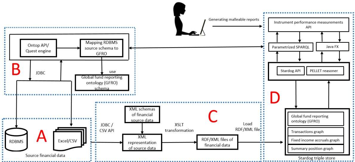
Figure 1: Data Management Framework Components
