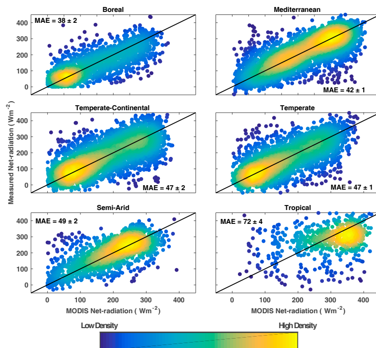
Figure 5. Comparison between daytime MODIS and measured net-radiation in six different climate types. MAE denotes mean absolute error in \text{W} \cdot \text{m}^{-2} .
