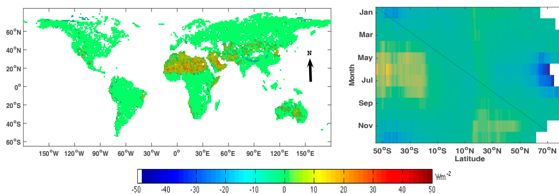
Figure 9. Comparison of MODIS net-radiation with corresponding estimates from CERES: ( left ) the difference between mean daily net-radiation from MODIS and CERES; and ( right ) (Hovmoller diagram) the monthly latitudinal distribution of difference between mean net-radiation from MODIS and CERES.
