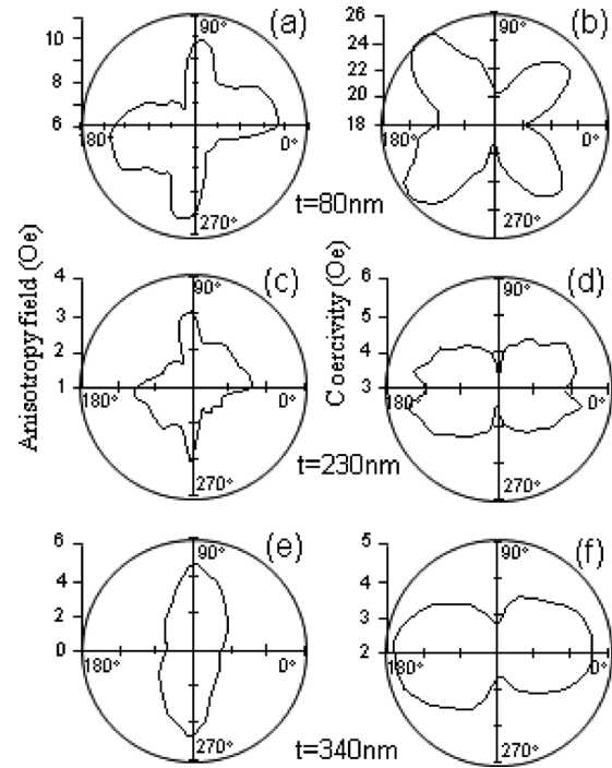
FIG. 3. Angle dependence of anisotropy field (left column) and coercivity (right column) taken from films with 220 nm modulation amplitude and different thicknesses as indicated.
