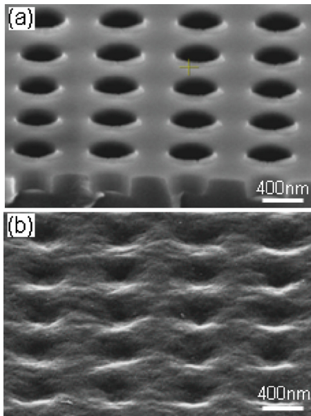
FIG. 1. (Color online) SEM images of the array of nanoholes in PMMA (a) and plated \text{Ni}_{43}\text{Fe}_{55} film with modulated surfaces (b).
