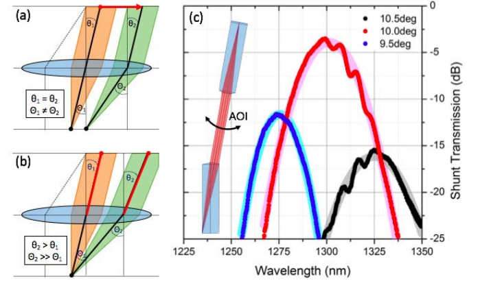
Fig. 5. (a) Schematic showing how two offset collimated beams incident on the \mu\text{Lens} array, with the same external AOI ( \theta_1 = \theta_2 ), converge at the focal-plane of the PIC surface with different internal angles of incidence ( \Theta_1 \neq \Theta_2 ). (b) Schematic showing how two collimated beams incident on the \mu\text{Lens} array, with different external AOI ( \theta_2 > \theta_1 ), firstly require a displacement offset to ensure focus at the same point on the focal plane (i.e., at the grating-coupler), and secondly converge at PIC surface with significantly different internal AOI ( \Theta_2 \gg \Theta_1 ). (c) The Fiber-to-Fiber shunt transmission spectra of the \mu\text{Lens} Fiber-to-PIC as a function of small changes to the external AOI.
