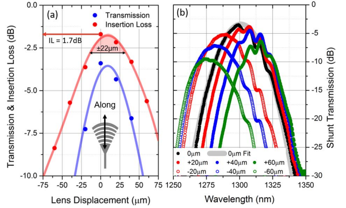
Fig. 4. (a) The Fiber-to-Fiber transmission (and the corresponding insertion-loss) through the optical-shunt at 1300nm as a function of the \mu\text{Lens} -FA displacement. (b) Shunt transmission spectra. Note that the central wavelength of these spectra does shift as the \mu\text{Lens} -FA is displaced, indicating a change in the AOI of the light incident on the grating-coupler.
