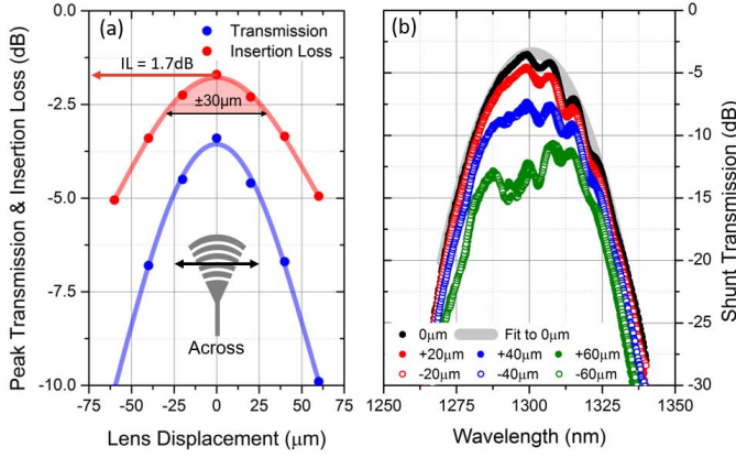
Fig. 3. (a) The peak Fiber-to-Fiber transmission through the optical-shunt (and the corresponding insertion-loss) as a function of the \mu\text{Lens} -FA displacement. The peak transmission is determined by a parabolic fit to the shunt transmission spectra shown in (b). Note that the central wavelength of these spectra does not shift significantly as the \mu\text{Lens} -FA is displaced.
