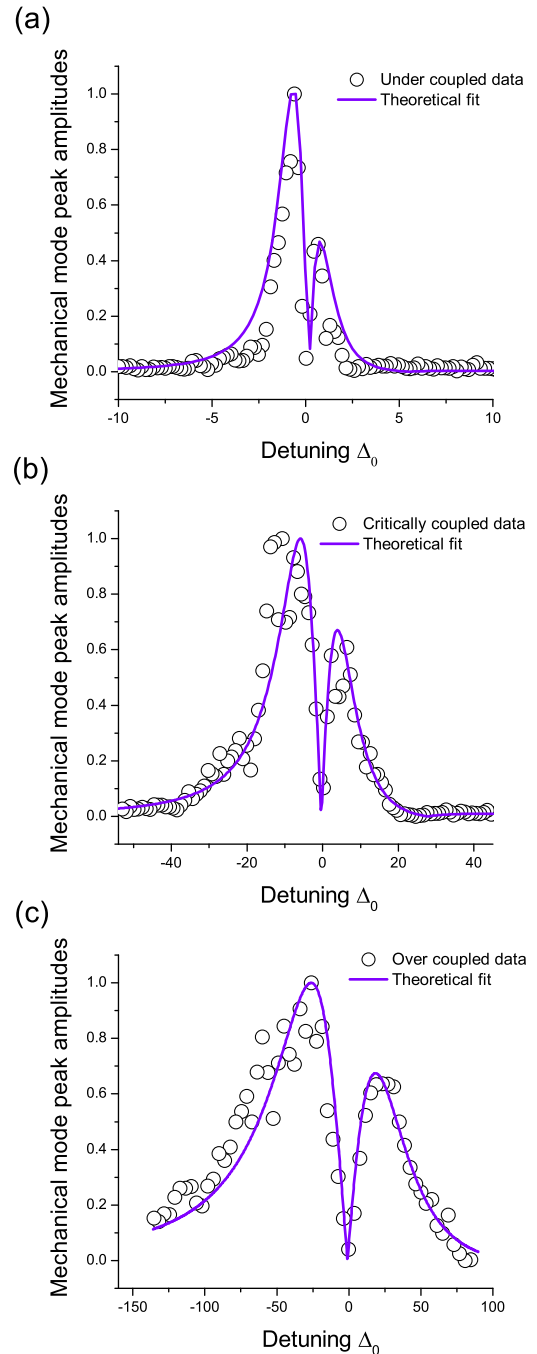
FIG. 3. Transduction response profiles. (a) undercoupled ( d_0 = 0.38 \mu\text{m} ), (b) critically coupled ( d_0 = 0.21 \mu\text{m} ), and (c) overcoupled ( d_0 = 0.12 \mu\text{m} ). Solid lines are theoretical fits. The experiments were repeated four times and data averages are presented.
