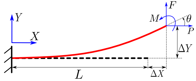
Figure 1. A simple beam flexure subject to combined force and moment loads.
