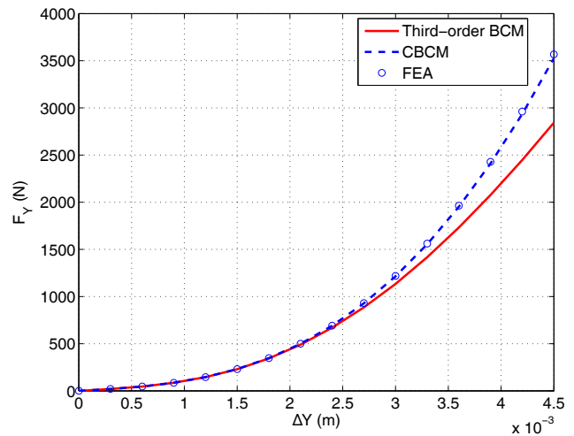
Figure 4. Comparison of the load-displacement relationship of the compliant parallelogram mechanism.
