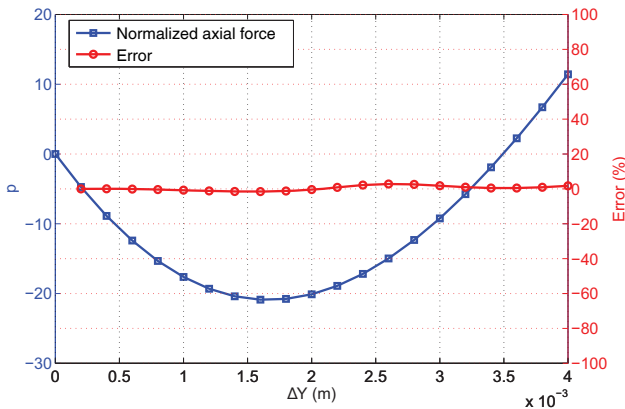
Figure 12. Comparison of normalized axial force and error of Example II.
