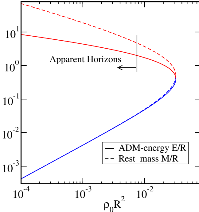
FIG. 1 (color online). ADM-energy and rest mass as function of \rho_0 R^2 for the constant-density star of Sec. III A.
