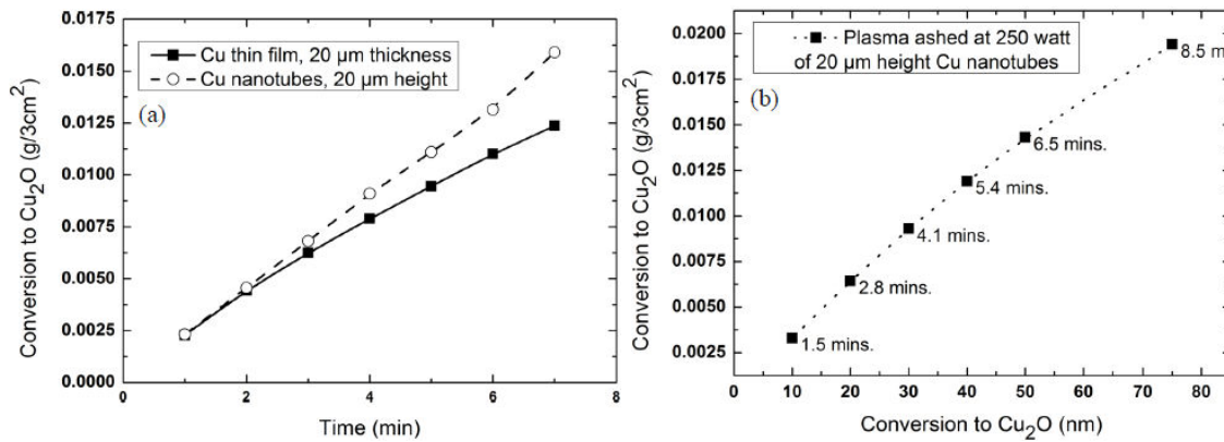
Figure 5. Conversion rate plots for Cu to \text{Cu}_2\text{O} by oxygen plasma treatment, (a) time related plot and (b) correlation plot with the wall thickness of Cu nanotubes.
