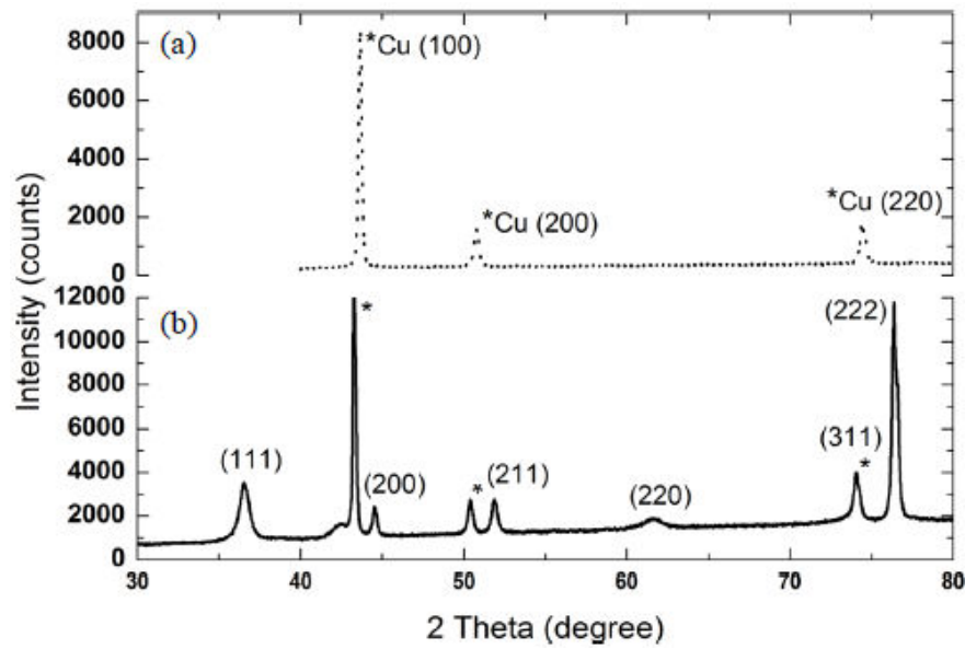
Figure 4. XRD patterns of (a) Cu nanotubes after removal of the AAO template and (b) \text{Cu}_2\text{O} nanotubes.
