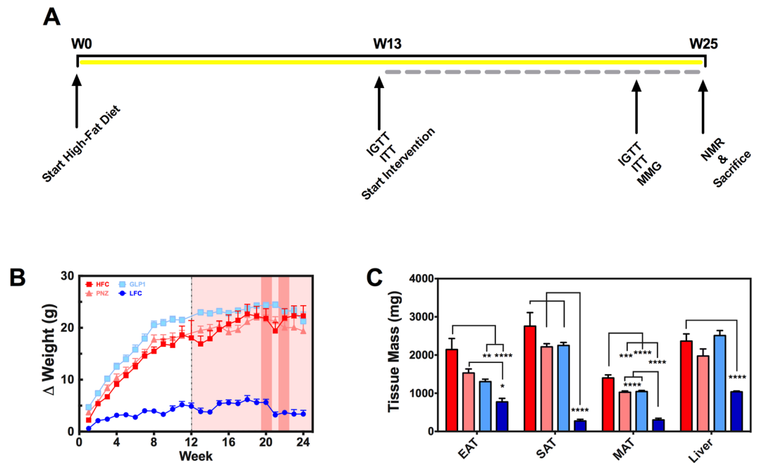
Figure 3. Lactobacillus paracasei Attenuates Mouse Adiposity Independently of GLP-1-Expression. Experiment II: (A) Mouse trial design and procedures detailed above, with high-fat diet represented by yellow bar and intervention by broken grey bar. (B) Delta change in body weights over the pre-feeding (white background) and intervention (red background) periods for HFC (dark red; n = 13 ), PNZ (light red; n = 14 ), GLP1 (light blue; n = 14 ) and LFC (dark blue; n = 14 ). Tall dark red boxes represent metabolic test weeks (IPGTT/ITT and mixed meal gavage, respectively). (C) Epididymal (EAT), subcutaneous (SAT) and mesenteric adipose tissue (MAT), and liver tissue weights are also depicted. Data was analysed by one-way ANOVA with Bonferroni correction, significant differences are represented by * ( p < 0.05 ), ** ( p < 0.01 ), *** ( p < 0.001 ), **** ( p < 0.0001 ), where the asterisks are coloured according to the group with which a significant difference was recorded. Plots depict replicates with mean and SEM.
