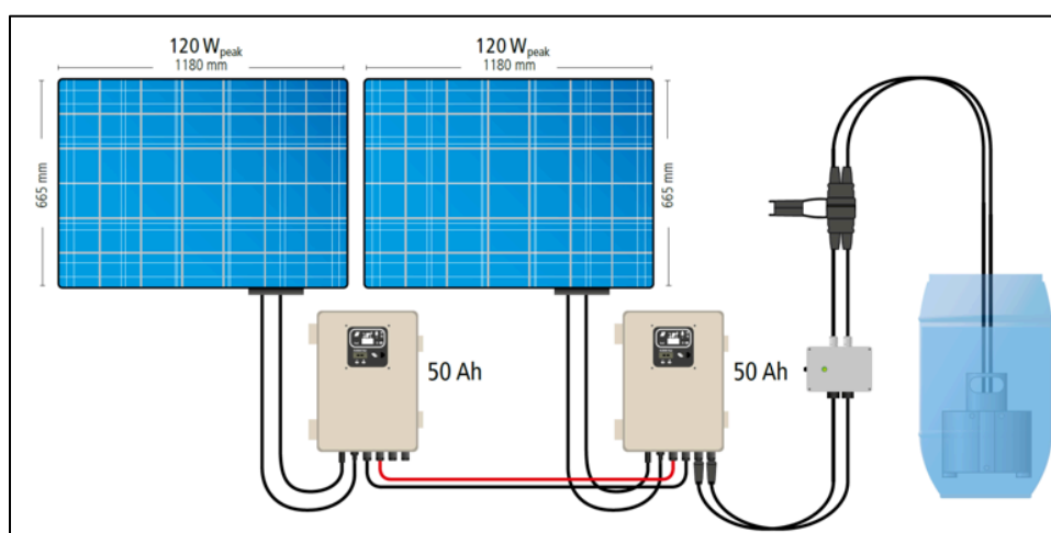
Figure 16. WATA solar kits. ( WATA Webpage ).
