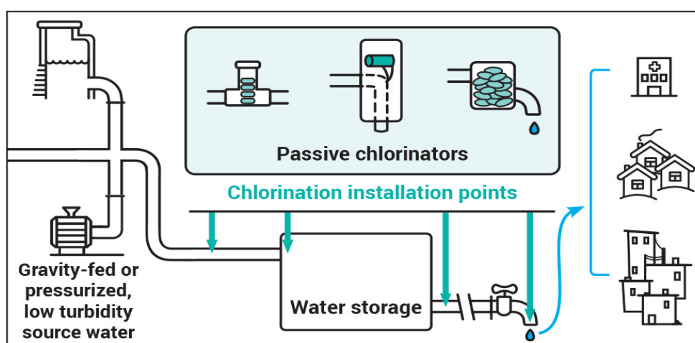
Figure 12. Passive chlorination at the point of consumption (63).
