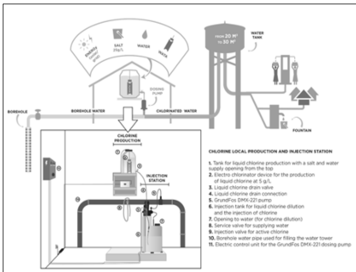
Figure 29. Chlorine production coupled into the dosing pump tank.
