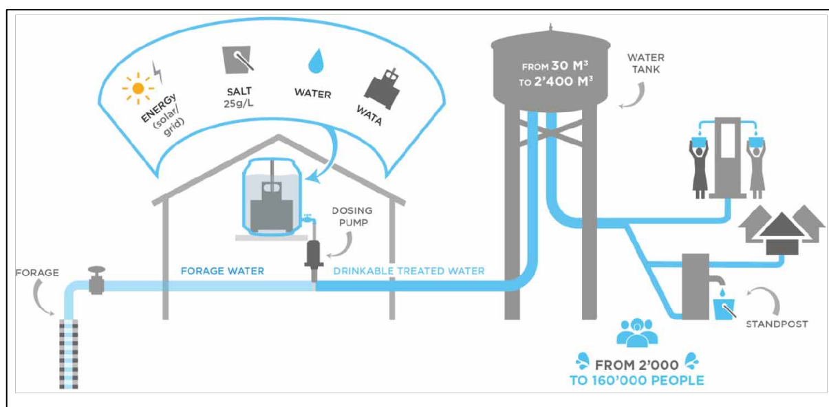
Figure 24. Adaptation of electro-chlorinators coupled to community water tanks.
