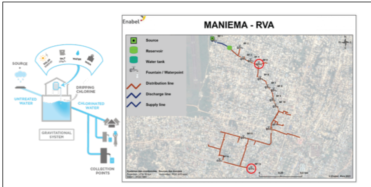
Figure 34. Water network and fountains selected. RVA in Kindu city, DRC.
