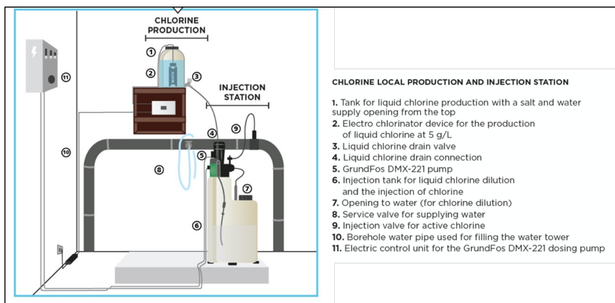
Figure 25. Chlorine production and injection station.
