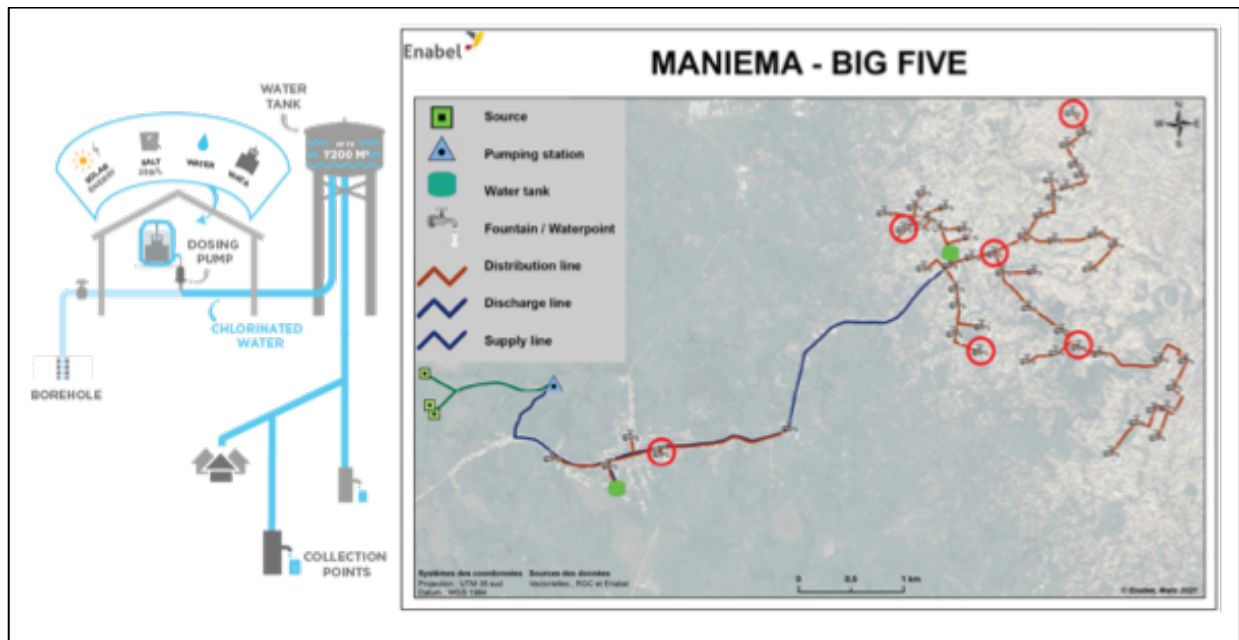
Figure 33. Water network station and fountains selected. Big Five, Kindu City, DRC.
