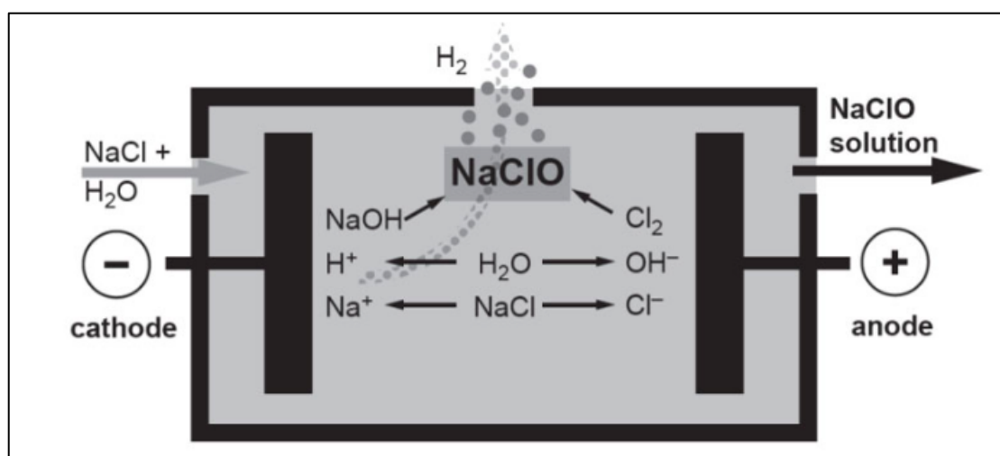
Figure 13. Representation of electrolysis (59).
