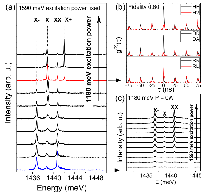
FIG. 5. (a) The set of spectra taken from a representative QD with variable dual wavelength excitation conditions. The above-bandgap excitation (1590 meV) was constant and only the 1180 meV excitation was increased. The increasing power of 1180 meV excitation is shown as a QD charge tuning mechanism. (b) Polarization-resolved second-order correlation curves measured from a QD with nearly neutral charge configuration. Polarization-entanglement is attested by the measured fidelity value of 0.600 \pm 0.025 . (c) A single wavelength excitation power dependent spectra showing that the negative charge configuration is dominant at all conditions and no correlations between X and XX can be efficiently measured.
