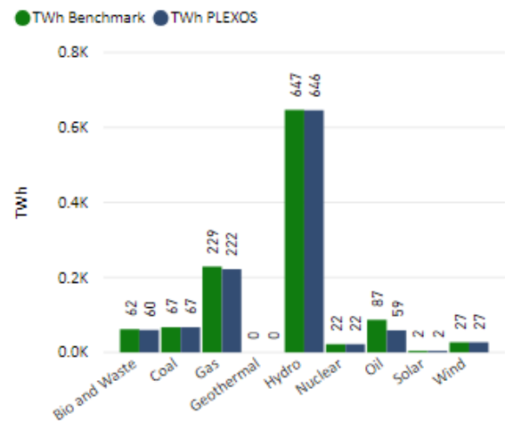
Figure C-7 Comparison of generation values per fuel type from the calibrated PLEXOS-World simulations with historically reported data for 2015.
