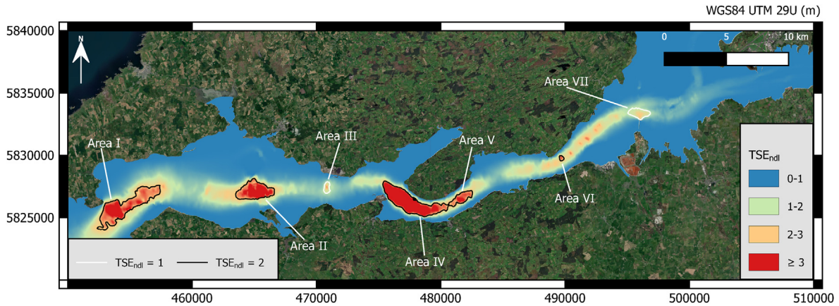
Fig. 9. Delimitation of the areas of interest for hydrokinetic energy exploitation based on the TSE_{ndl} . The lines corresponding to TSE_{ndl} values of 2 and 1 delimit the areas exceeding these thresholds.
