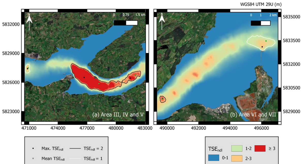
Fig. 10. Detailed view of the selected areas, identifying the representative points (maximum TSE_{ndl} and mean TSE_{ndl} ) selected for high-resolution analysis.
