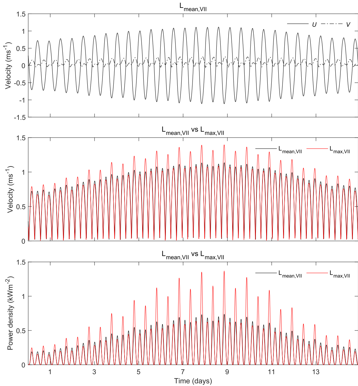
Fig. 14. High-resolution analysis in Area VII showing the time distribution of the current velocity components, U and V , at L_{\text{mean},\text{VII}} (above), the magnitude of current velocity at L_{\text{mean},\text{VII}} and L_{\text{max},\text{VII}} (intermediate), and the power density at L_{\text{mean},\text{VII}} and L_{\text{max},\text{VII}} (bottom).
