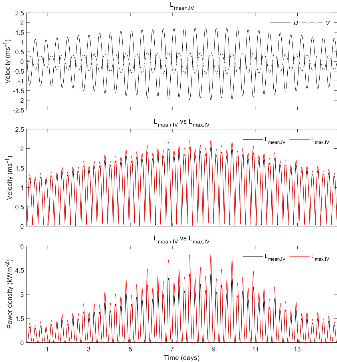
Fig. 12. High-resolution analysis in Area IV showing the time distribution of the current velocity components, U and V , at L_{\text{mean,IV}} (above), the magnitude of current velocity at L_{\text{mean,IV}} and L_{\text{max,IV}} (intermediate), and the power density at L_{\text{mean,IV}} and L_{\text{max,IV}} (bottom).
