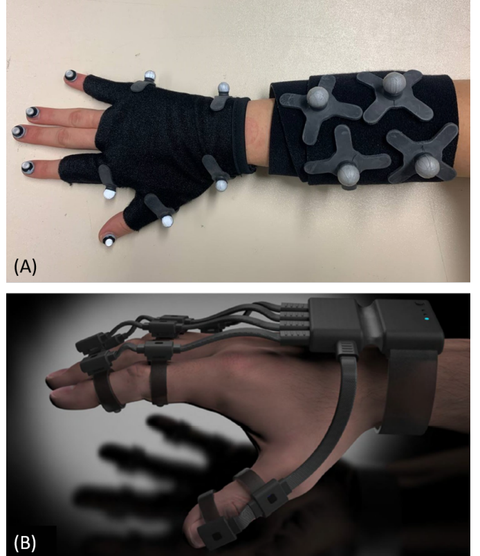
Fig. 1. (A) Hand with the 10 reflective markers and 4 markers for the forearm. (B) Tyndall Smart Glove (Tyndall National Institute, CO, IE).
