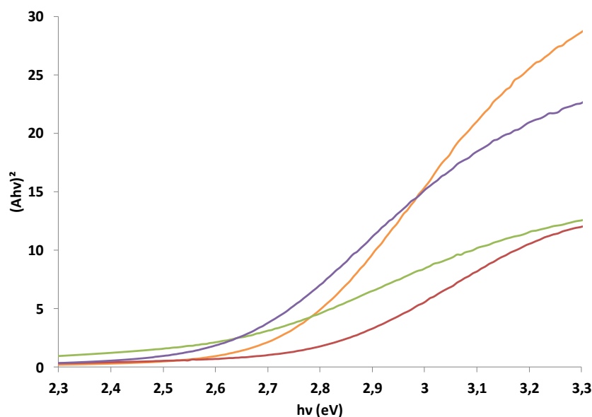
Fig S7: plot of (Ah\nu)^2=f(h\nu) for mono-aminated bdc-NH 2 -based samples: 10%-MIL-125-NH 2 (red), 20%-MIL-125-NH 2 (green) 50%-MIL-125-NH 2 (purple) MIL-125-NH 2 and 100%-MIL-125-NH 2 (orange).
