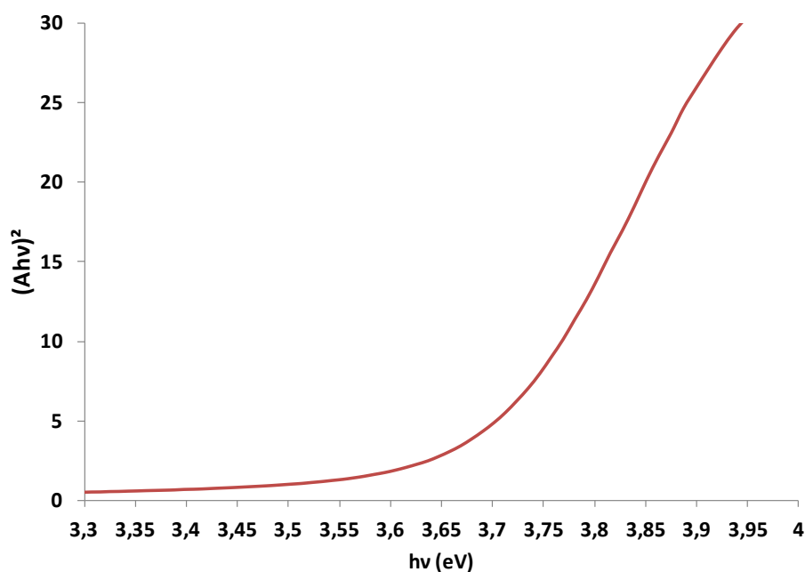
Fig S6: plot of (Ah\nu)^2=f(h\nu) for MIL-125
