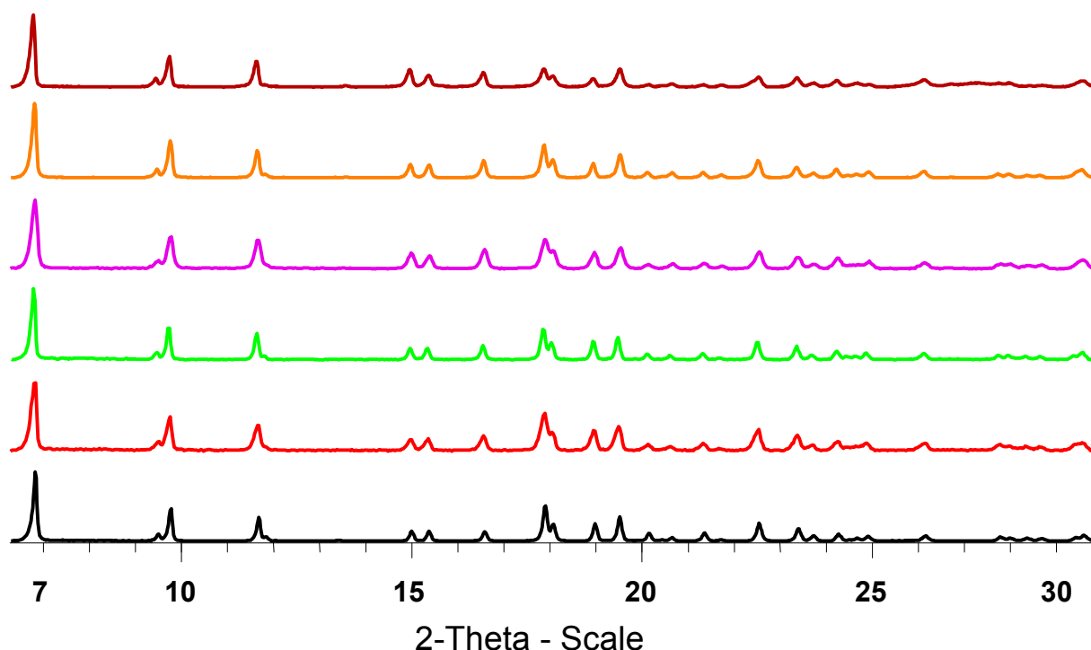
Fig S1: XRD patterns of MIL-125 (black), and mono-aminated bdc-NH 2 -based samples: 10%-MIL-125-NH 2 (red), 20%-MIL-125-NH 2 (green), 50%-MIL-125-NH 2 (purple), MIL-125-NH 2 or 100%-MIL-125-NH 2 (orange) and the 10%/90% di/mono-aminated MIL-125 (brown).
